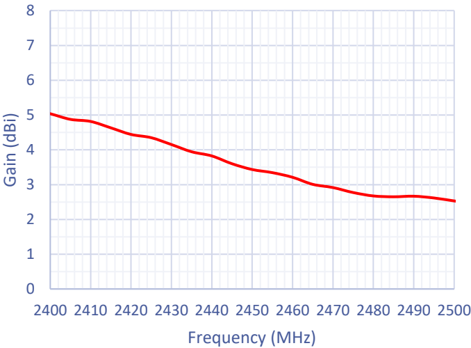
Realized Antenna Gain
