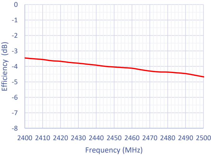
Total Antenna Efficiency
