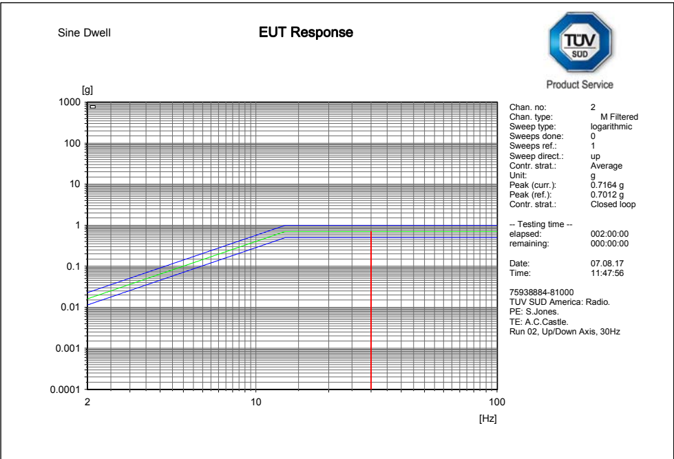
Figure 12 – Endurance Run (EUT) – Up and Down
