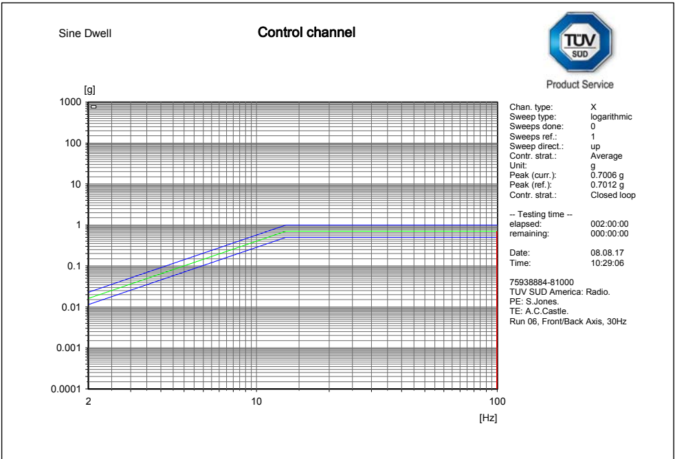
Figure 3 – Endurance Run (Control) - Fore-Aft
