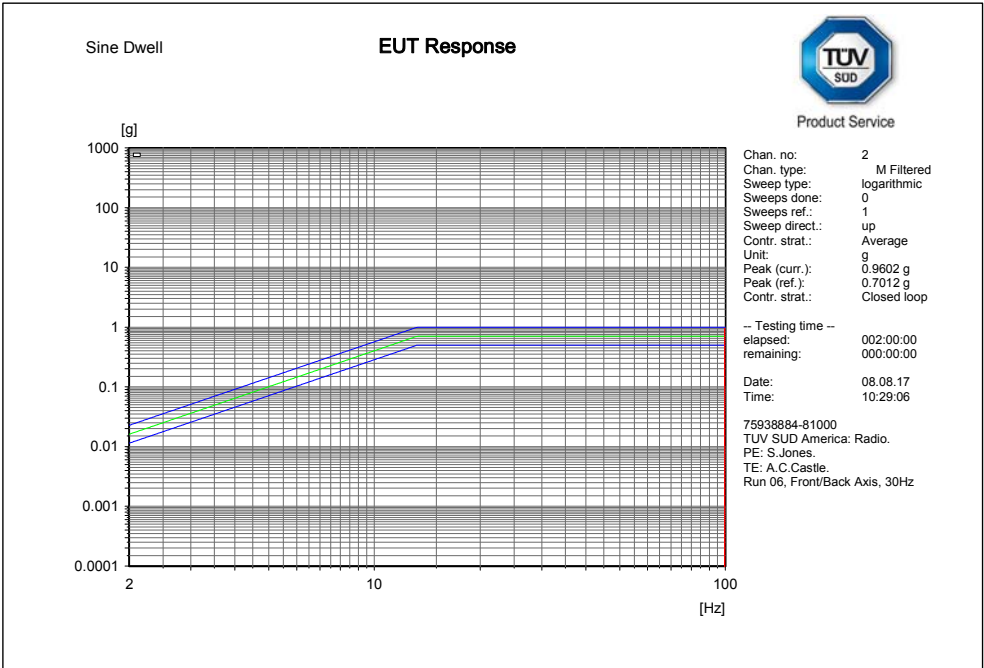
Figure 4 – Endurance Run (EUT) - Fore-Aft
