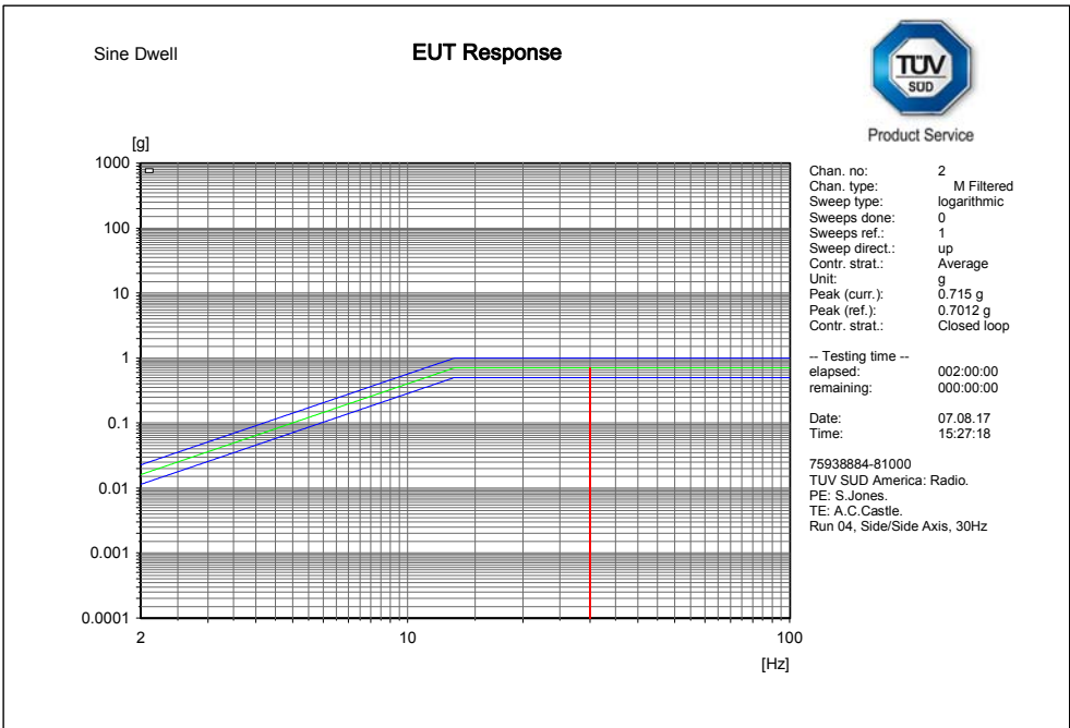
Figure 8 – Endurance Run (EUT) – Side to Side
