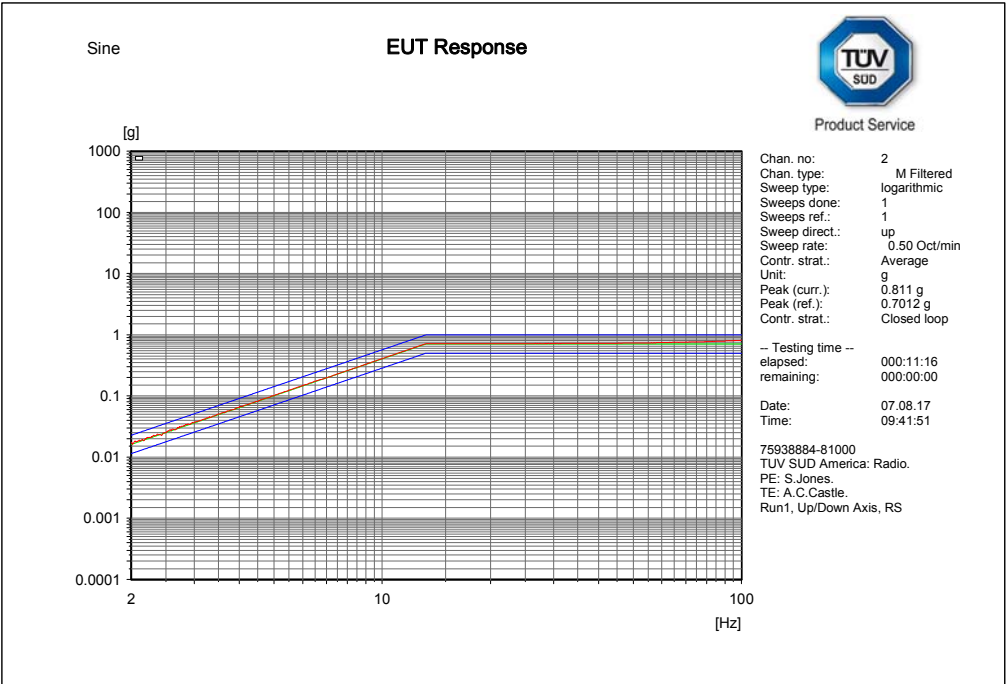
Figure 10 - Resonance Search (EUT) – Up and Down
