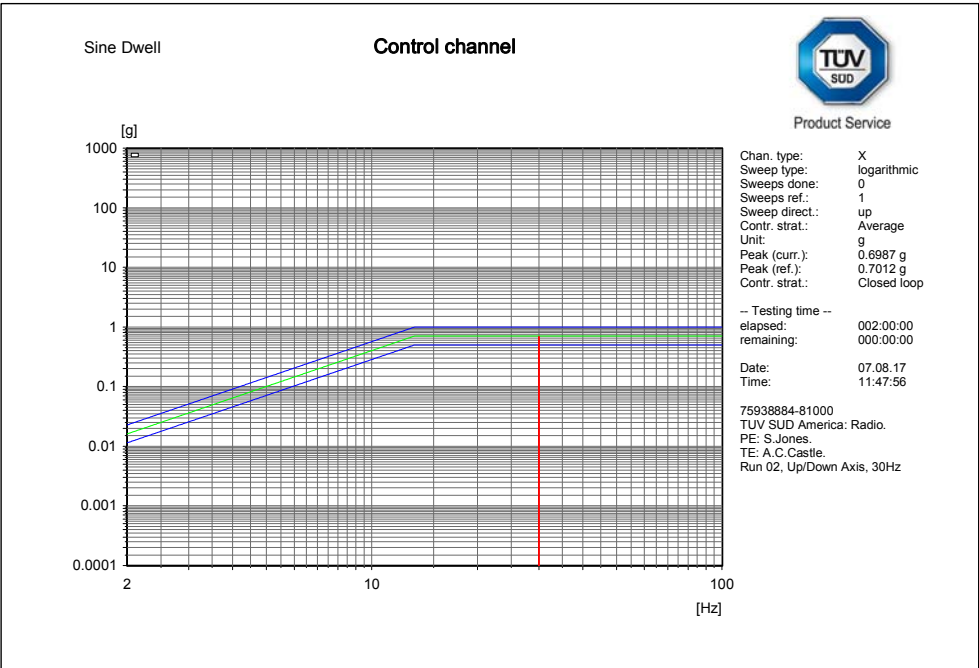
Figure 11 – Endurance Run (Control) – Up and Down
