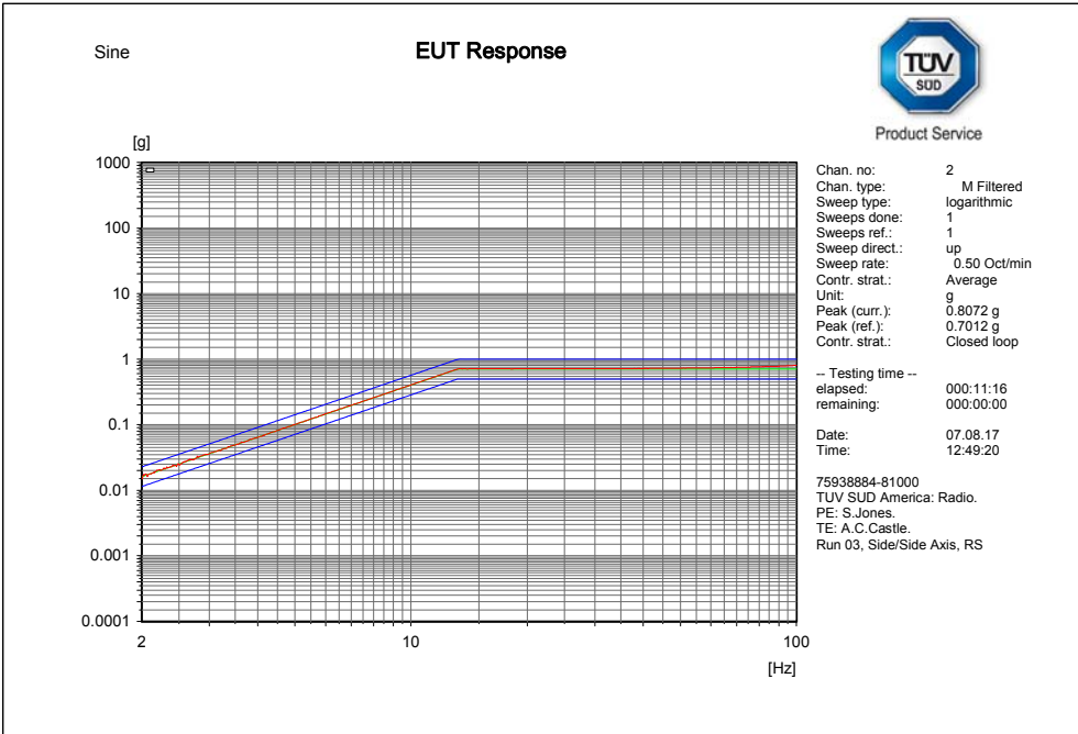
Figure 6 - Resonance Search (EUT) – Side to Side
