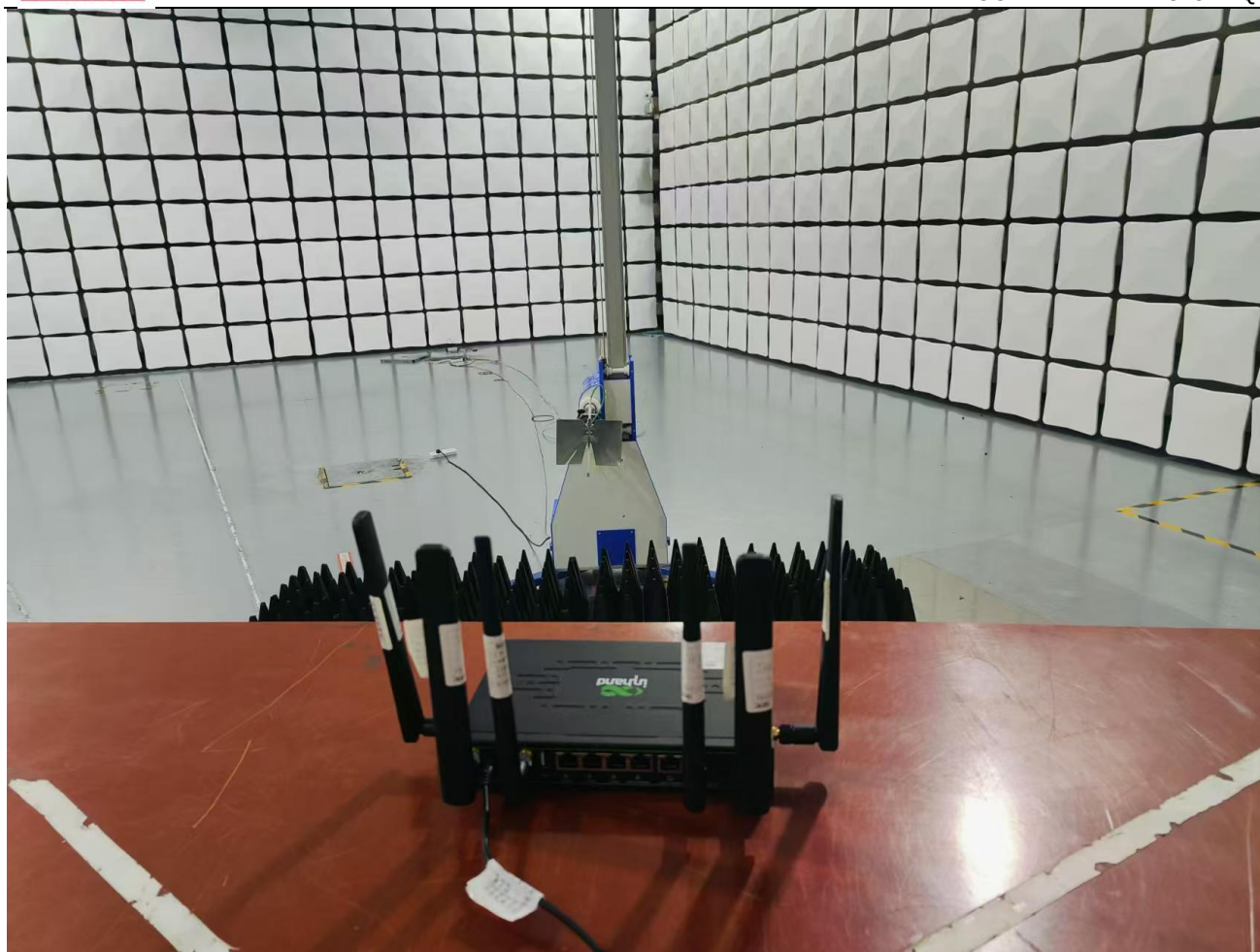
RF Radiated Test setup (>1GHz)
