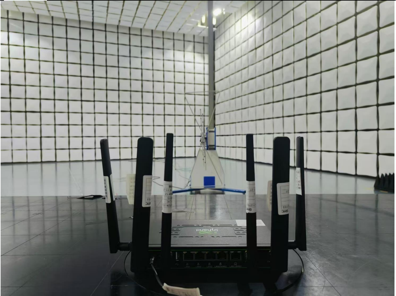
RF Radiated Test setup (30MHz~1GHz)
