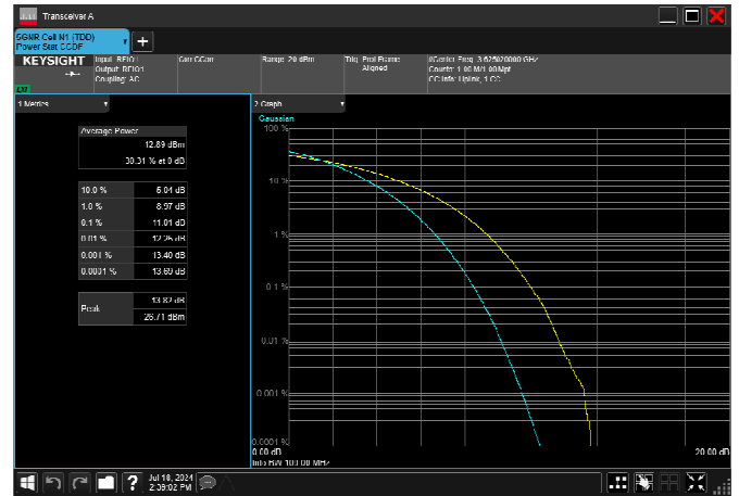
n77_2_100MHz_30kHz_3625MHz_CP-OFDM 64 QAM_RB273@0 11.01dB
