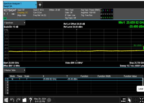
B2_N7(50M)_DFT-s- OFDM_QPSK_Edge_1RB_Left_Mid_CH
