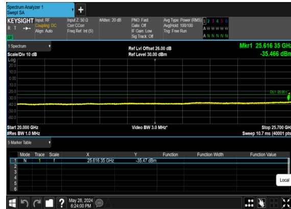
B2_N7(5M)_DFT-s- OFDM_QPSK_Edge_1RB_Left_Mid_CH
