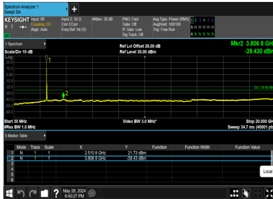
B2_N7(50M)_DFT-s- OFDM_QPSK_Edge_1RB_Left_Mid_CH
