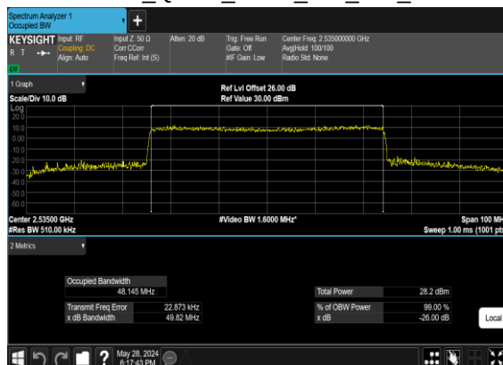
B2_N7(50M)_CP- OFDM_QPSK_Outer_Full_Mid_CH
