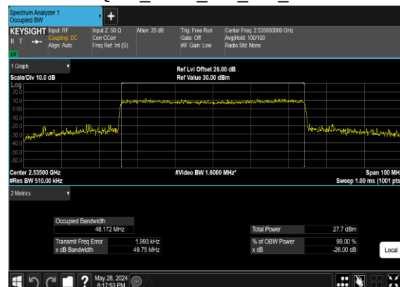
B2_N7(50M)_CP-OFDM_16 QAM_Outer_Full_Mid_CH
