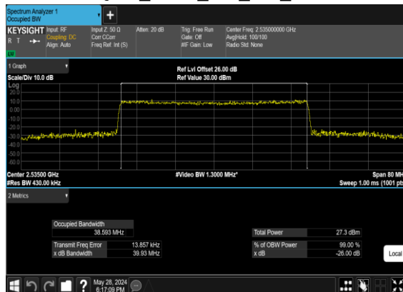
B2_N7(40M)_CP-OFDM_64 QAM_Outer_Full_Mid_CH
