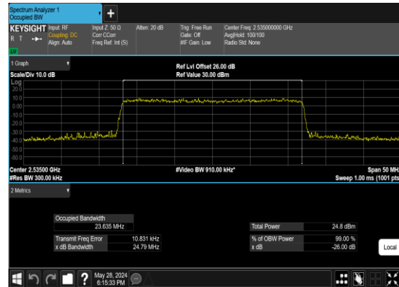
B2_N7(25M)_CP-OFDM_256 QAM_Outer_Full_Mid_CH
