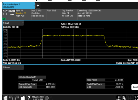
B2_N7(10M)_CP-OFDM_16 QAM_Outer_Full_Mid_CH
