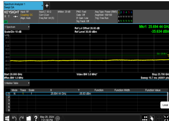
B2_N7(50M)_DFT-s- OFDM_QPSK_Edge_1RB_Left_High_CH
