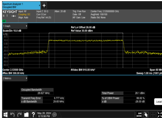
B2_N7(30M)_CP- OFDM_QPSK_Outer_Full_Mid_CH
