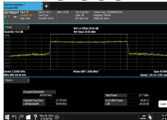
B2_N7(40M)_CP-OFDM_16 QAM_Outer_Full_Mid_CH
