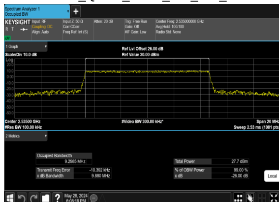
B2_N7(10M)_CP- OFDM_QPSK_Outer_Full_Mid_CH
