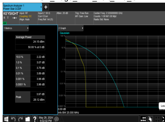
B2_N7(20M)_DFT-s-OFDM_PI_2-BPSK_Edge_1RB_Left_Mid_CH
