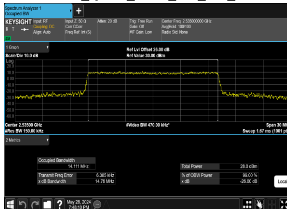
B2_N7(15M)_CP- OFDM_QPSK_Outer_Full_Mid_CH
