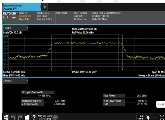
B2_N7(5M)_CP-OFDM_64 QAM_Outer_Full_Mid_CH
