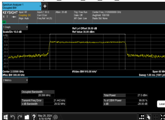
B2_N7(30M)_CP-OFDM_64 QAM_Outer_Full_Mid_CH
