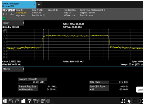
B2_N7(25M)_CP-OFDM_64 QAM_Outer_Full_Mid_CH
