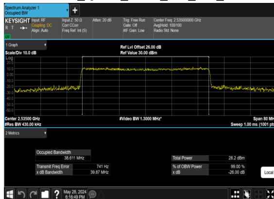
B2_N7(40M)_CP- OFDM_QPSK_Outer_Full_Mid_CH
