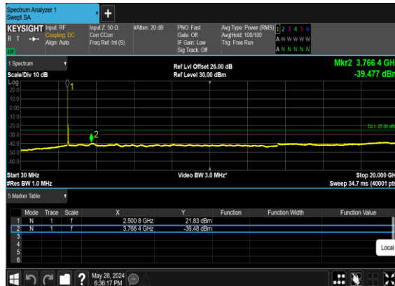
B2_N7(50M)_DFT-s- OFDM_BPSK_Edge_1RB_Left_Low_CH
