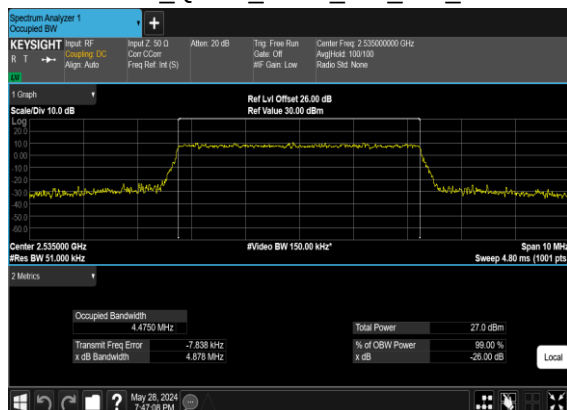
B2_N7(5M)_CP- OFDM_QPSK_Outer_Full_Mid_CH
