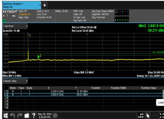
B2_N7(50M)_DFT-s- OFDM_BPSK_Edge_1RB_Left_High_CH
