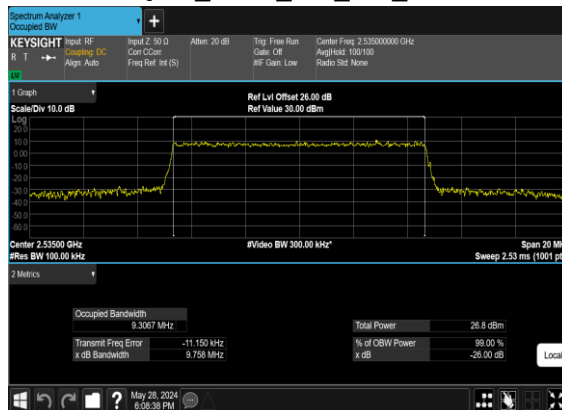
B2_N7(10M)_CP-OFDM_64 QAM_Outer_Full_Mid_CH
