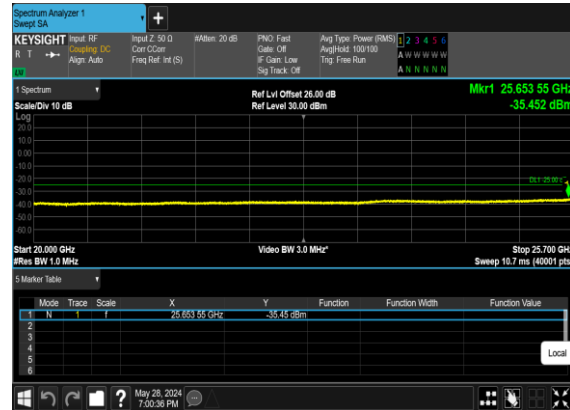
B2_N7(50M)_DFT-s- OFDM_BPSK_Edge_1RB_Left_High_CH
