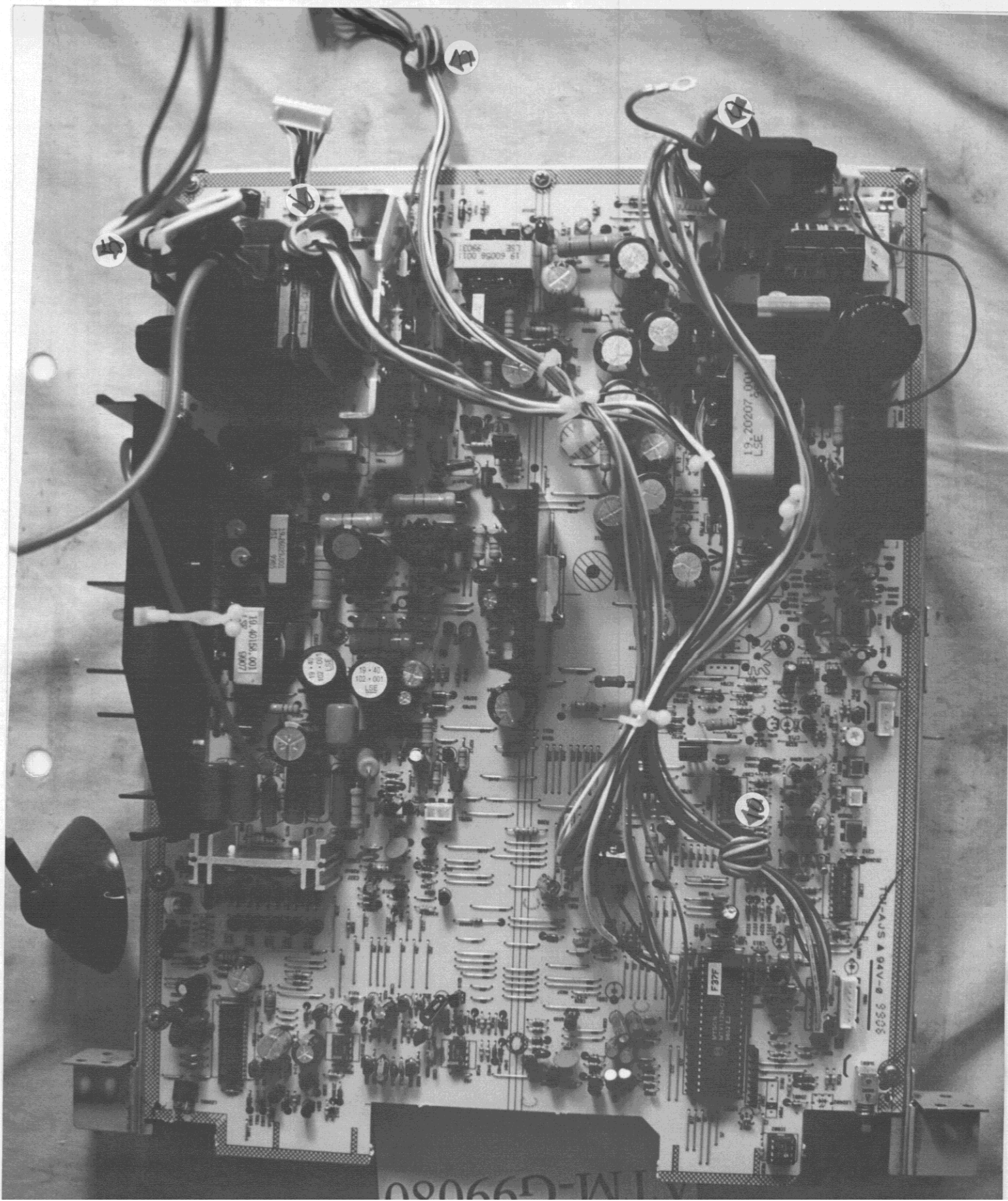
Figure 14 Mother Board (Component Side)
