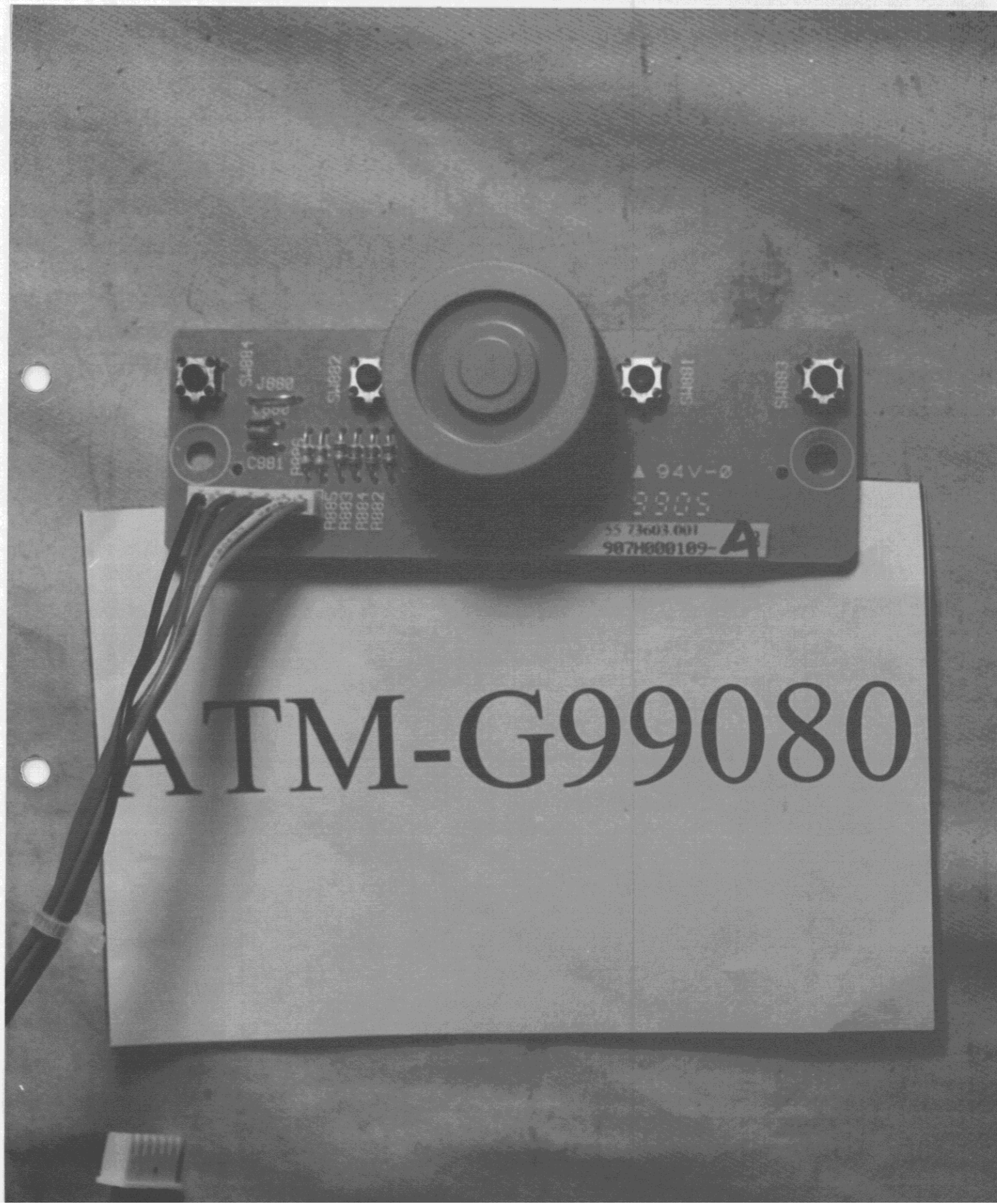
Figure 18 OSD Button Control Board (Component Side)
