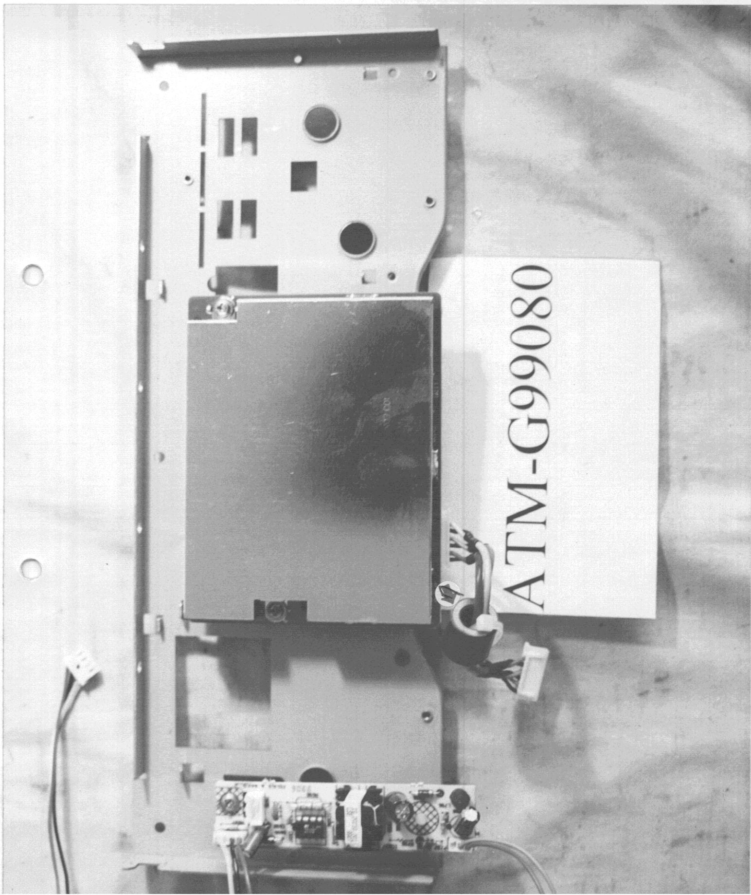
Figure 10 I/O Control Board & Inverter Board with Bracket
