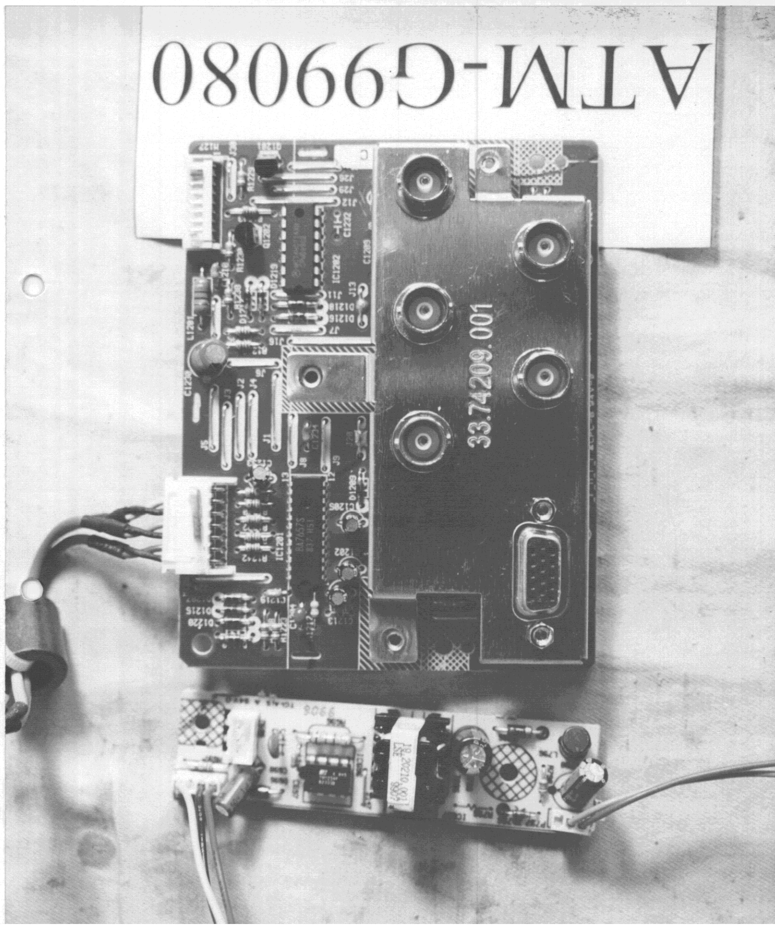
Figure 11 I/O Control Board & Inverter Board (Component Side)
