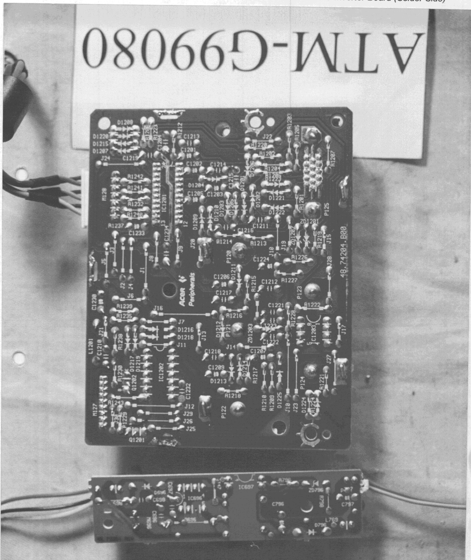
Figure 13 I/O Control Board & Inverter Board (Solder Side)
