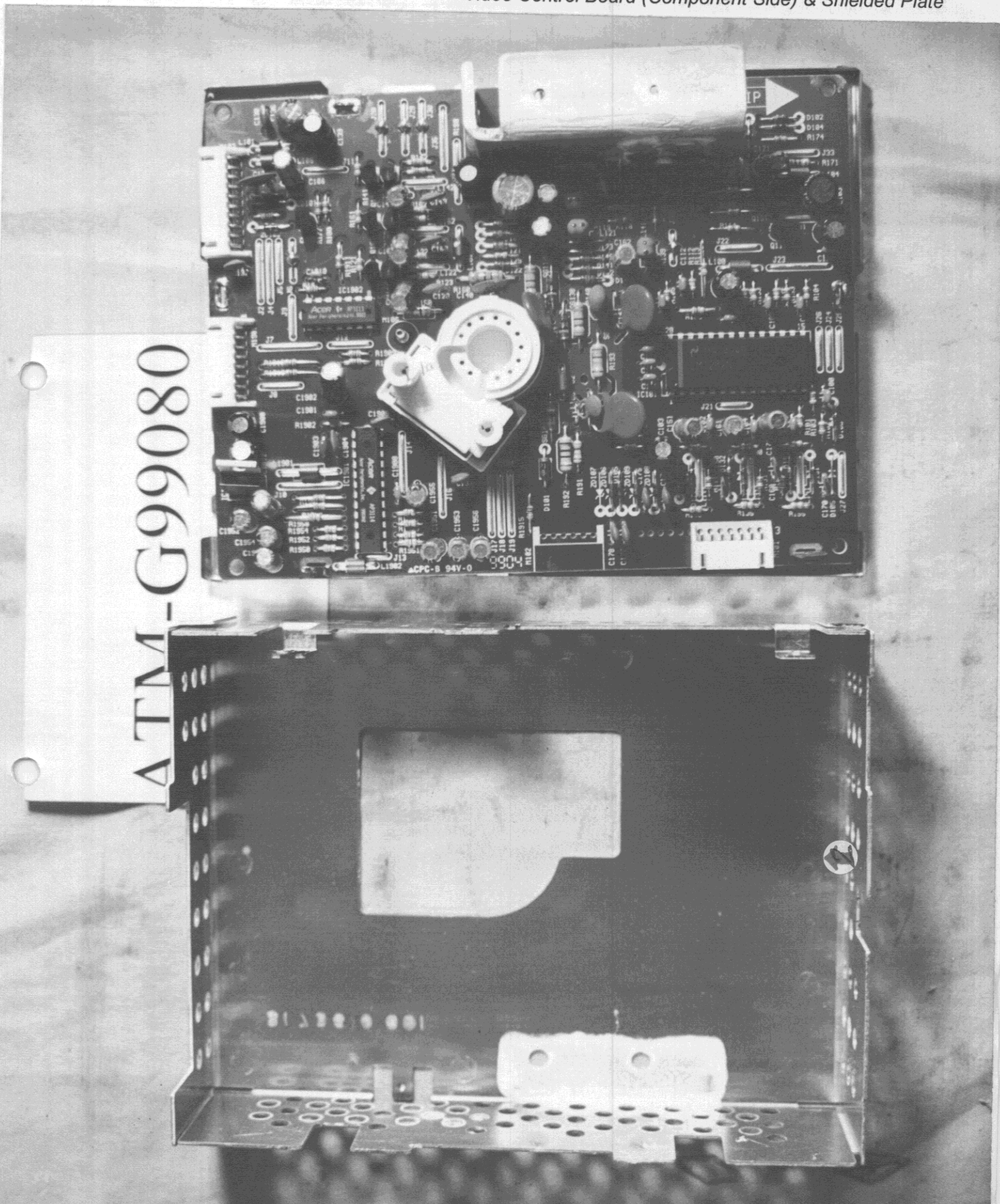
Figure 16 Video Control Board (Component Side) & Shielded Plate
