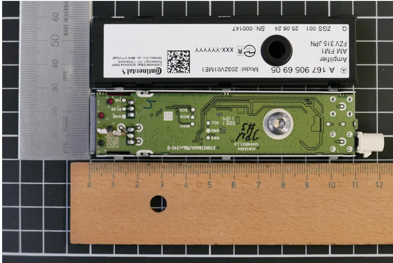
Module opened PCBA BOTTOM
