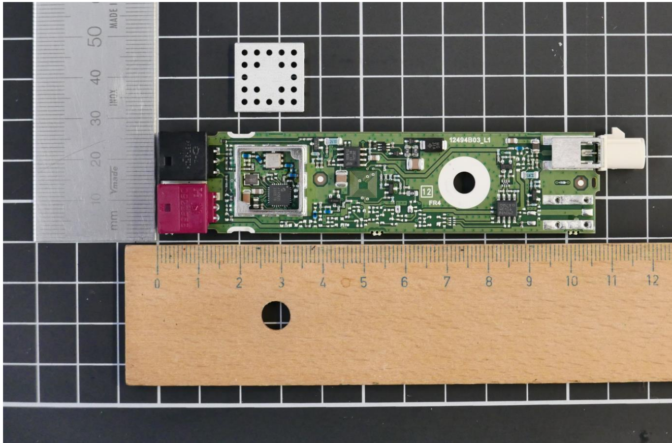
PCBA TOP / shielding opened
