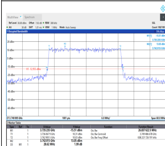
1-N78-3700-3800--30-30-M-1-DFT-QPSK-Outer_Full-75@0-Ant1-26.838-28.620-≤30-PAS S
