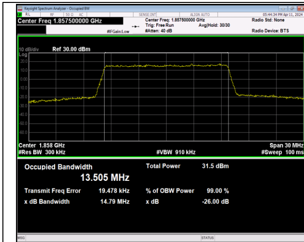
Band2-15MHz-QPSK-18675-75RB#0-PASS
