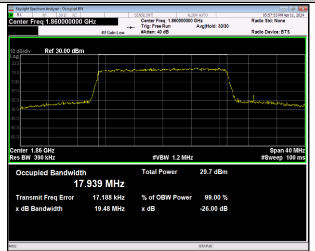
Band2-20MHz-64QAM-18700-100RB#0-PASS
