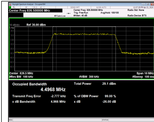
Band5-5MHz-64QAM-20425-25RB#0-PASS
