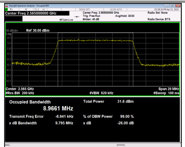
Band7-10MHz-QPSK-21400-50RB#0-PASS
