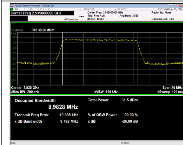
Band7-10MHz-QPSK-21100-50RB#0-PASS
