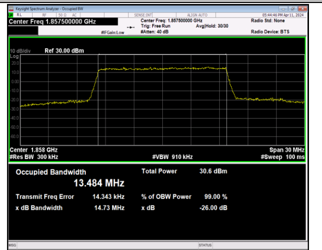
Band2-15MHz-16QAM-18675-75RB#0-PASS
