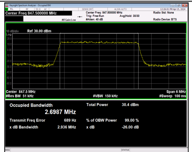
Band5-3MHz-QPSK-20635-15RB#0-PASS
