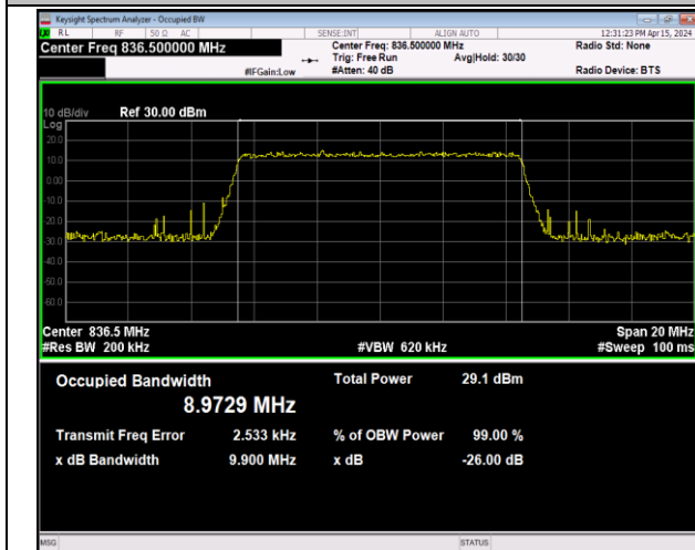
Band5-10MHz-64QAM-20525-50RB#0-PASS
