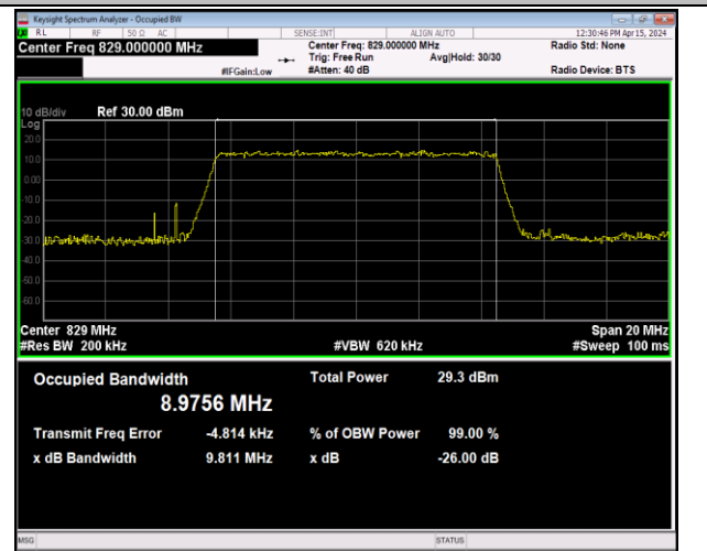
Band5-10MHz-64QAM-20450-50RB#0-PASS
