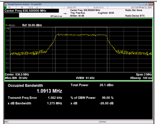
Band5-1.4MHz-64QAM-20525-6RB#0-PASS
