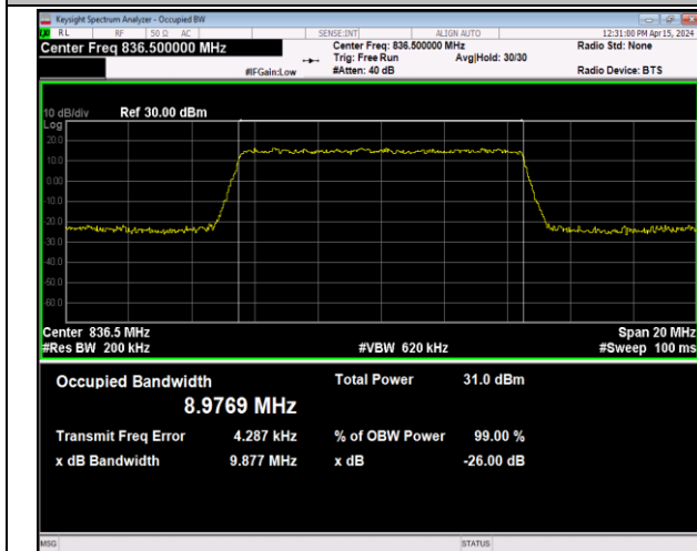
Band5-10MHz-QPSK-20525-50RB#0-PASS
