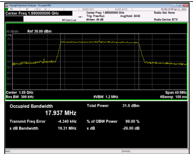
Band2-20MHz-16QAM-18900-100RB#0-PASS
