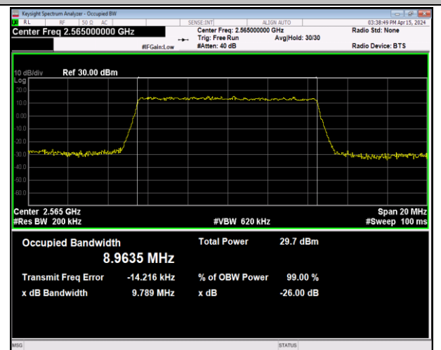
Band7-10MHz-64QAM-21400-50RB#0-PASS
