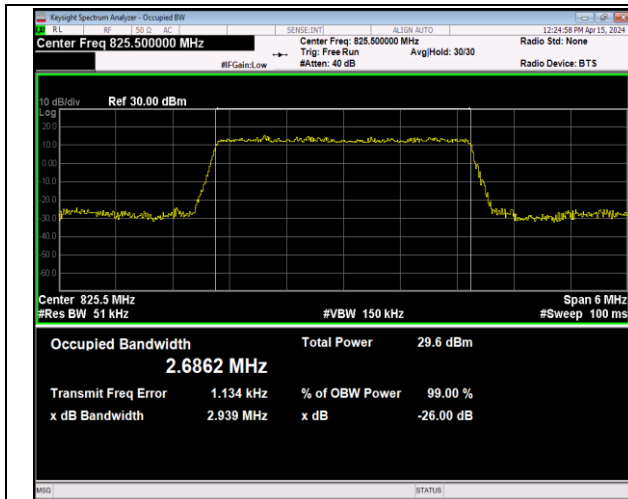
Band5-3MHz-16QAM-20415-15RB#0-PASS
