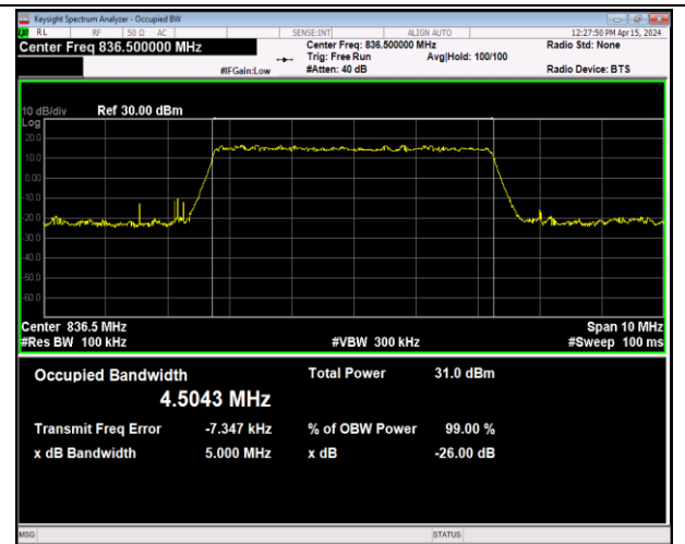
Band5-5MHz-QPSK-20525-25RB#0-PASS
