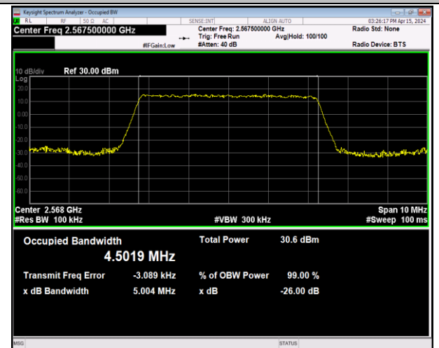
Band7-5MHz-16QAM-21425-25RB#0-PASS
