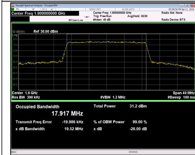
Band2-20MHz-16QAM-19100-100RB#0-PASS
