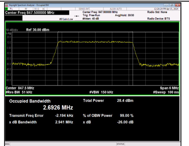
Band5-3MHz-64QAM-20635-15RB#0-PASS
