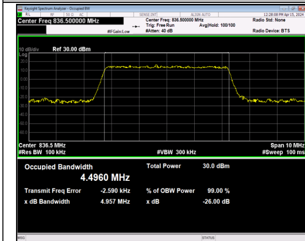
Band5-5MHz-16QAM-20525-25RB#0-PASS
