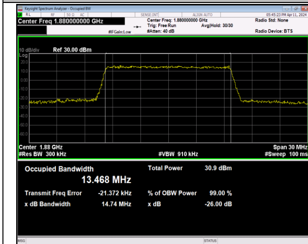
Band2-15MHz-16QAM-18900-75RB#0-PASS
