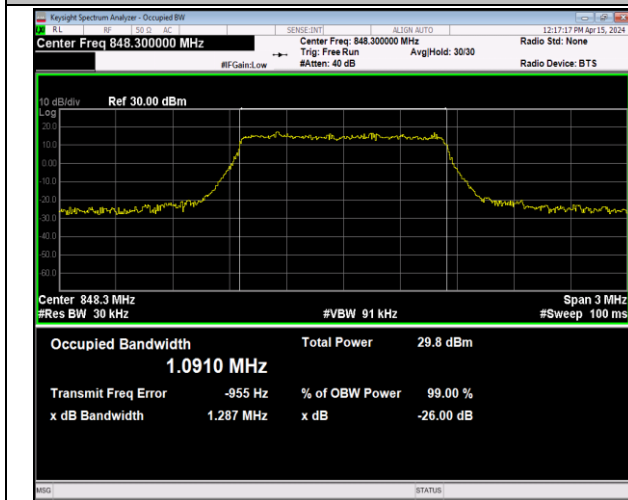
Band5-1.4MHz-QPSK-20643-6RB#0-PASS
