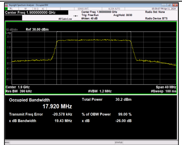
Band2-20MHz-64QAM-19100-100RB#0-PASS
