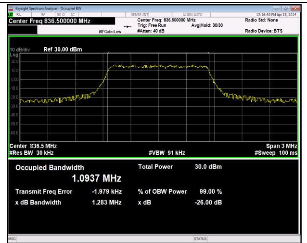
Band5-1.4MHz-QPSK-20525-6RB#0-PASS
