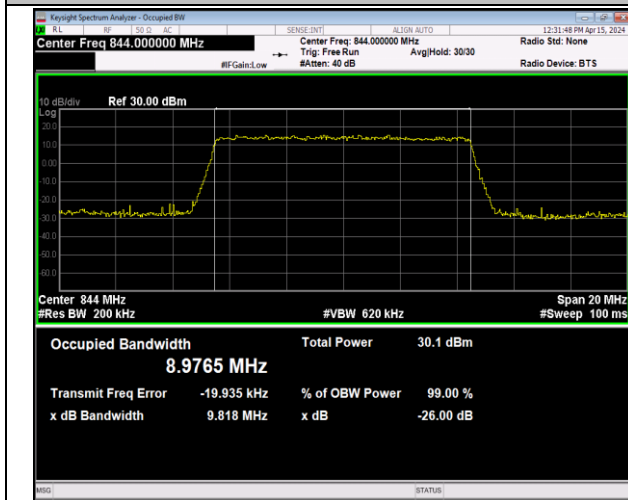
Band5-10MHz-16QAM-20600-50RB#0-PASS
