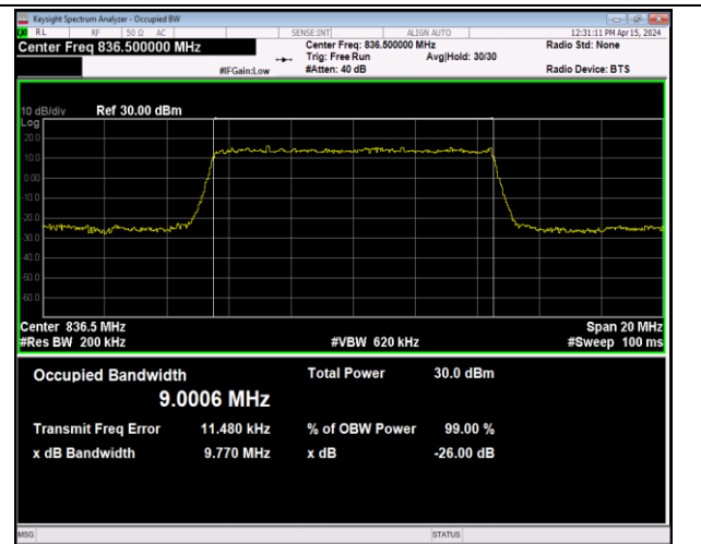
Band5-10MHz-16QAM-20525-50RB#0-PASS
