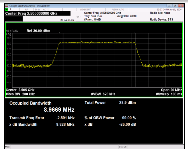
Band7-10MHz-64QAM-20800-50RB#0-PASS
