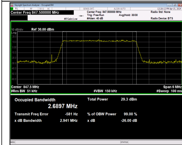
Band5-3MHz-16QAM-20635-15RB#0-PASS
