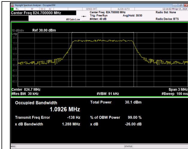
Band5-1.4MHz-QPSK-20407-6RB#0-PASS
