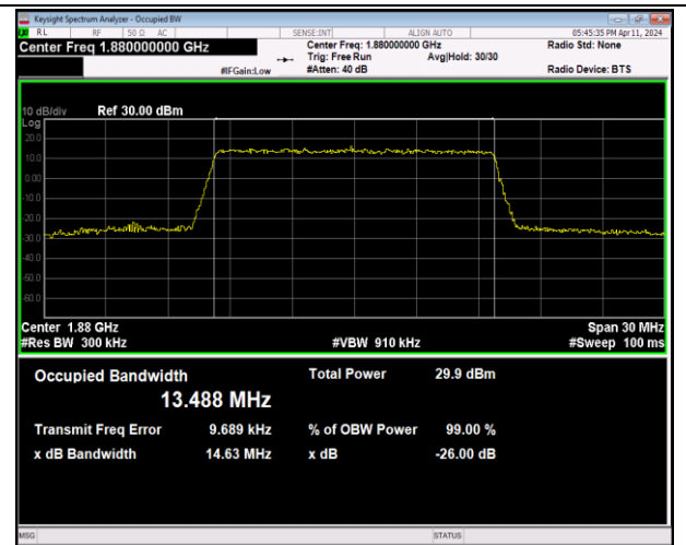
Band2-15MHz-64QAM-18900-75RB#0-PASS
