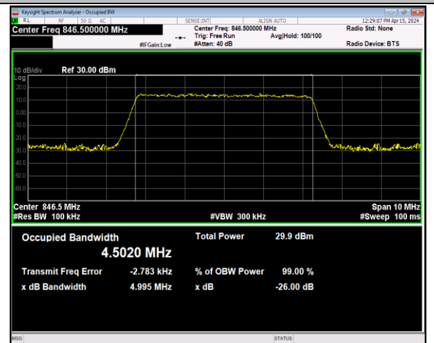
Band5-5MHz-16QAM-20625-25RB#0-PASS
