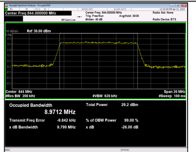
Band5-10MHz-64QAM-20600-50RB#0-PASS
