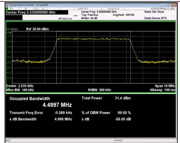
Band7-5MHz-QPSK-21100-25RB#0-PASS
