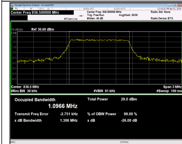
Band5-1.4MHz-16QAM-20525-6RB#0-PASS
