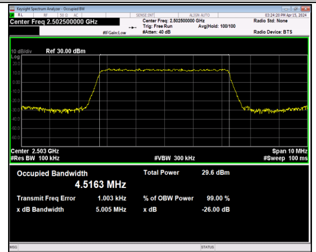
Band7-5MHz-16QAM-20775-25RB#0-PASS
