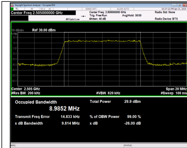
Band7-10MHz-16QAM-20800-50RB#0-PASS
