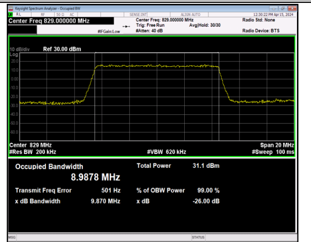
Band5-10MHz-QPSK-20450-50RB#0-PASS
