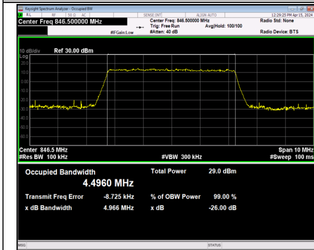
Band5-5MHz-64QAM-20625-25RB#0-PASS
