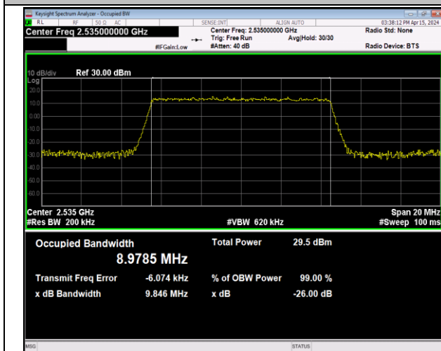
Band7-10MHz-64QAM-21100-50RB#0-PASS
