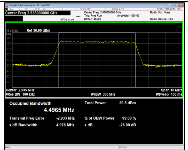
Band7-5MHz-64QAM-21100-25RB#0-PASS
