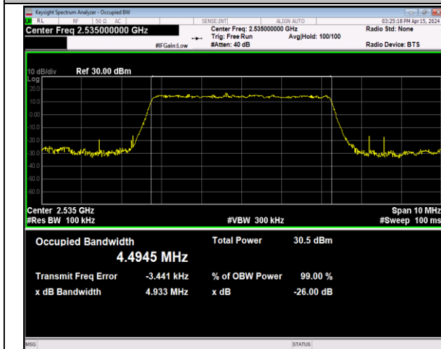
Band7-5MHz-16QAM-21100-25RB#0-PASS
