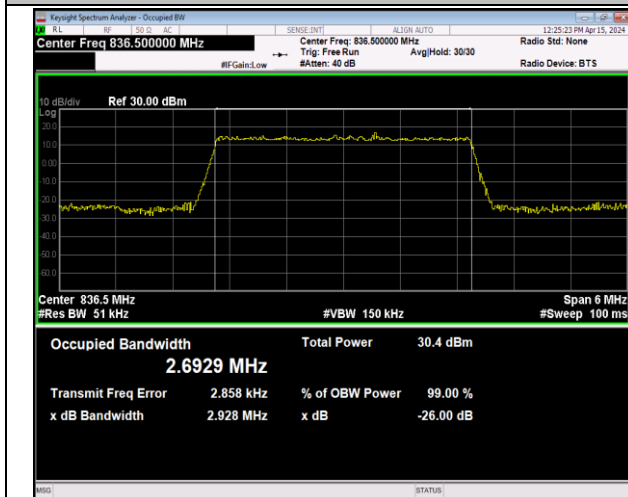
Band5-3MHz-QPSK-20525-15RB#0-PASS
