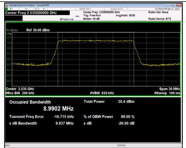
Band7-10MHz-16QAM-21100-50RB#0-PASS
