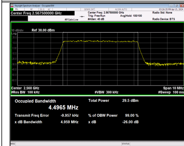
Band7-5MHz-64QAM-21425-25RB#0-PASS
