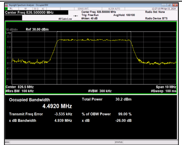
Band5-5MHz-16QAM-20425-25RB#0-PASS
