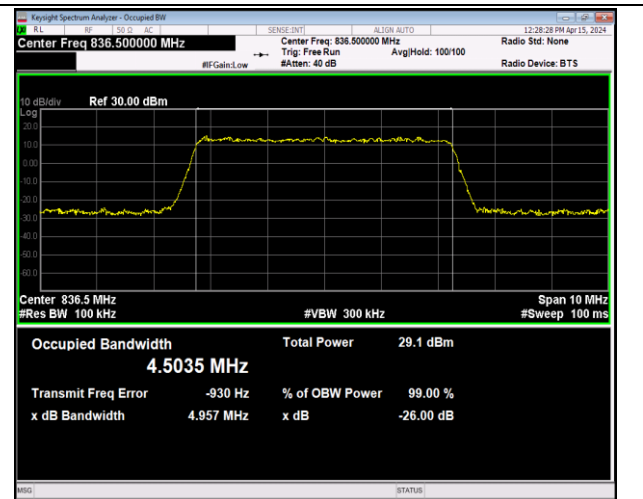
Band5-5MHz-64QAM-20525-25RB#0-PASS
