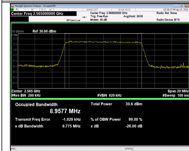
Band7-10MHz-16QAM-21400-50RB#0-PASS
