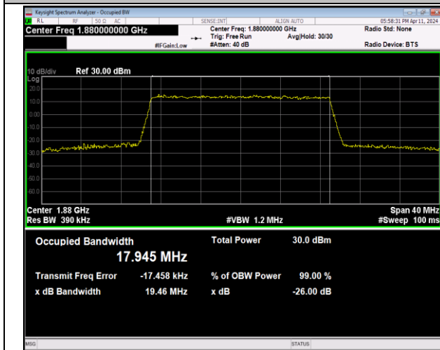
Band2-20MHz-64QAM-18900-100RB#0-PASS
