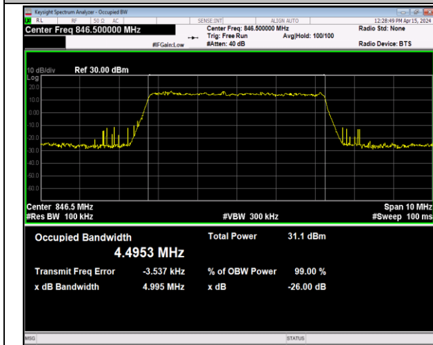
Band5-5MHz-QPSK-20625-25RB#0-PASS
