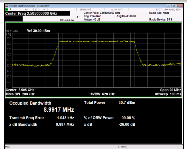
Band7-10MHz-QPSK-20800-50RB#0-PASS
