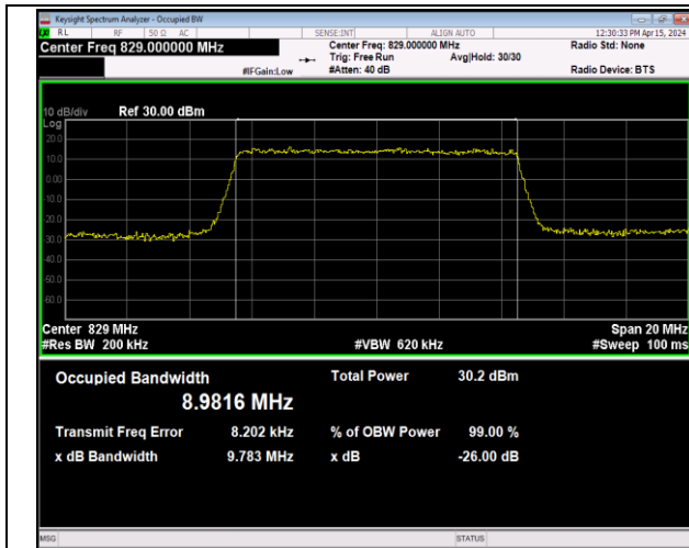
Band5-10MHz-16QAM-20450-50RB#0-PASS
