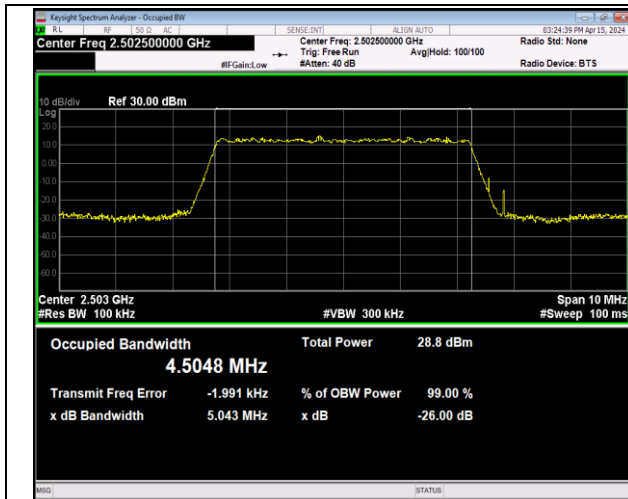
Band7-5MHz-64QAM-20775-25RB#0-PASS
