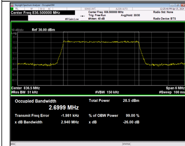
Band5-3MHz-64QAM-20525-15RB#0-PASS
