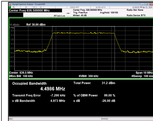
Band5-5MHz-QPSK-20425-25RB#0-PASS
