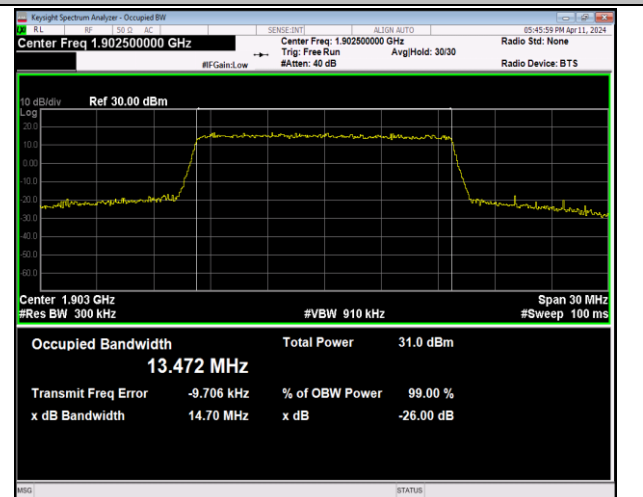
Band2-15MHz-16QAM-19125-75RB#0-PASS
