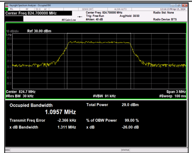
Band5-1.4MHz-16QAM-20407-6RB#0-PASS
