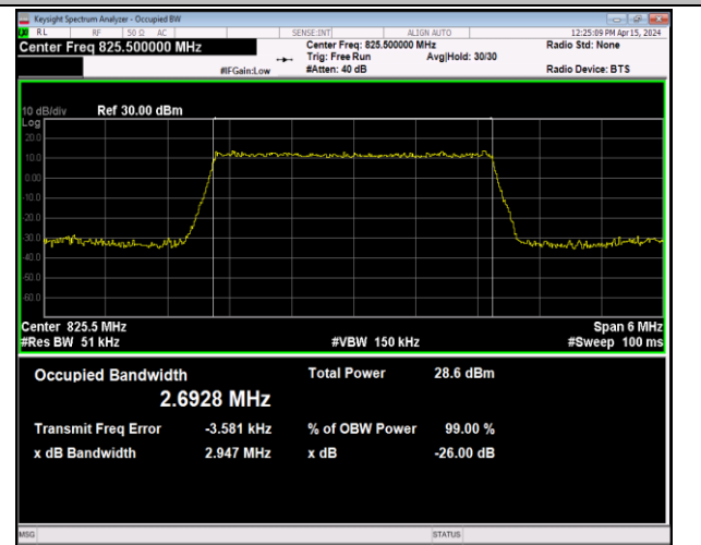
Band5-3MHz-64QAM-20415-15RB#0-PASS
