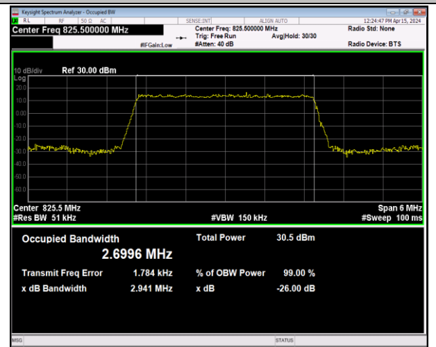
Band5-3MHz-QPSK-20415-15RB#0-PASS
