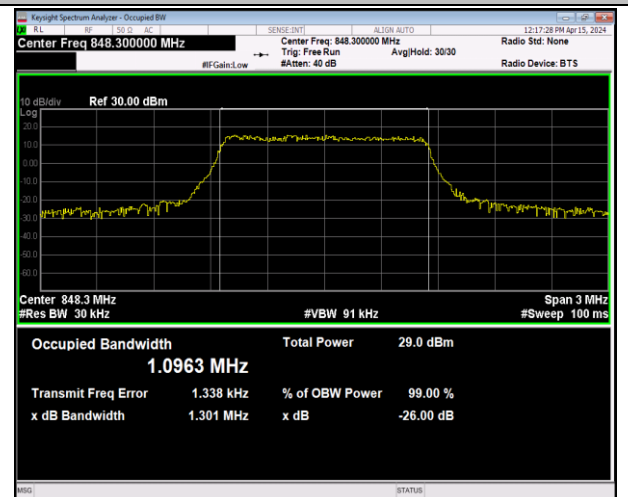
Band5-1.4MHz-16QAM-20643-6RB#0-PASS
