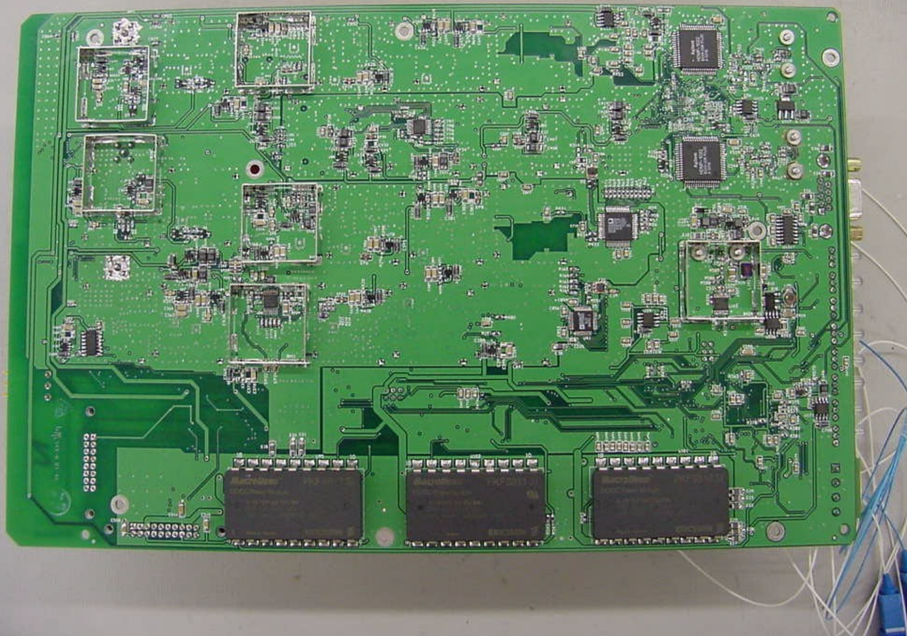
Digivance LRCS 800 MHz STM Control Board - Bottom View
