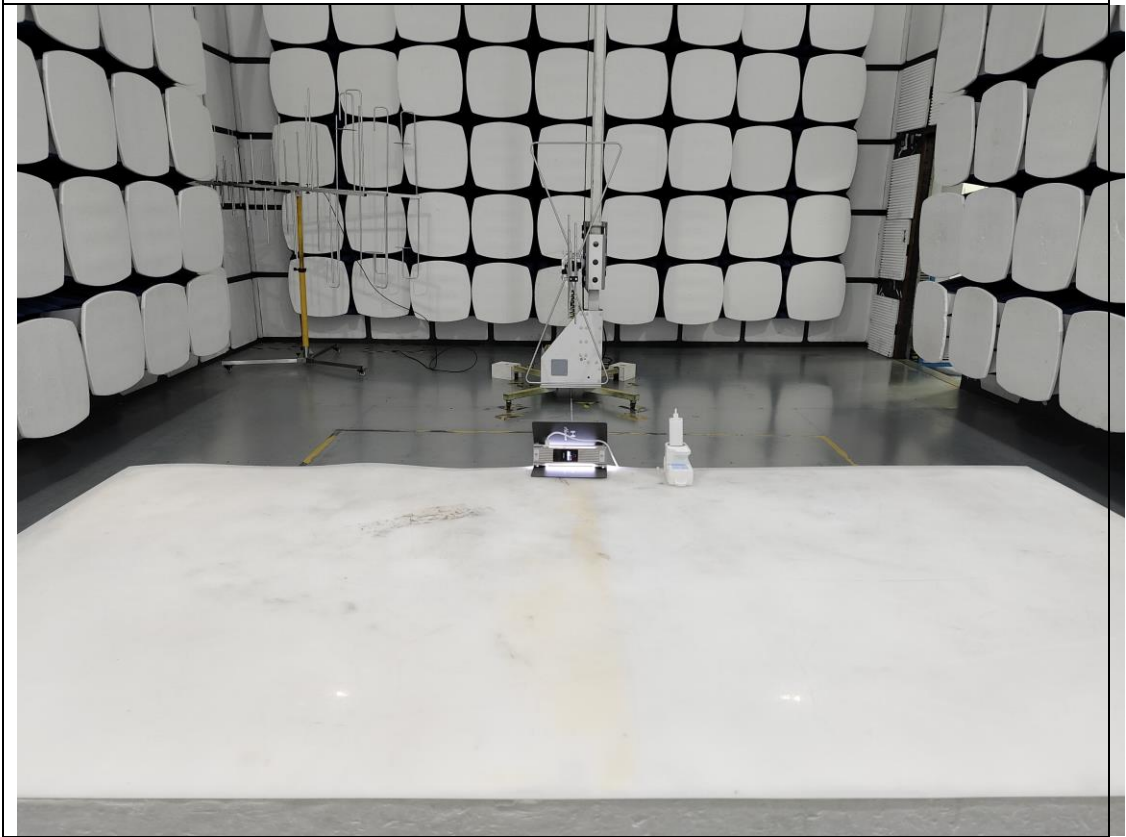
Radiated Emission
