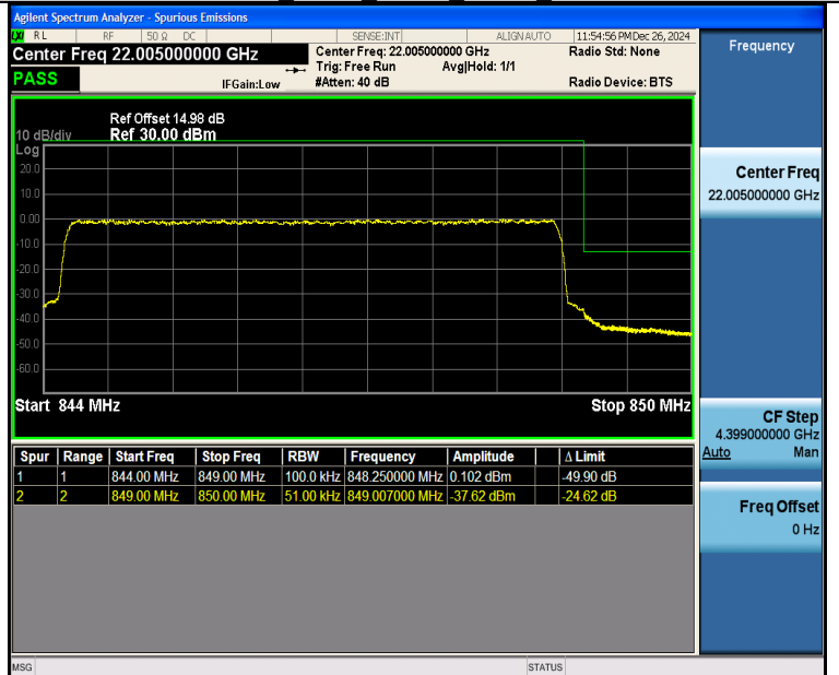
Band26 5MHz QPSK 27015 25RB#0
