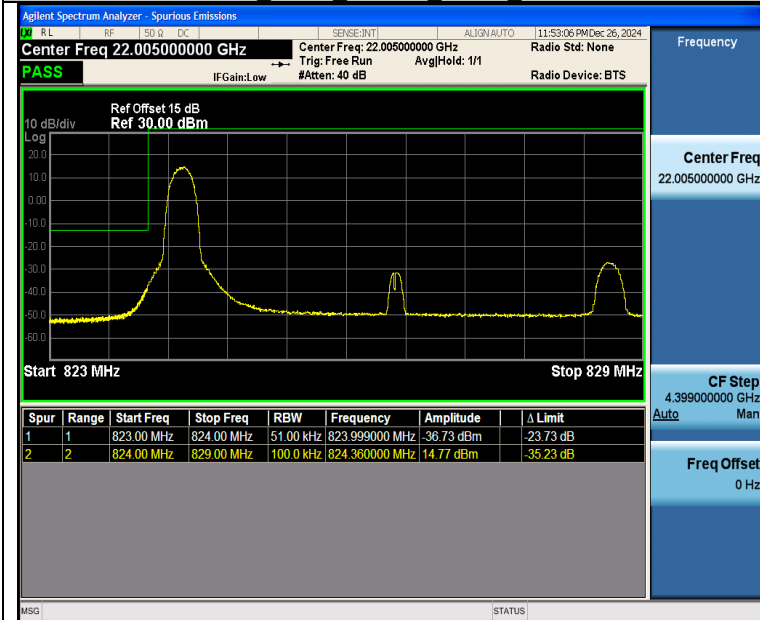
Band26 5MHz 16QAM 26815 1RB#0
