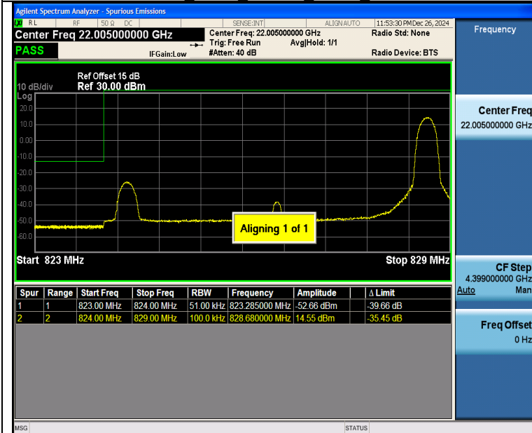
Band26 5MHz 16QAM 26815 1RB#24
