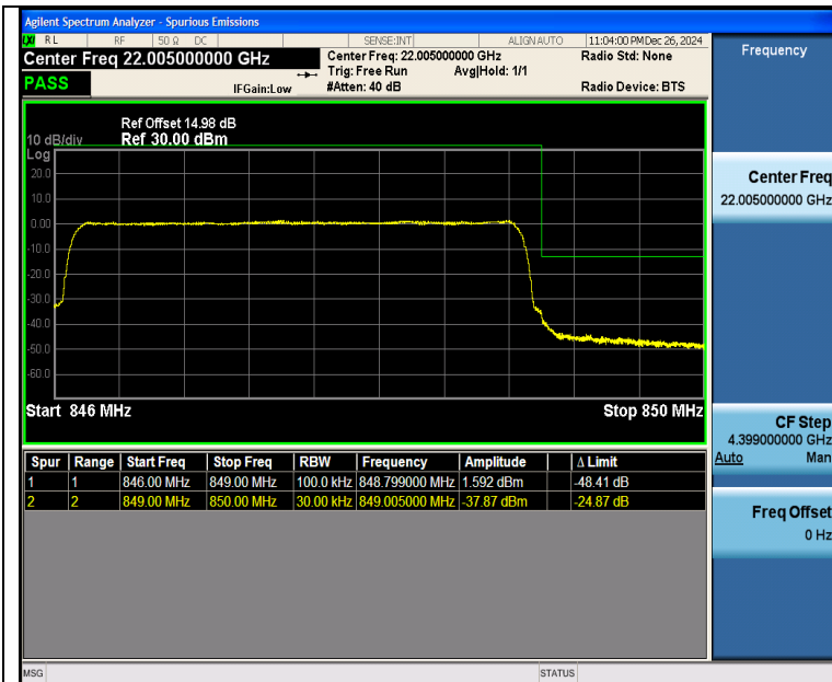
Band26 3MHz 16QAM 27025 15RB#0
