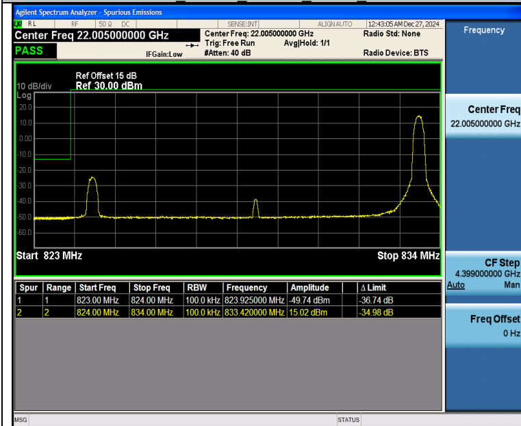
Band26_10MHz_16QAM_26840_1RB#49
