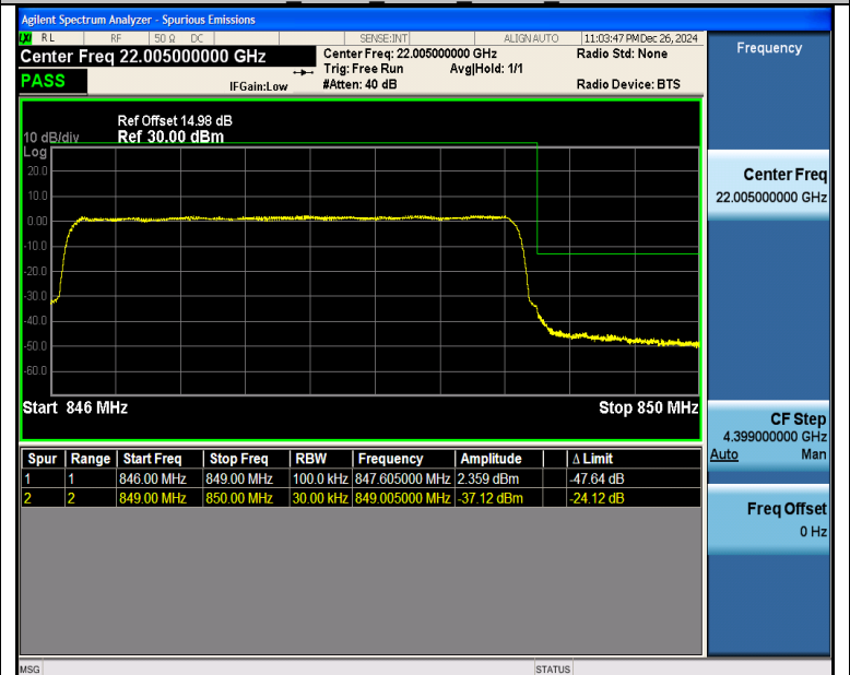
Band26 3MHz QPSK 27025 15RB#0
