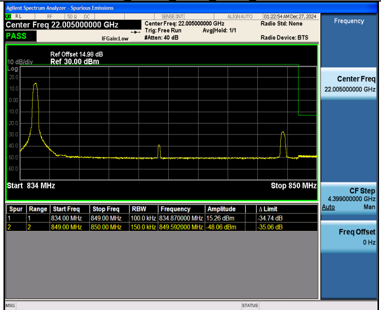
Band26 15MHz QPSK 26965 1RB#0
