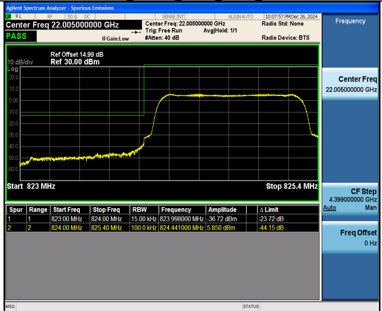
Band26 1.4MHz QPSK 26797 6RB#0
