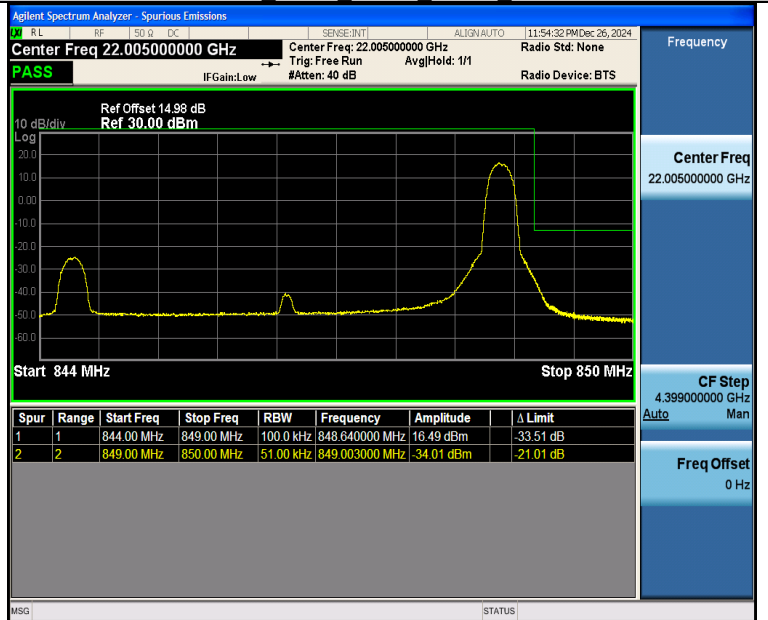
Band26 5MHz QPSK 27015 1RB#24
