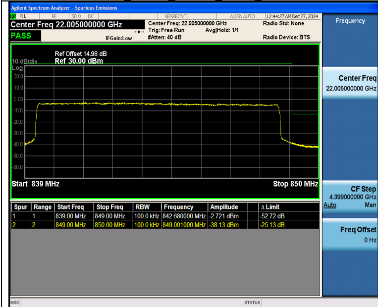
Band26 10MHz_QPSK_26990_50RB#0
