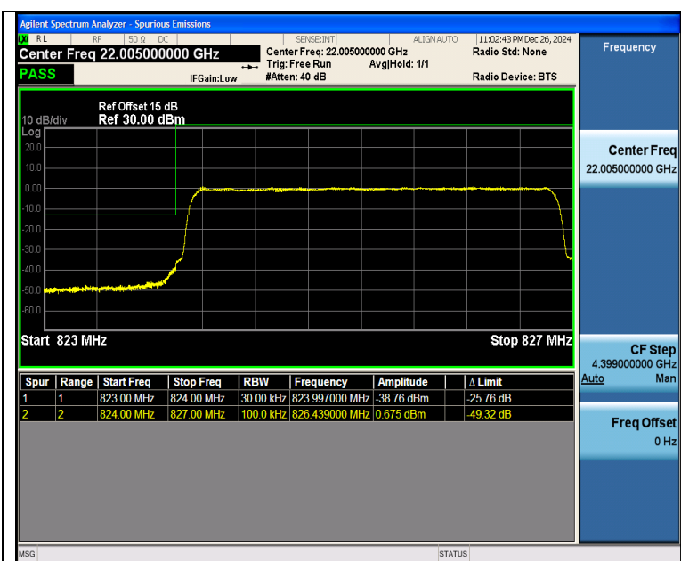
Band26 3MHz 16QAM 26805 15RB#0
