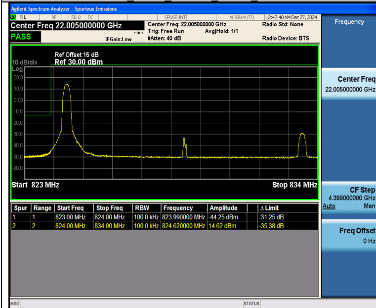
Band26 10MHz 16QAM 26840 1RB#0
