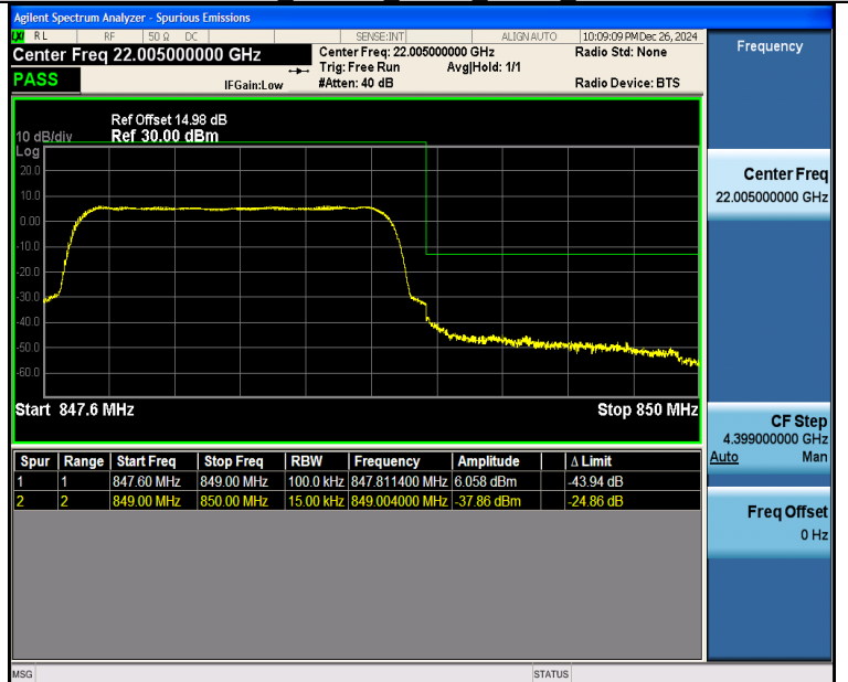
Band26 1.4MHz QPSK 27033 6RB#0
