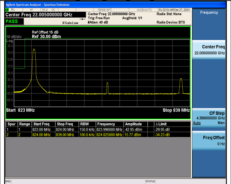
Band26 15MHz_QPSK_26865_1RB#0
