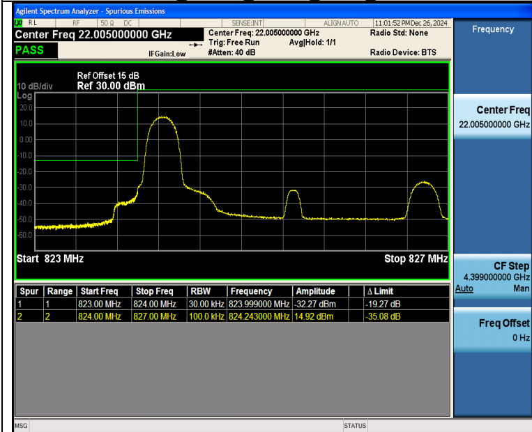
Band26 3MHz 16QAM 26805 1RB#0
