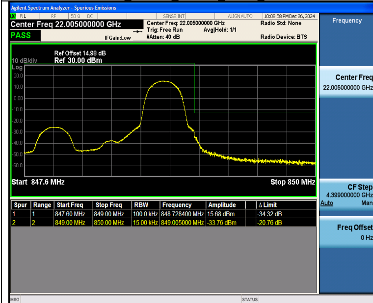
Band26 1.4MHz 16QAM 27033 1RB#5
