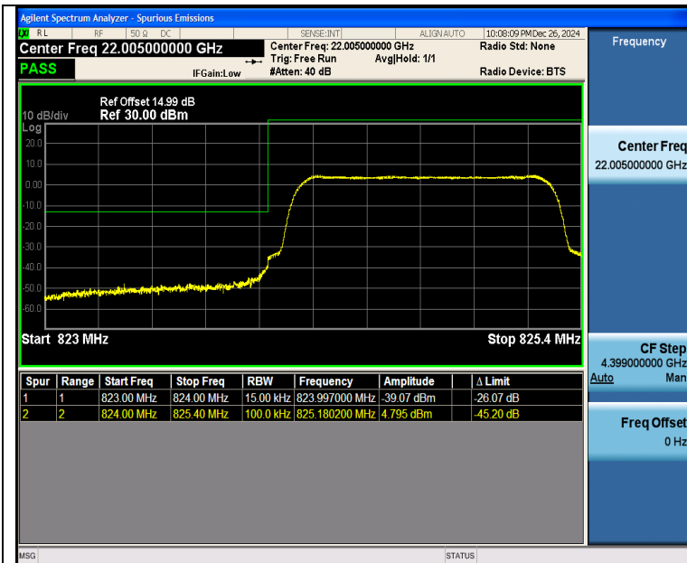
Band26 1.4MHz 16QAM 26797 6RB#0
