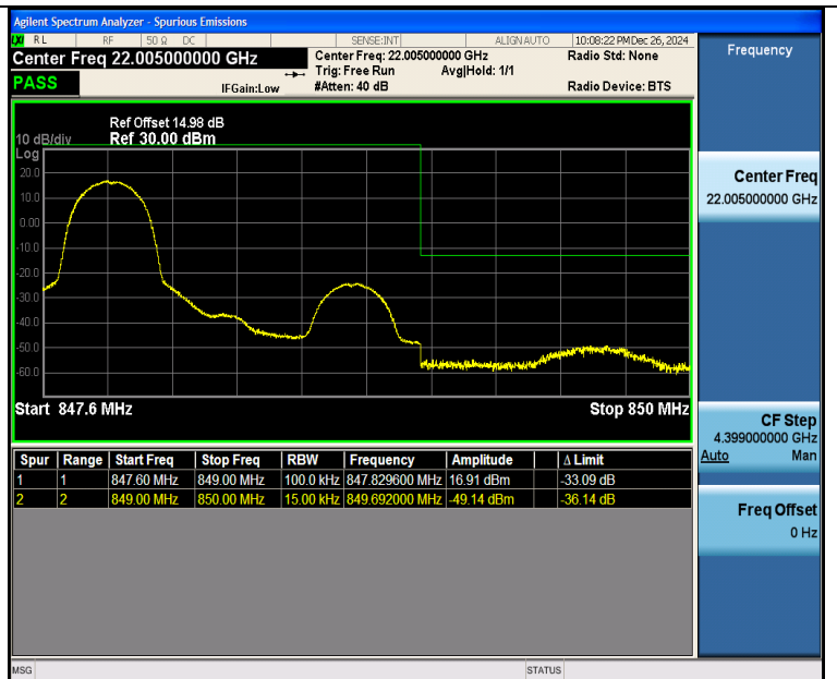
Band26 1.4MHz QPSK 27033 1RB#0
