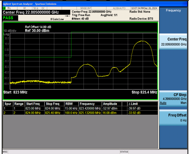
Band26 1.4MHz QPSK 26797 1RB#5
