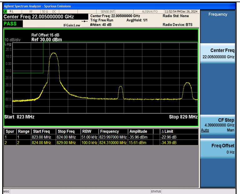
Band26 5MHz QPSK 26815 1RB#0
