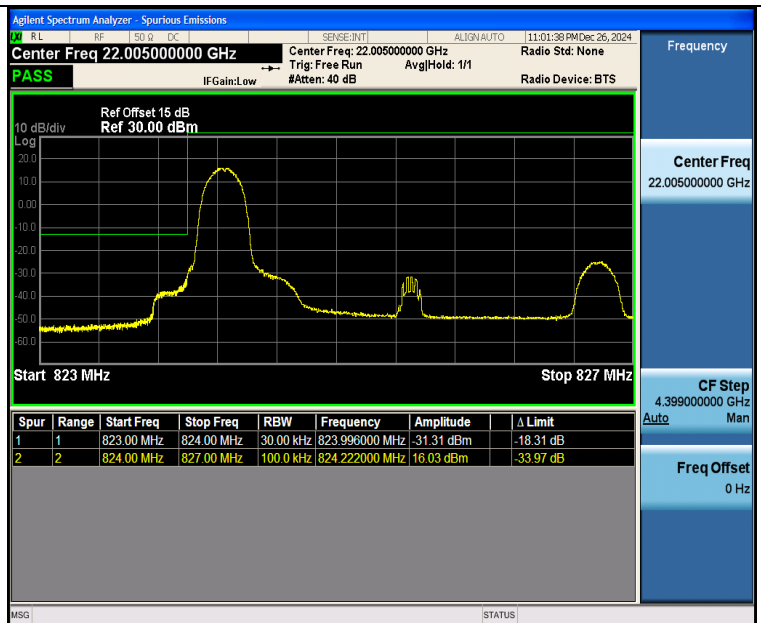
Band26 3MHz QPSK 26805 1RB#0
