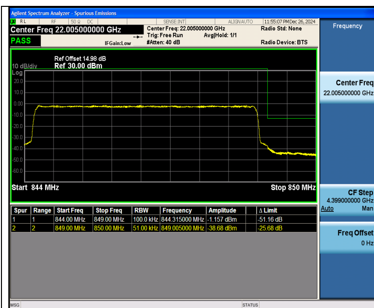
Band26 5MHz 16QAM 27015 25RB#0
