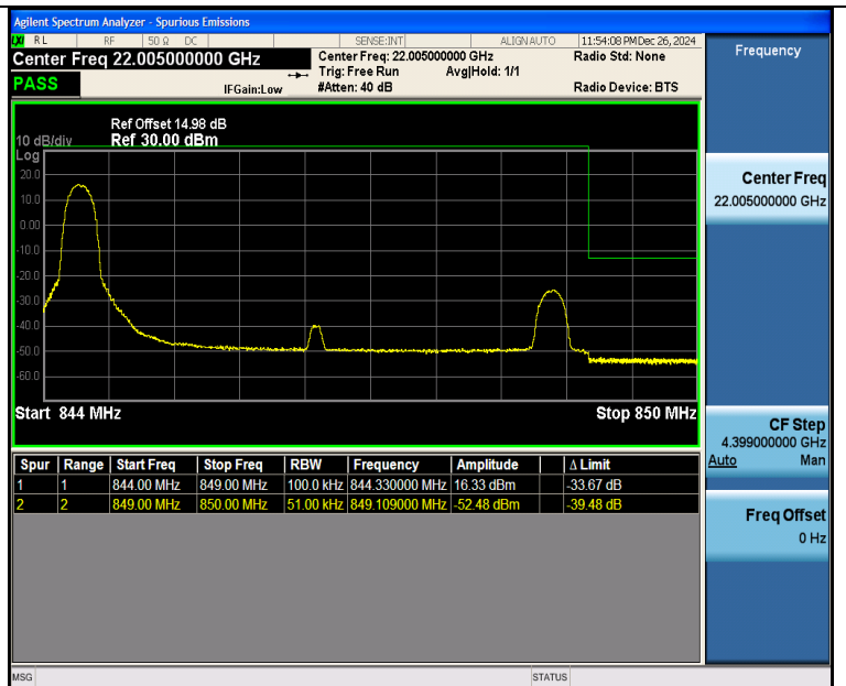
Band26 5MHz QPSK 27015 1RB#0
