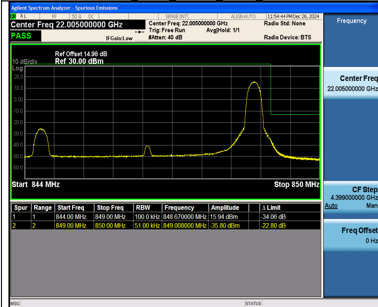
Band26 5MHz 16QAM 27015 1RB#24
