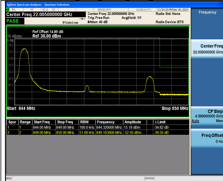
Band26 5MHz 16QAM 27015 1RB#0
