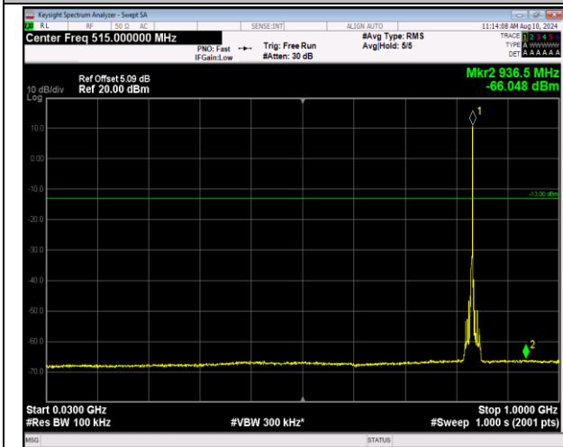
5-5-3MHz-5MHz-16QAM-16QAM-20501-20540-1RB#14- ORB#0-30~1000MHz-PASS
