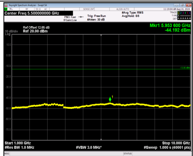
5-5-3MHz-5MHz-16QAM-16QAM-20586-20625-1RB#14-0R B#0-1000~10000MHz-PASS
