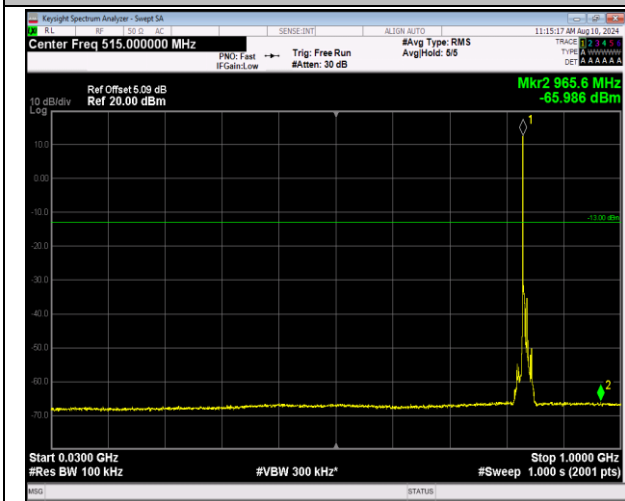
5-5-3MHz-5MHz-16QAM-16QAM-20501-20540-1RB#0-1 RB#24-30~1000MHz-PASS
