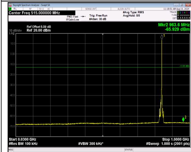
5-5-3MHz-5MHz-16QAM-16QAM-20586-20625-1RB#14- ORB#0-30~1000MHz-PASS
