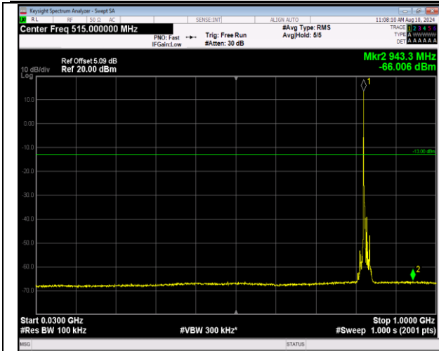
5-5-3MHz-5MHz-16QAM-16QAM-20416-20455-1RB#0-0 RB#0-30~1000MHz-PASS
