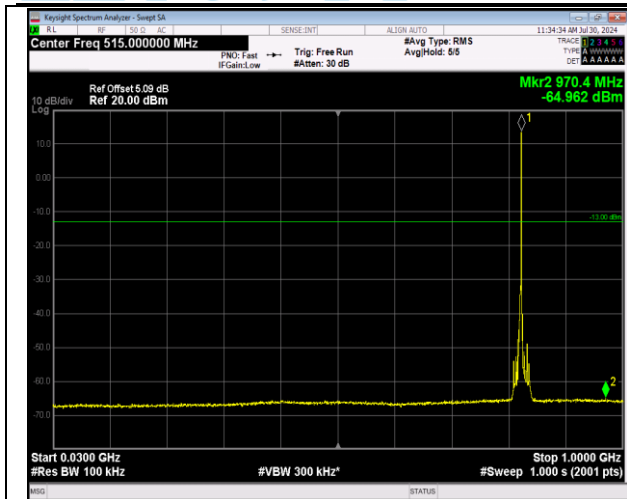
5-5-3MHz-5MHz-64QAM-64QAM-20416-20455-1RB#14- ORB#0-30~1000MHz-PASS
