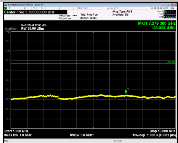
5-5-3MHz-5MHz-64QAM-64QAM-20586-20625-1RB#0-1RB#24-1000~10000MHz-PASS
