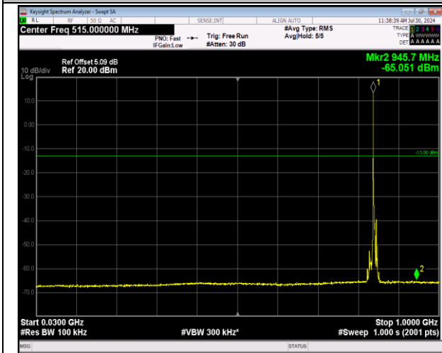
5-5-3MHz-5MHz-64QAM-64QAM-20586-20625-1RB#0-0RB#0-30~1000MHz-PASS
