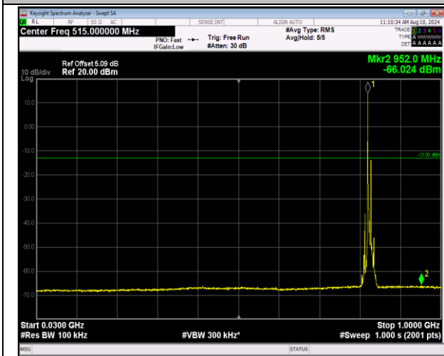
5-5-3MHz-5MHz-16QAM-16QAM-20416-20455-1RB#0-1 RB#24-30~1000MHz-PASS
