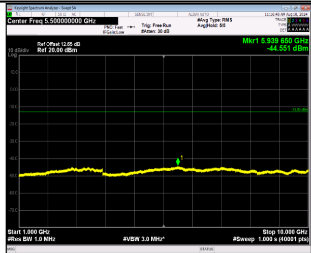
5-5-3MHz-5MHz-16QAM-16QAM-20501-20540-15RB#0-25RB#0-1000~10000MHz-PASS
