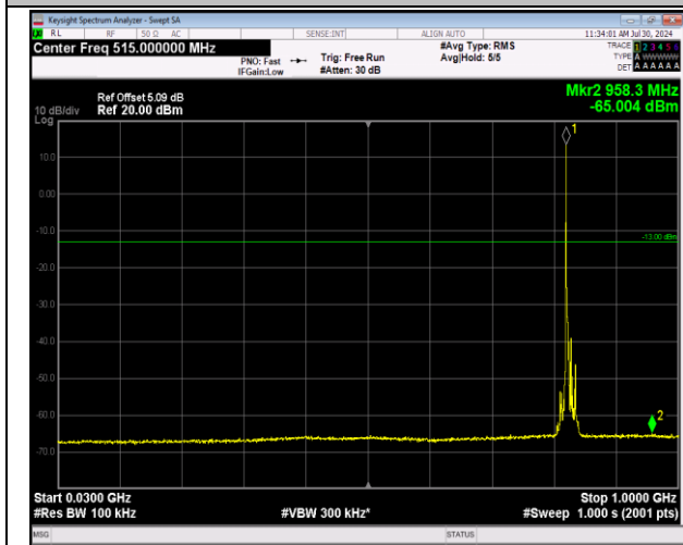
5-5-3MHz-5MHz-64QAM-64QAM-20416-20455-1RB#0-0-0RB#0-30~1000MHz-PASS
