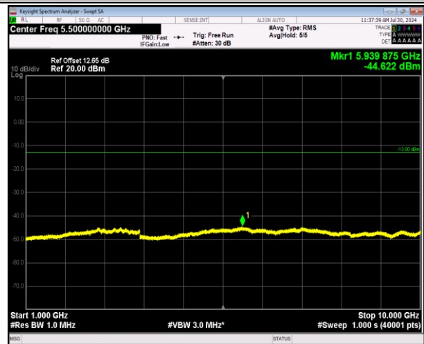
5-5-3MHz-5MHz-64QAM-64QAM-20501-20540-1RB#0-1-0RB#24-1000~10000MHz-PASS
