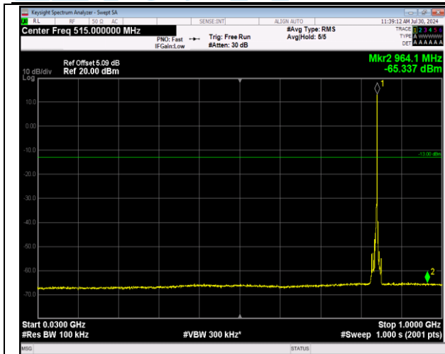
5-5-3MHz-5MHz-64QAM-64QAM-20586-20625-1RB#14- ORB#0-30~1000MHz-PASS
