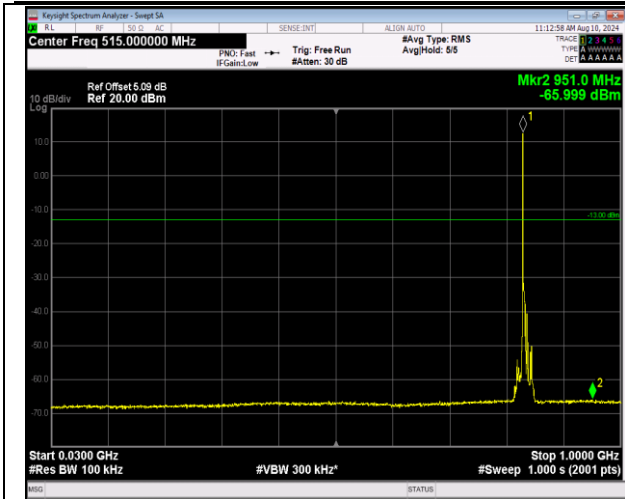
5-5-3MHz-5MHz-16QAM-16QAM-20501-20540-1RB#0-0 RB#0-30~1000MHz-PASS
