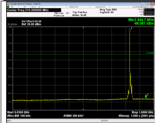
5-5-3MHz-5MHz-QPSK-QPSK-20501-20540-1RB#0-1RB #24-30~1000MHz-PASS
