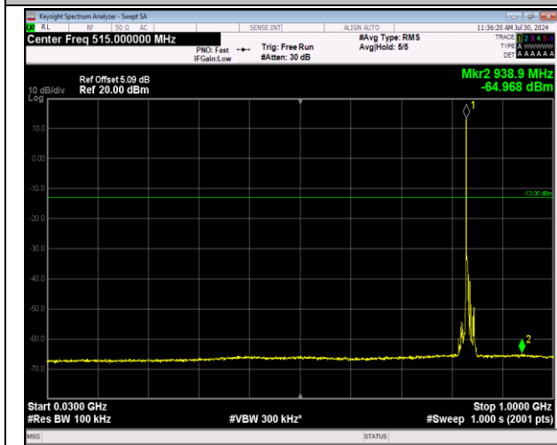
5-5-3MHz-5MHz-64QAM-64QAM-20501-20540-1RB#0-0-0RB#0-30~1000MHz-PASS
