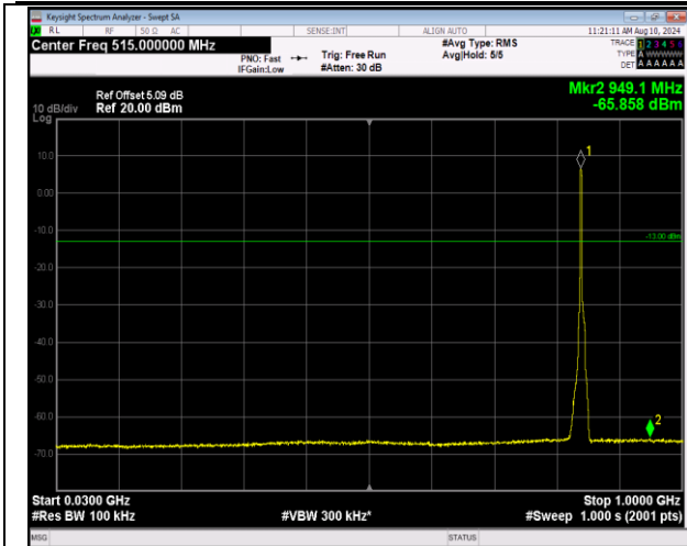
5-5-3MHz-5MHz-16QAM-16QAM-20586-20625-15RB#0-0-25RB#0-30~1000MHz-PASS
