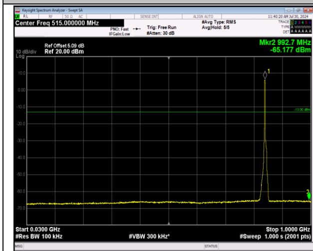
5-5-3MHz-5MHz-64QAM-64QAM-20586-20625-15RB#0- 25RB#0-30~1000MHz-PASS
