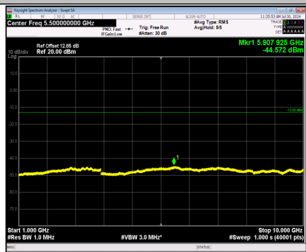
5-5-3MHz-5MHz-64QAM-64QAM-20416-20455-15RB#0-25 RB#0-1000~10000MHz-PASS
