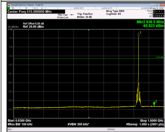
5-5-3MHz-5MHz-QPSK-QPSK-20501-20540-1RB#14-0R B#0-30~1000MHz-PASS
