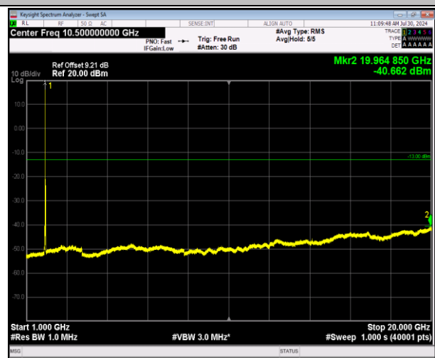
2-2-20MHz-20MHz-64QAM-64QAM-18902-19100-1RB#0-0 RB#0-1000~20000MHz-PASS
