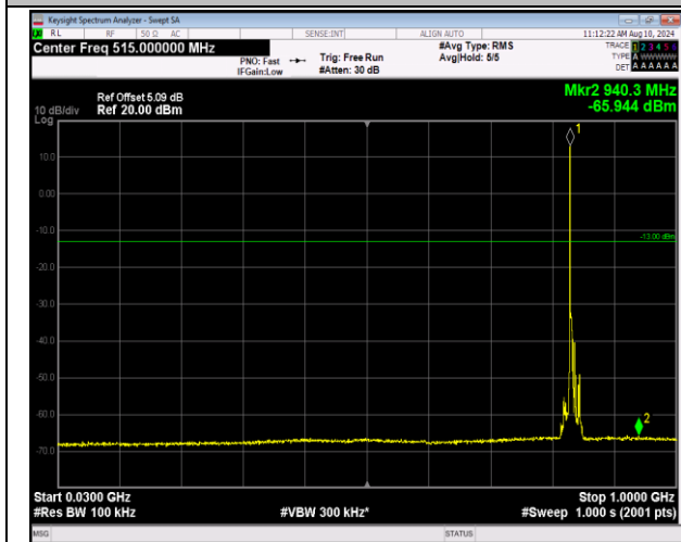
5-5-3MHz-5MHz-QPSK-QPSK-20501-20540-1RB#0-ORB #0-30~1000MHz-PASS
