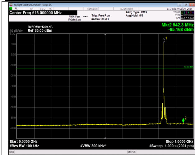
5-5-3MHz-5MHz-64QAM-64QAM-20501-20540-1RB#14-0RB#0-30~1000MHz-PASS
