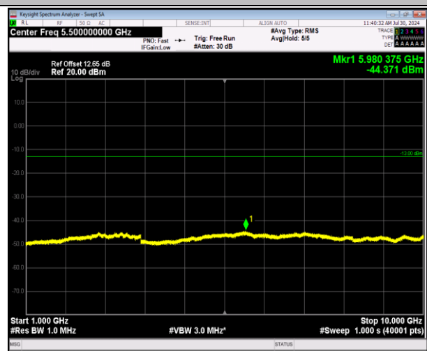
5-5-3MHz-5MHz-64QAM-64QAM-20586-20625-15RB#0-25 RB#0-1000~10000MHz-PASS
