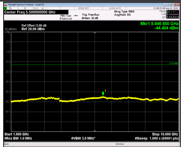
5-5-3MHz-5MHz-16QAM-16QAM-20416-20455-1RB#0-0R B#0-1000~10000MHz-PASS
