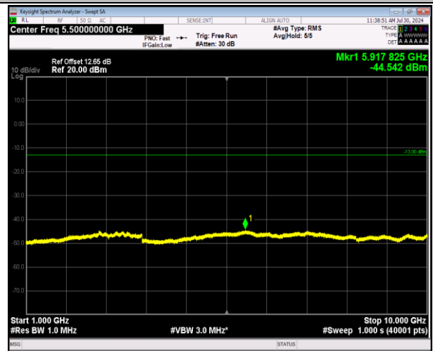
5-5-3MHz-5MHz-64QAM-64QAM-20586-20625-1RB#0-0RB#0-1000~10000MHz-PASS
