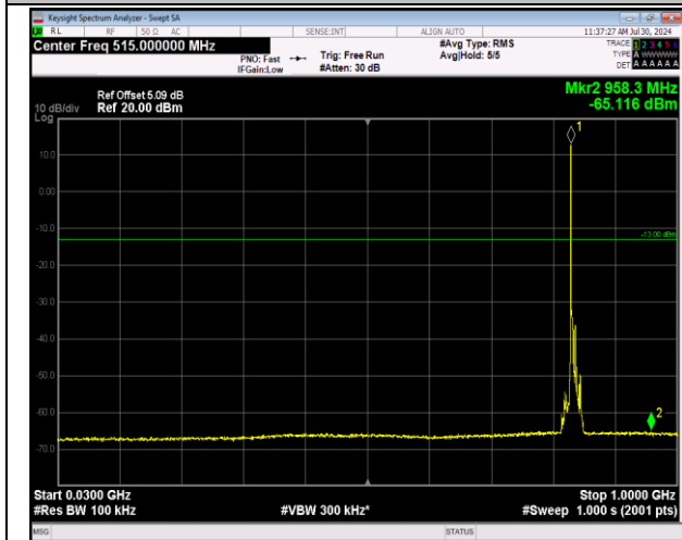
5-5-3MHz-5MHz-64QAM-64QAM-20501-20540-1RB#0-0-1RB#24-30~1000MHz-PASS
