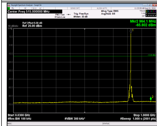
5-5-5MHz-3MHz-QPSK-QPSK-20425-20464-1RB#24-0R B#0-30~1000MHz-PASS
