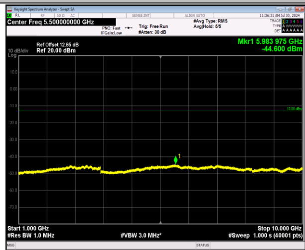
5-5-3MHz-5MHz-64QAM-64QAM-20501-20540-1RB#0-0-0RB#0-1000~10000MHz-PASS
