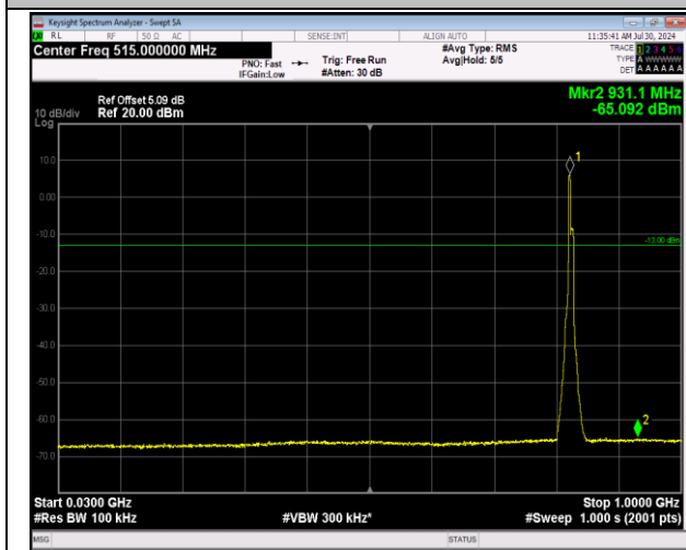
5-5-3MHz-5MHz-64QAM-64QAM-20416-20455-15RB#0- 25RB#0-30~1000MHz-PASS
