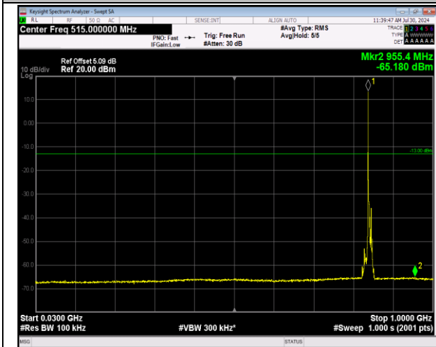
5-5-3MHz-5MHz-64QAM-64QAM-20586-20625-1RB#0-1RB#24-30~1000MHz-PASS
