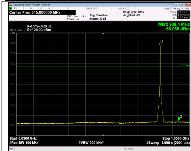
5-5-3MHz-5MHz-16QAM-16QAM-20501-20540-15RB#0-0-25RB#0-30~1000MHz-PASS
