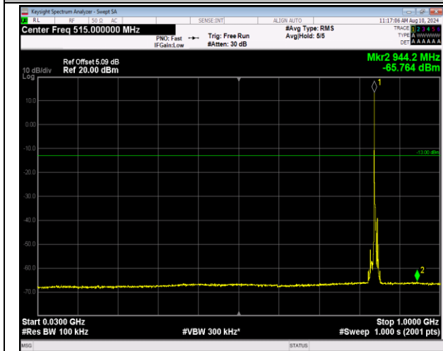
5-5-3MHz-5MHz-QPSK-QPSK-20586-20625-1RB#0-0RB#0-30~1000MHz-PASS
