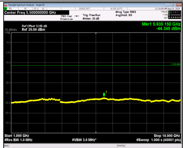
5-5-3MHz-5MHz-QPSK-QPSK-20501-20540-15RB#0-25RB #0-1000~10000MHz-PASS
