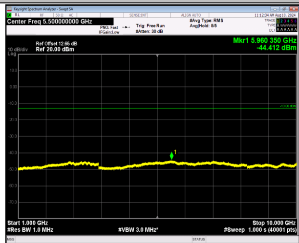
5-5-3MHz-5MHz-QPSK-QPSK-20501-20540-1RB#0-ORB#0 -1000~10000MHz-PASS
