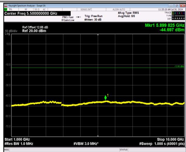
5-5-3MHz-5MHz-64QAM-64QAM-20416-20455-1RB#0-1R B#24-1000~10000MHz-PASS
