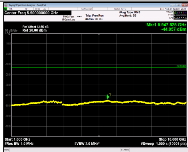
5-5-3MHz-5MHz-QPSK-QPSK-20586-20625-1RB#0-0RB#0-1000~10000MHz-PASS
