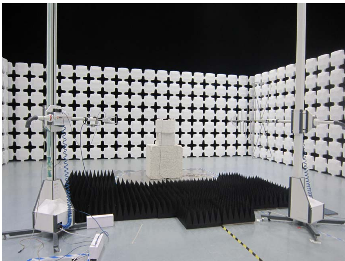
Spurious Emission
