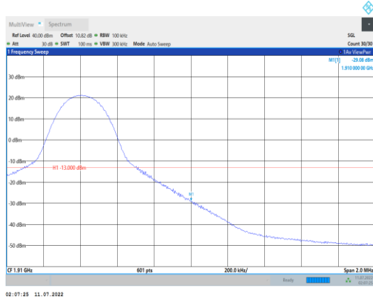
Band2-10MHz-QPSK-19150-1RB#49
