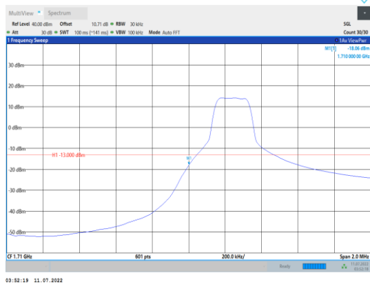
Band4-3MHz-16QAM-19965-1RB#0
