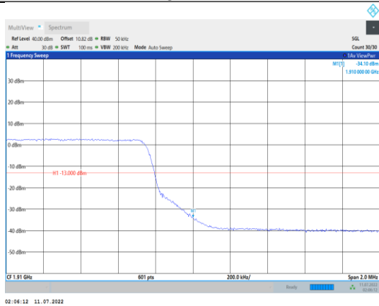
Band2-5MHz-QPSK-19175-25RB#0
