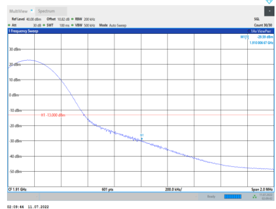
Band2-15MHz-QPSK-19125-1RB#74
