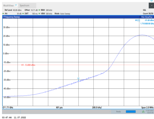
Band4-15MHz-16QAM-20025-1RB#0
