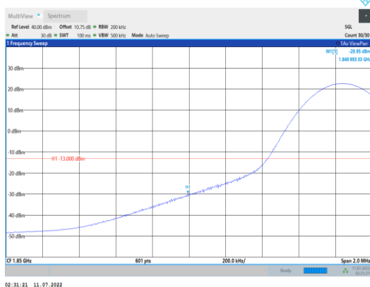
Band2-15MHz-QPSK-18675-1RB#0
