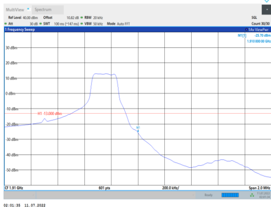
Band2-1.4MHz-16QAM-19193-1RB#5
