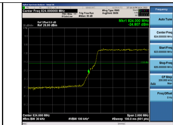
Band5-3MHz-QPSK-20415-15RB#0
