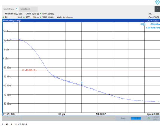
Band4-15MHz-16QAM-20325-1RB#74
