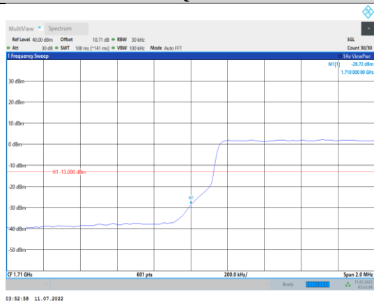
Band4-3MHz-16QAM-19965-15RB#0
