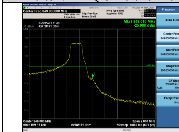
Band5-1.4MHz-QPSK-20643-1RB#5
