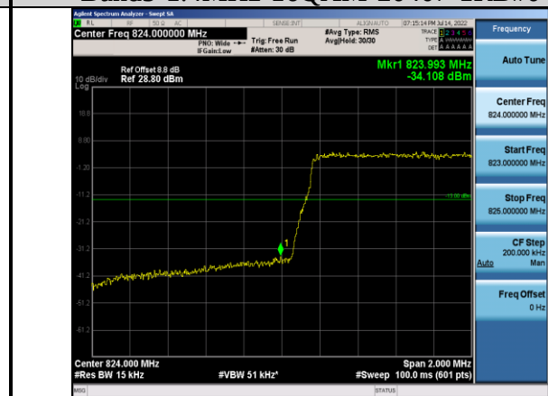
Band5-1.4MHz-16QAM-20407-6RB#0
