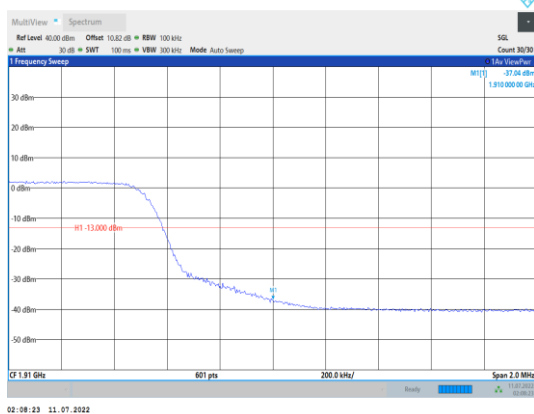
Band2-10MHz-16QAM-19150-50RB#0
