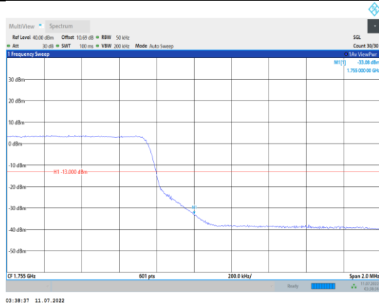
Band4-5MHz-QPSK-20375-25RB#0
