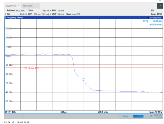
Band2-3MHz-16QAM-19185-15RB#0
