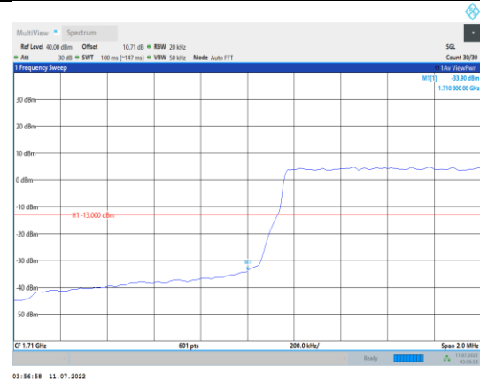
Band4-1.4MHz-16QAM-19957-6RB#0
