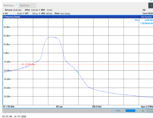
Band4-5MHz-QPSK-20375-1RB#24
