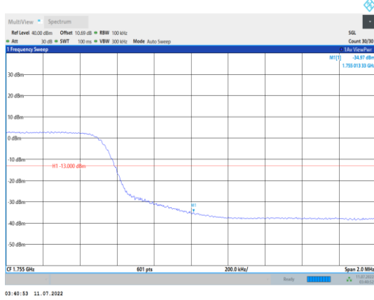
Band4-10MHz-16QAM-20350-50RB#0
