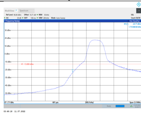
Band4-5MHz-QPSK-19975-1RB#0
