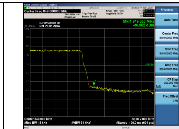
Band5-1.4MHz-QPSK-20643-6RB#0
