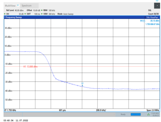
Band4-10MHz-QPSK-20350-50RB#0
