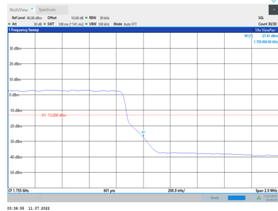
Band4-3MHz-16QAM-20385-15RB#0
