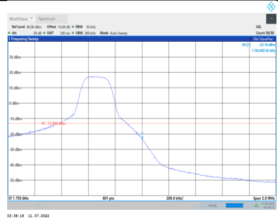
Band4-5MHz-16QAM-20375-1RB#24
