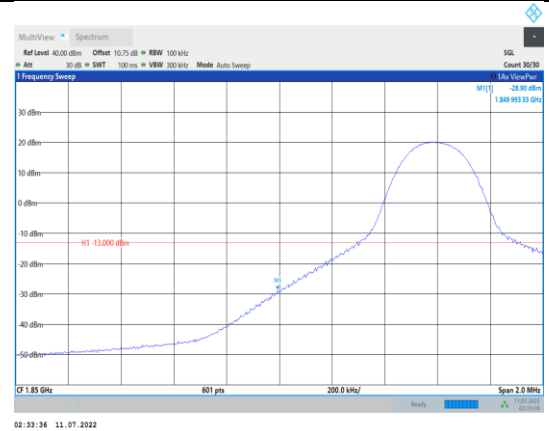
Band2-10MHz-16QAM-18650-1RB#0
