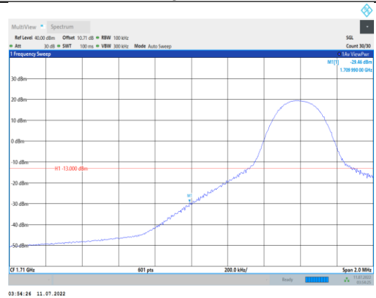
Band4-10MHz-16QAM-20000-1RB#0
