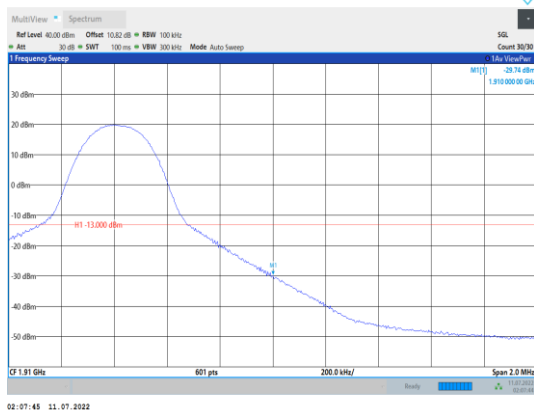
Band2-10MHz-16QAM-19150-1RB#49
