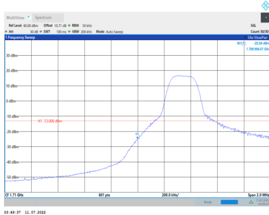
Band4-5MHz-16QAM-19975-1RB#0
