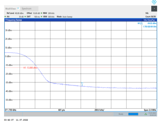
Band4-15MHz-QPSK-20325-75RB#0
