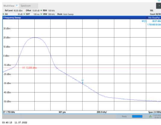
Band4-10MHz-16QAM-20350-1RB#49
