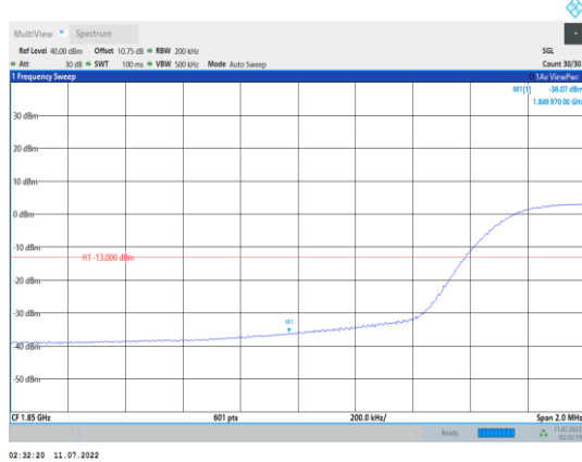
Band2-15MHz-16QAM-18675-75RB#0
