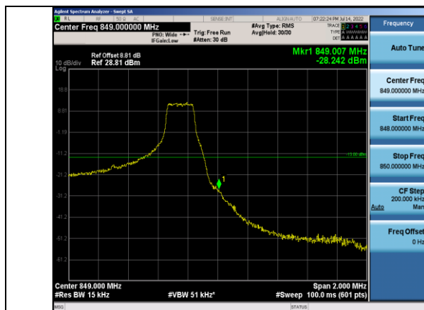
Band5-1.4MHz-16QAM-20643-1RB#5
