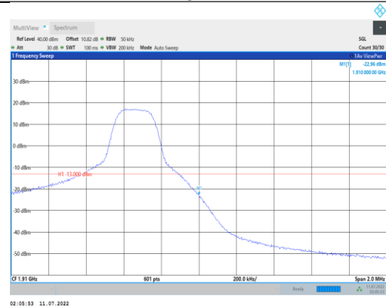
Band2-5MHz-16QAM-19175-1RB#24
