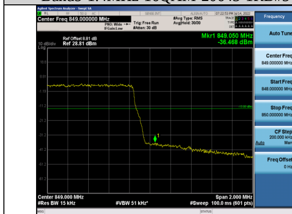
Band5-1.4MHz-16QAM-20643-6RB#0
