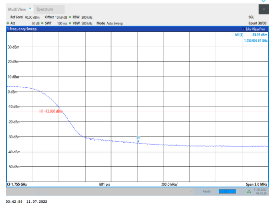
Band4-15MHz-16QAM-20325-75RB#0
