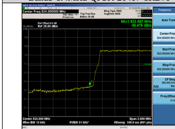
Band5-1.4MHz-QPSK-20407-6RB#0
