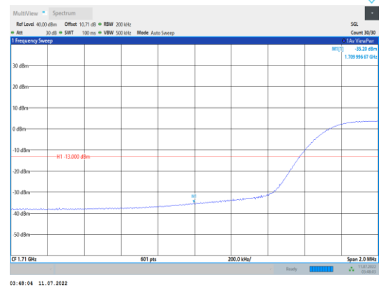
Band4-15MHz-QPSK-20025-75RB#0
