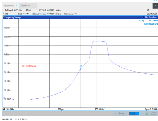
Band2-3MHz-16QAM-18615-1RB#0
