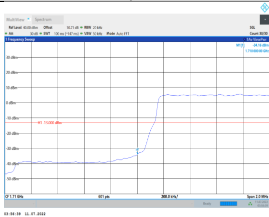
Band4-1.4MHz-QPSK-19957-6RB#0
