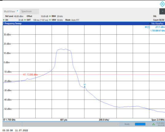
Band4-1.4MHz-QPSK-20393-1RB#5
