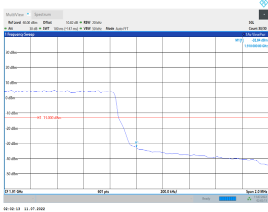
Band2-1.4MHz-16QAM-19193-6RB#0
