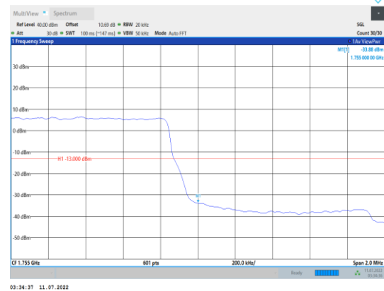
Band4-1.4MHz-QPSK-20393-6RB#0
