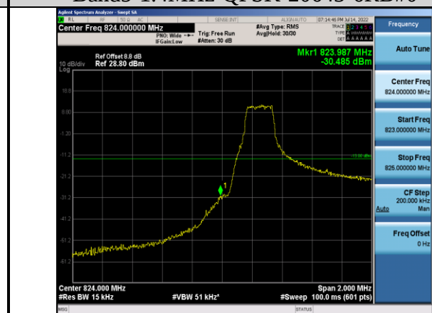
Band5-1.4MHz-16QAM-20407-1RB#0
