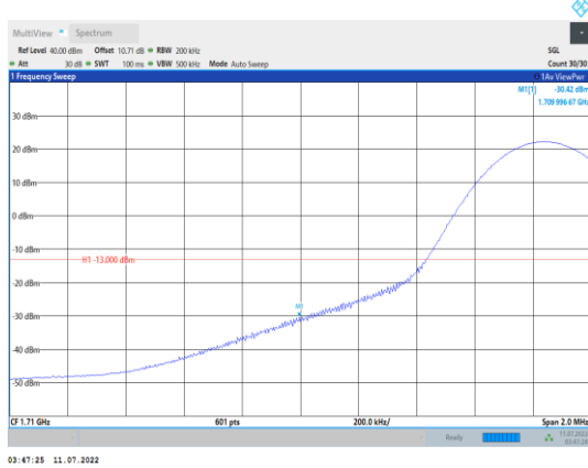
Band4-15MHz-QPSK-20025-1RB#0
