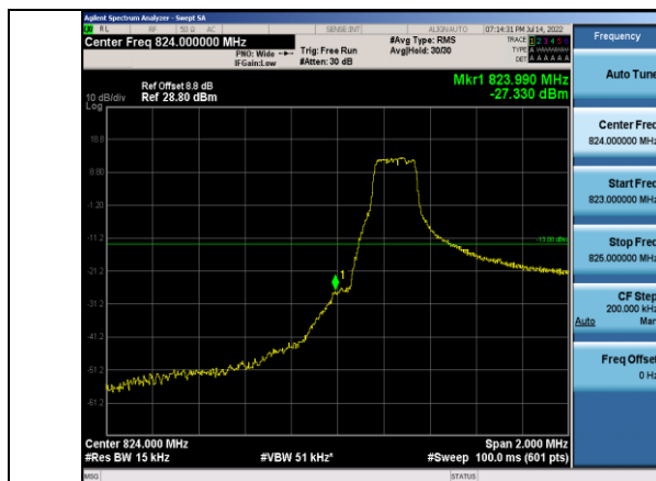
Band5-1.4MHz-QPSK-20407-1RB#0
