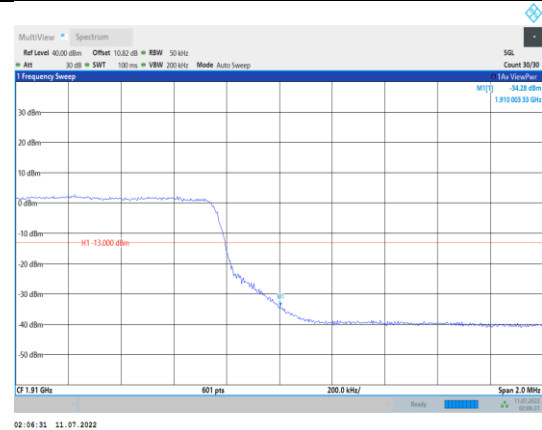
Band2-5MHz-16QAM-19175-25RB#0
