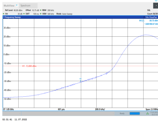
Band2-15MHz-16QAM-18675-1RB#0
