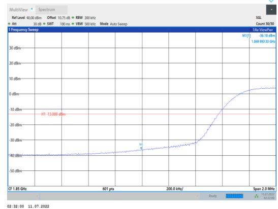
Band2-15MHz-QPSK-18675-75RB#0
