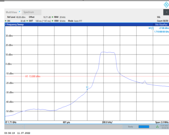
Band4-1.4MHz-16QAM-19957-1RB#0
