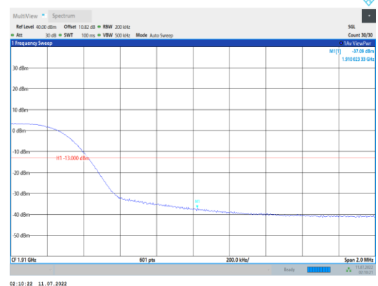
Band2-15MHz-QPSK-19125-75RB#0
