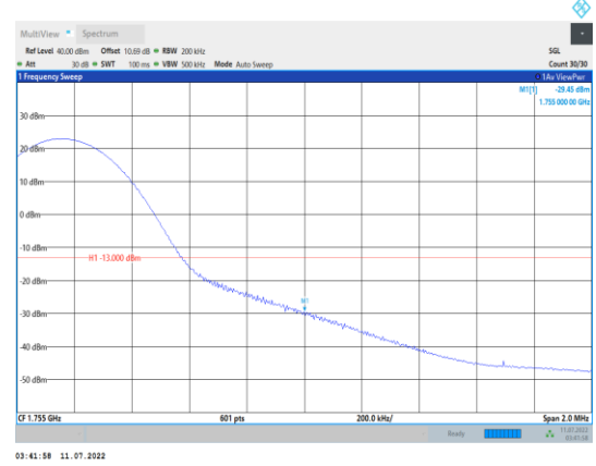
Band4-15MHz-QPSK-20325-1RB#74
