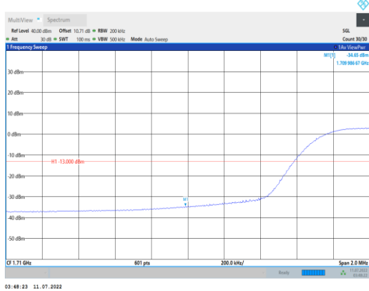
Band4-15MHz-16QAM-20025-75RB#0
