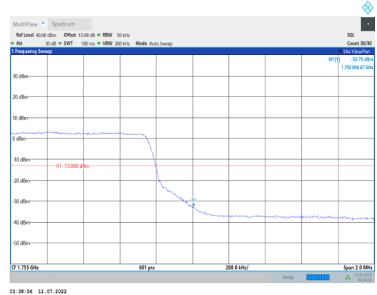
Band4-5MHz-16QAM-20375-25RB#0
