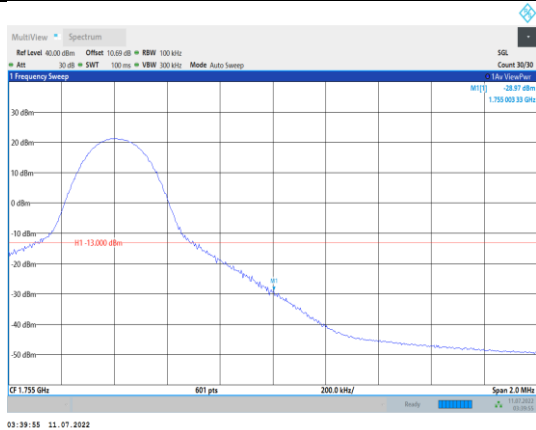
Band4-10MHz-QPSK-20350-1RB#49
