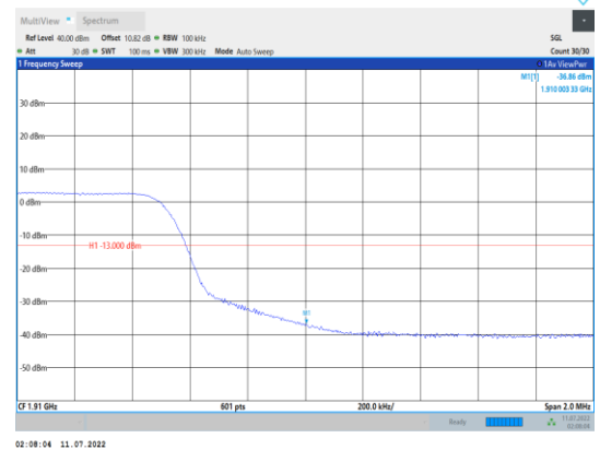
Band2-10MHz-QPSK-19150-50RB#0
