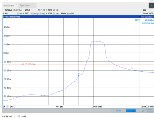
Band4-1.4MHz-QPSK-19957-1RB#0
