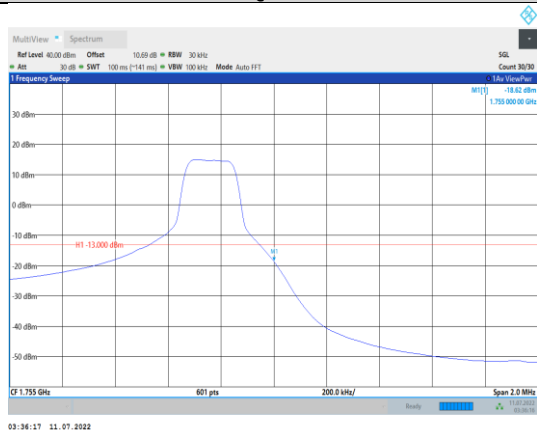
Band4-3MHz-16QAM-20385-1RB#14
