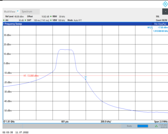
Band2-3MHz-16QAM-19185-1RB#14
