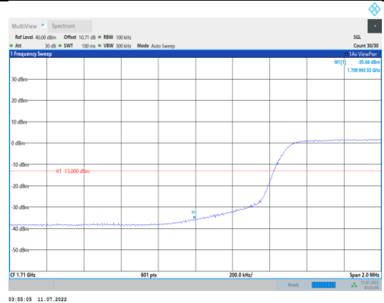
Band4-10MHz-16QAM-20000-50RB#0
