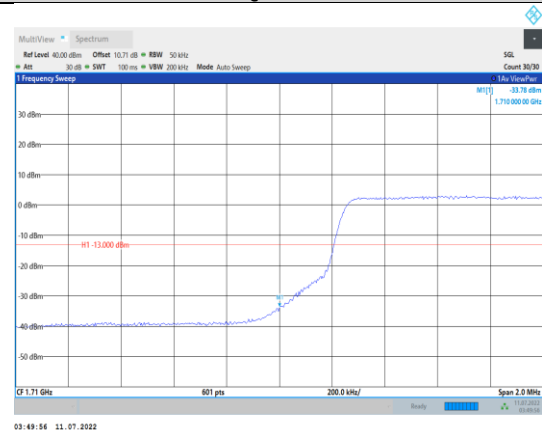
Band4-5MHz-QPSK-19975-25RB#0
