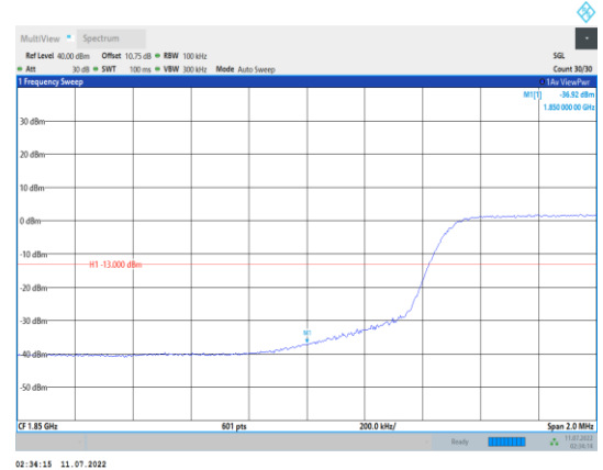
Band2-10MHz-16QAM-18650-50RB#0
