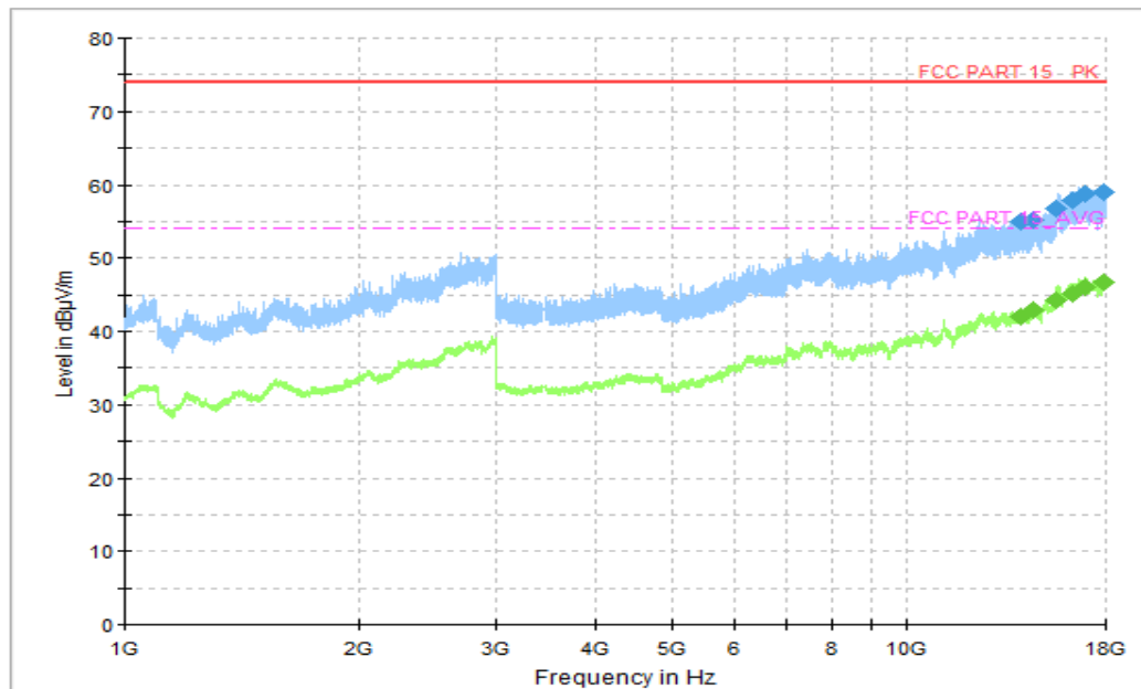
Figure A.1.29. Radiated Emission (Camera,1GHz to 18GHz)
