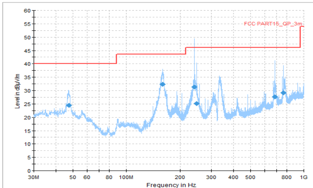
Figure A.1.34. Radiated Emission (Data Transfer: PC to EUT,30MHz to 1GHz)
