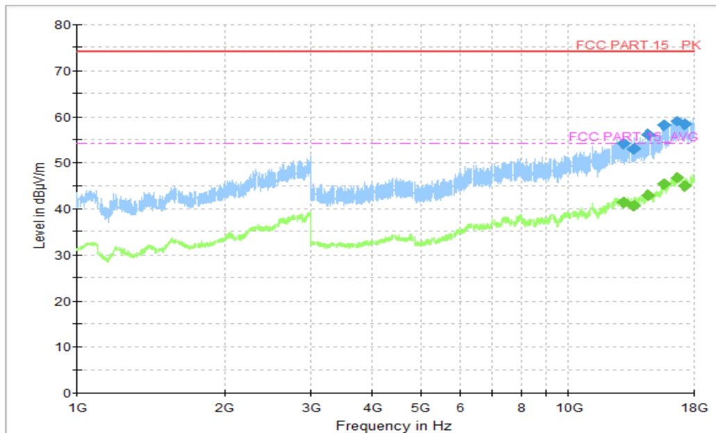
Figure A.1.23. Radiated Emission (Video Player,1GHz to 18GHz)
