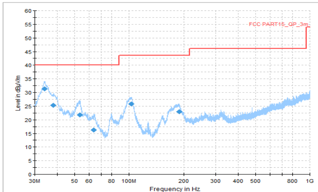
Figure A.1.25. Radiated Emission (Camera, 30MHz to 1GHz)
