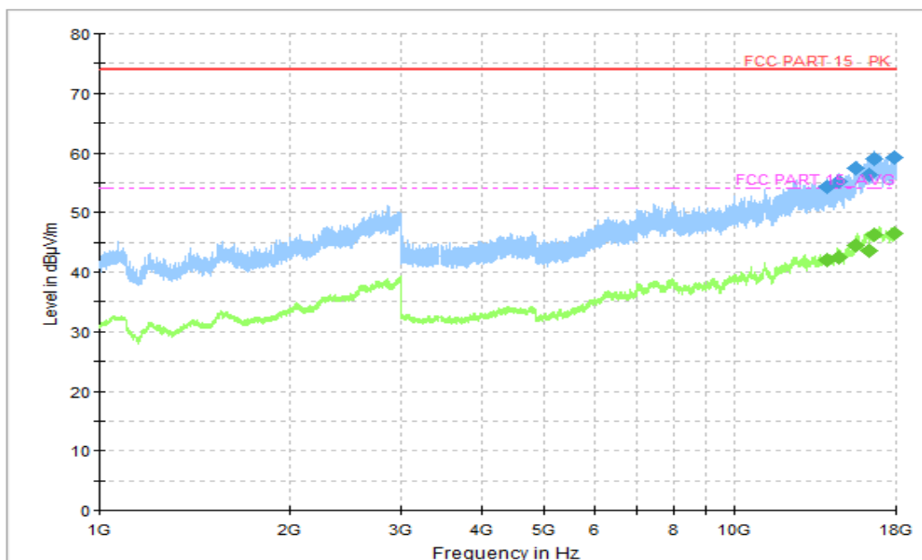
Figure A.1.41. Radiated Emission (Data Transfer: TF Card to PC,1GHz to 18GHz)
