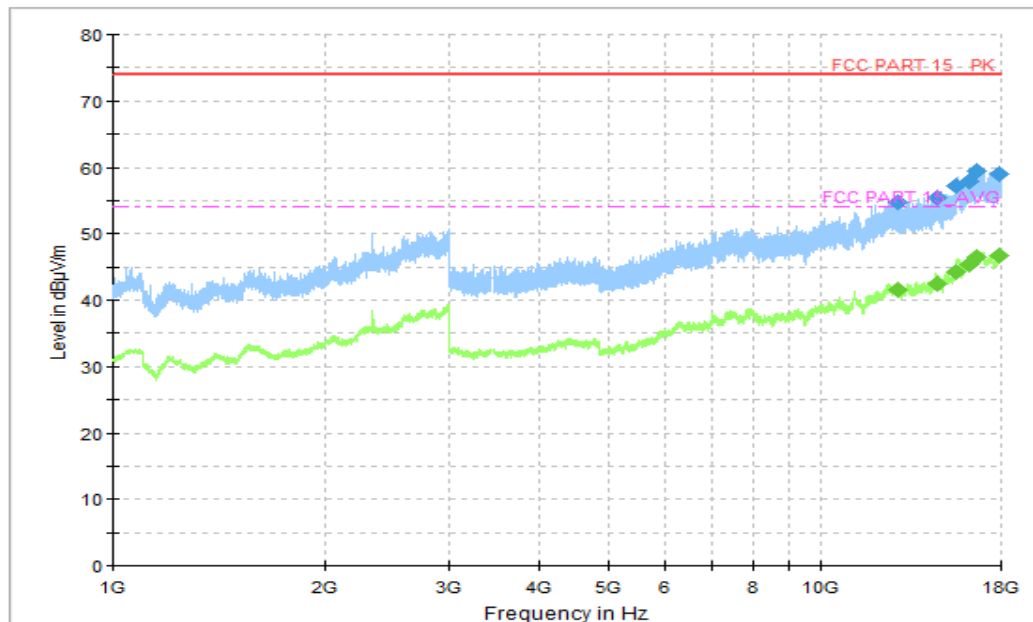
Figure A.1.11. Radiated Emission (LTE Receiver Band 12,,1GHz to 18GHz)
