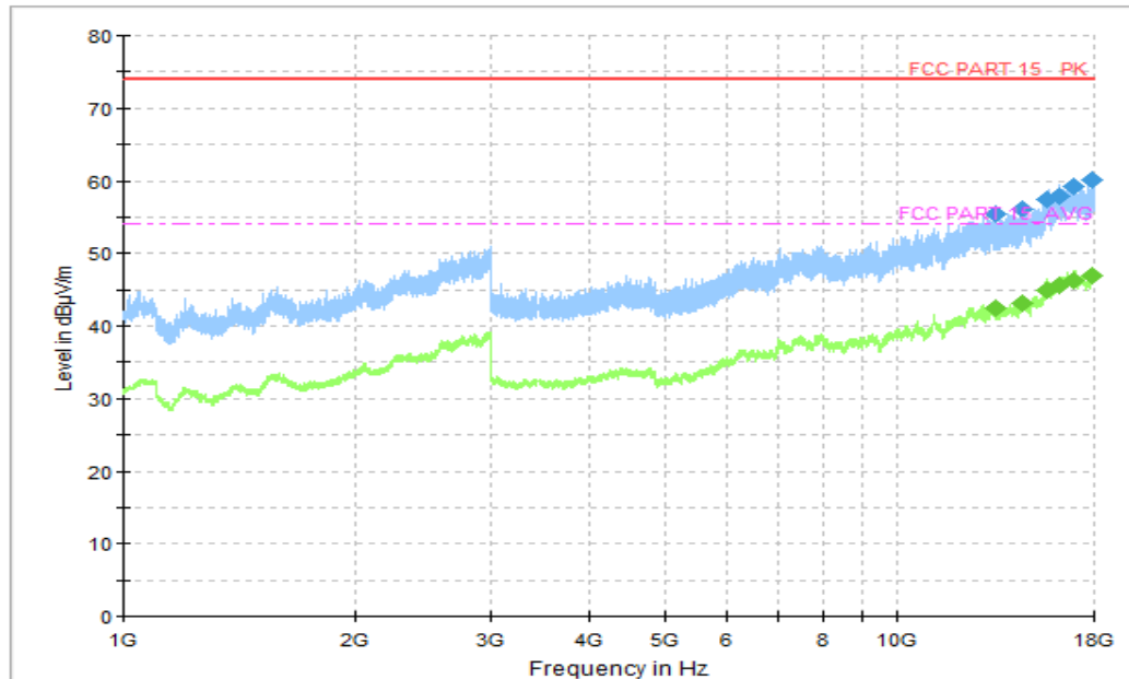
Figure A.1.44. Radiated Emission (Data Transfer: TF Card to PC,1GHz to 18GHz)
