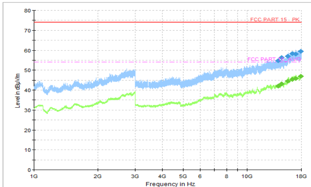
Figure A.1.35. Radiated Emission (Data Transfer: PC to EUT,1GHz to 18GHz)
