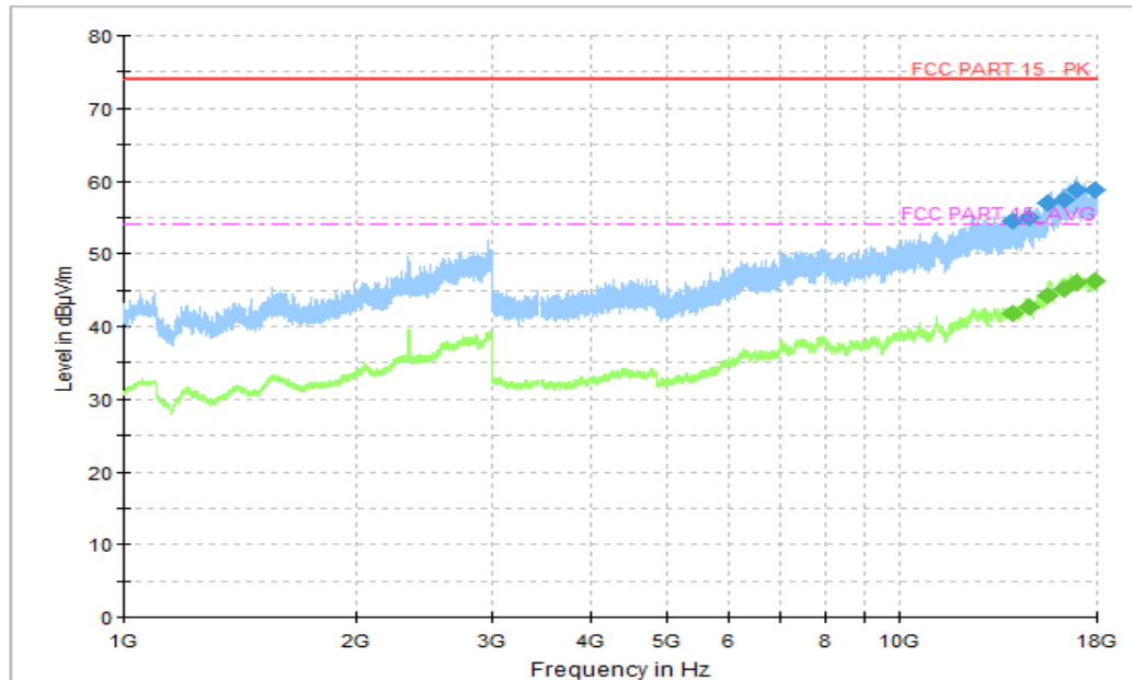
Figure A.1.26. Radiated Emission (Camera,1GHz to 18GHz)
