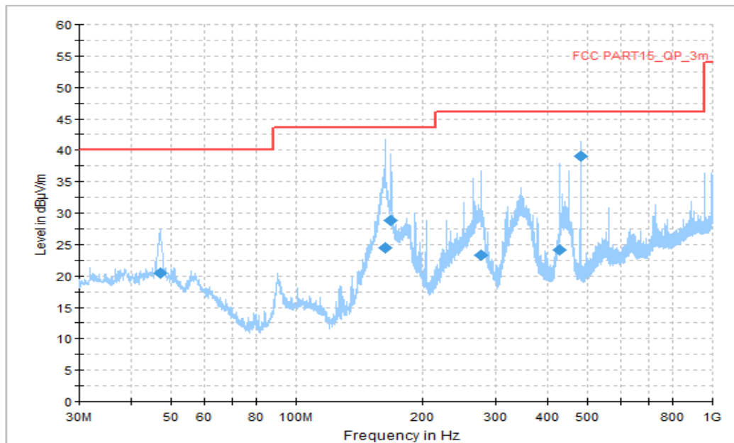
Figure A.1.43. Radiated Emission (Data Transfer: TF Card to PC,30MHz to 1GHz)
