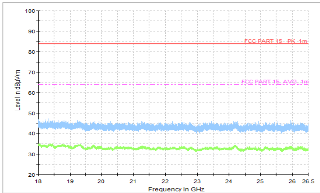
Figure A.1.27. Radiated Emission (Camera,18GHz to 26.5GHz)
