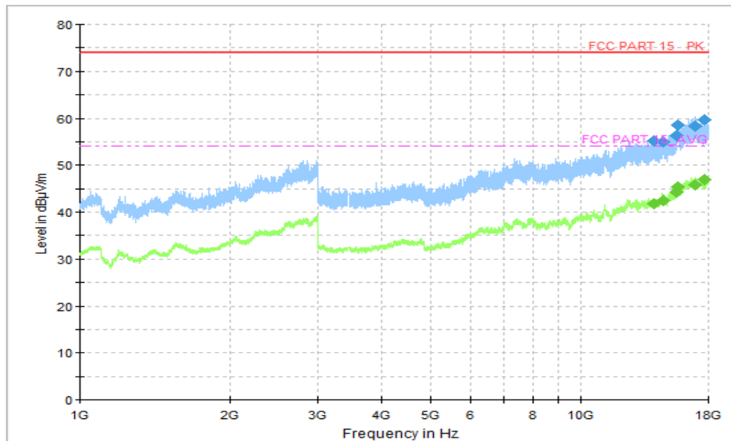
Figure A.1.17. Radiated Emission (GSM Receiver 850MHz,1GHz to 18GHz)
