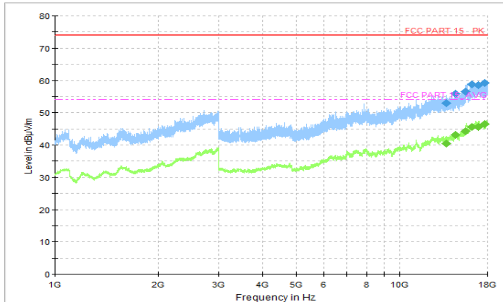
Figure A.1.38. Radiated Emission (Data Transfer: PC to TF Card,1GHz to 18GHz)
