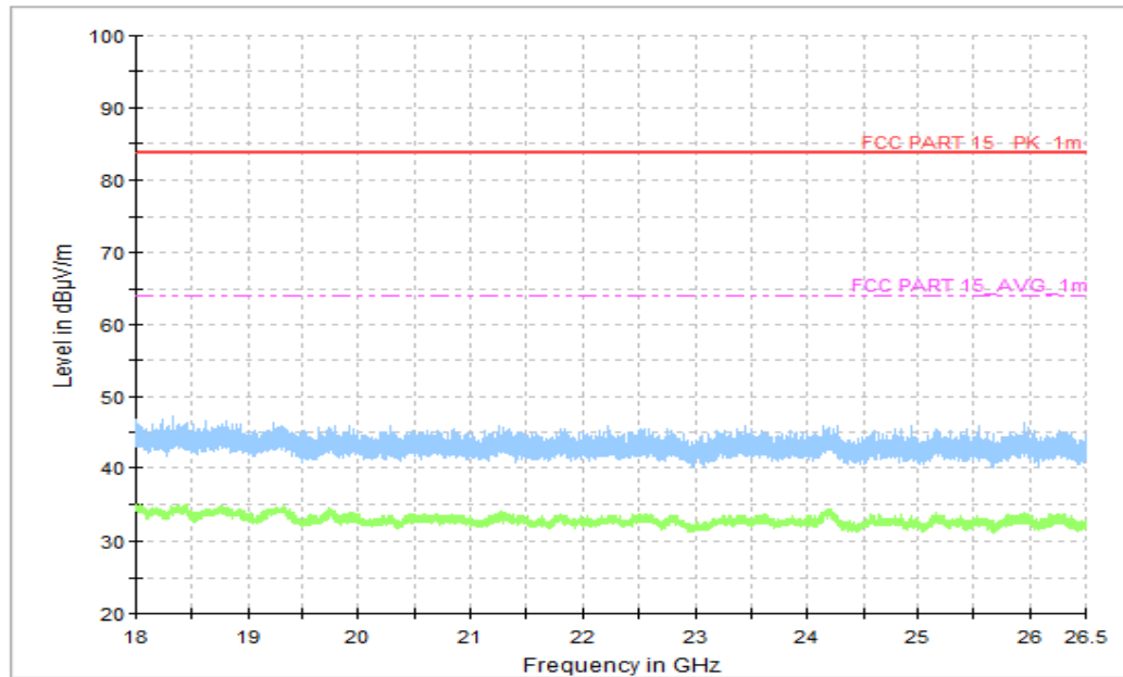
Figure A.1.12. Radiated Emission (LTE Receiver Band 12 ,18GHz to 26.5GHz)
