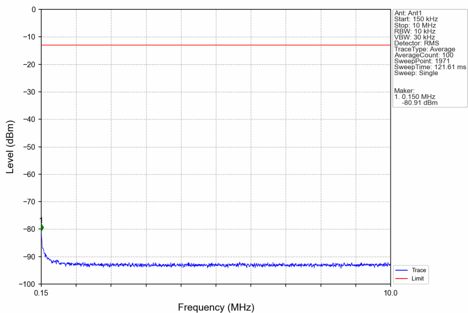
Band12_5MHz_QPSK_MCH_707.5MHz_RB_1_0_NTNV
