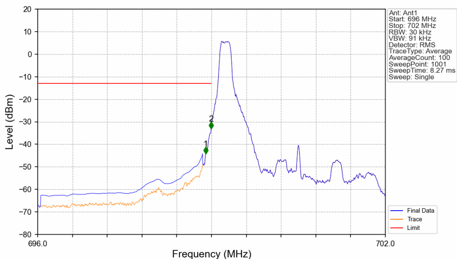
Band12_3MHz_QPSK_LCH_700.5MHz_RB_1_0_NTNV
