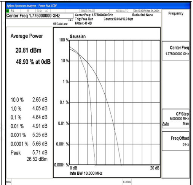
Band66-10MHz-16QAM-132622-1RB#0-PASS
