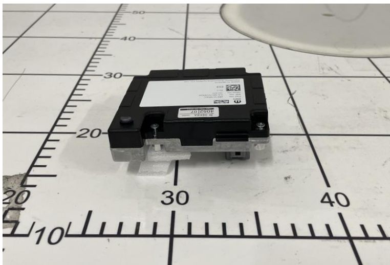
Figure B.3: DUT side view
