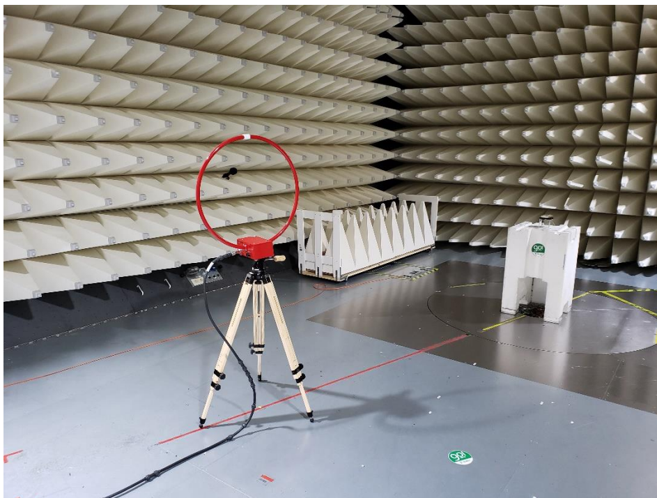
Figure B.6: Radiated Test setup 1
