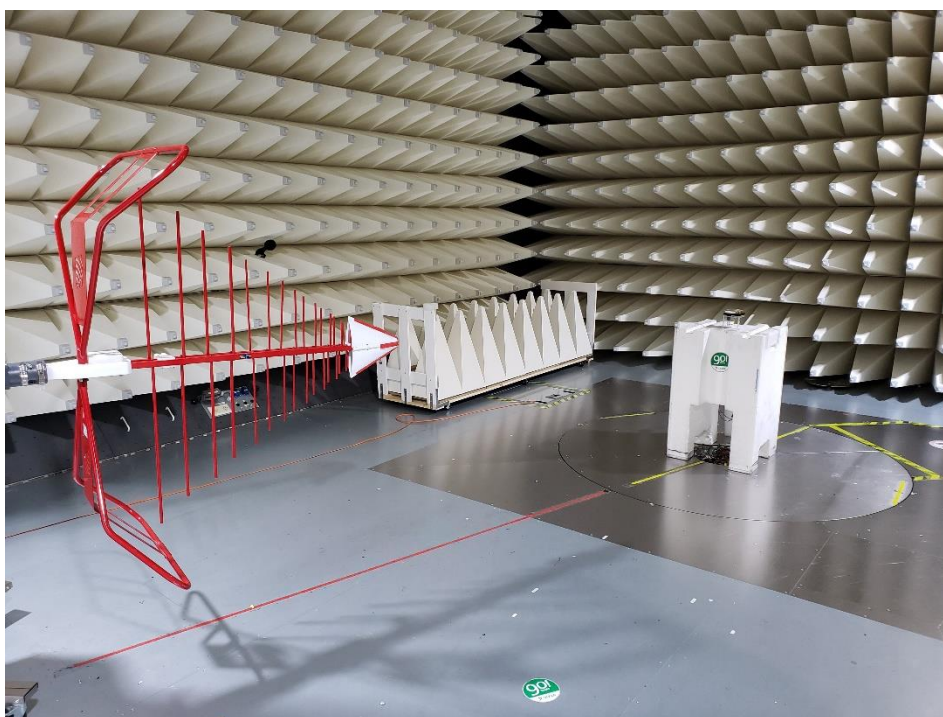
Figure B.7: Radiated Test setup 2
