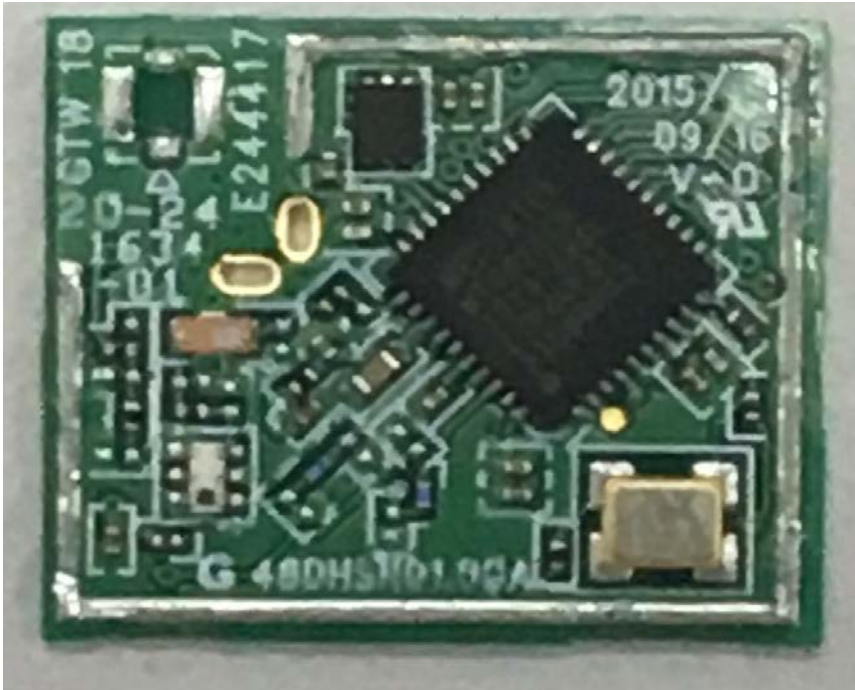
Top Without shield case
