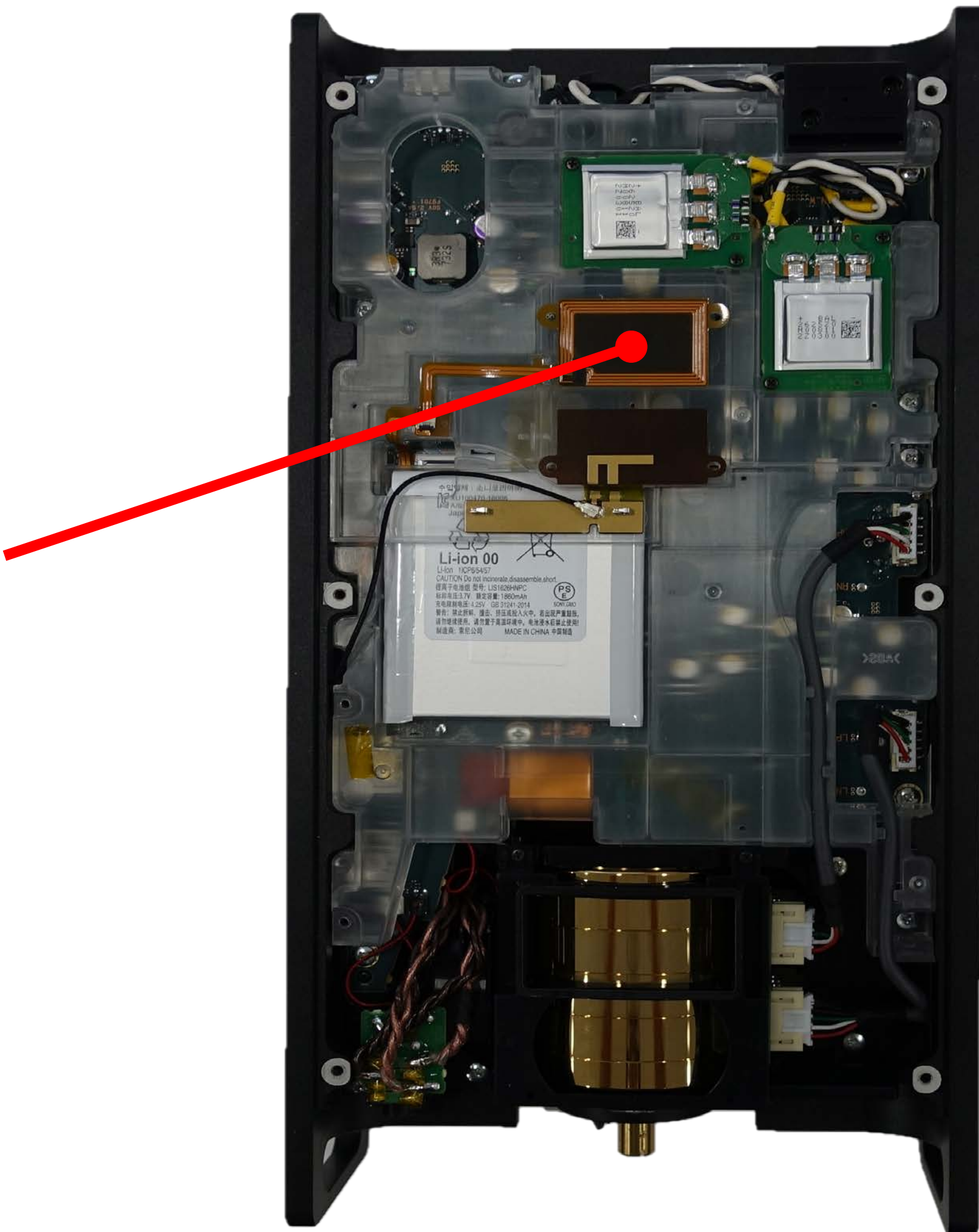
Top side of the product
