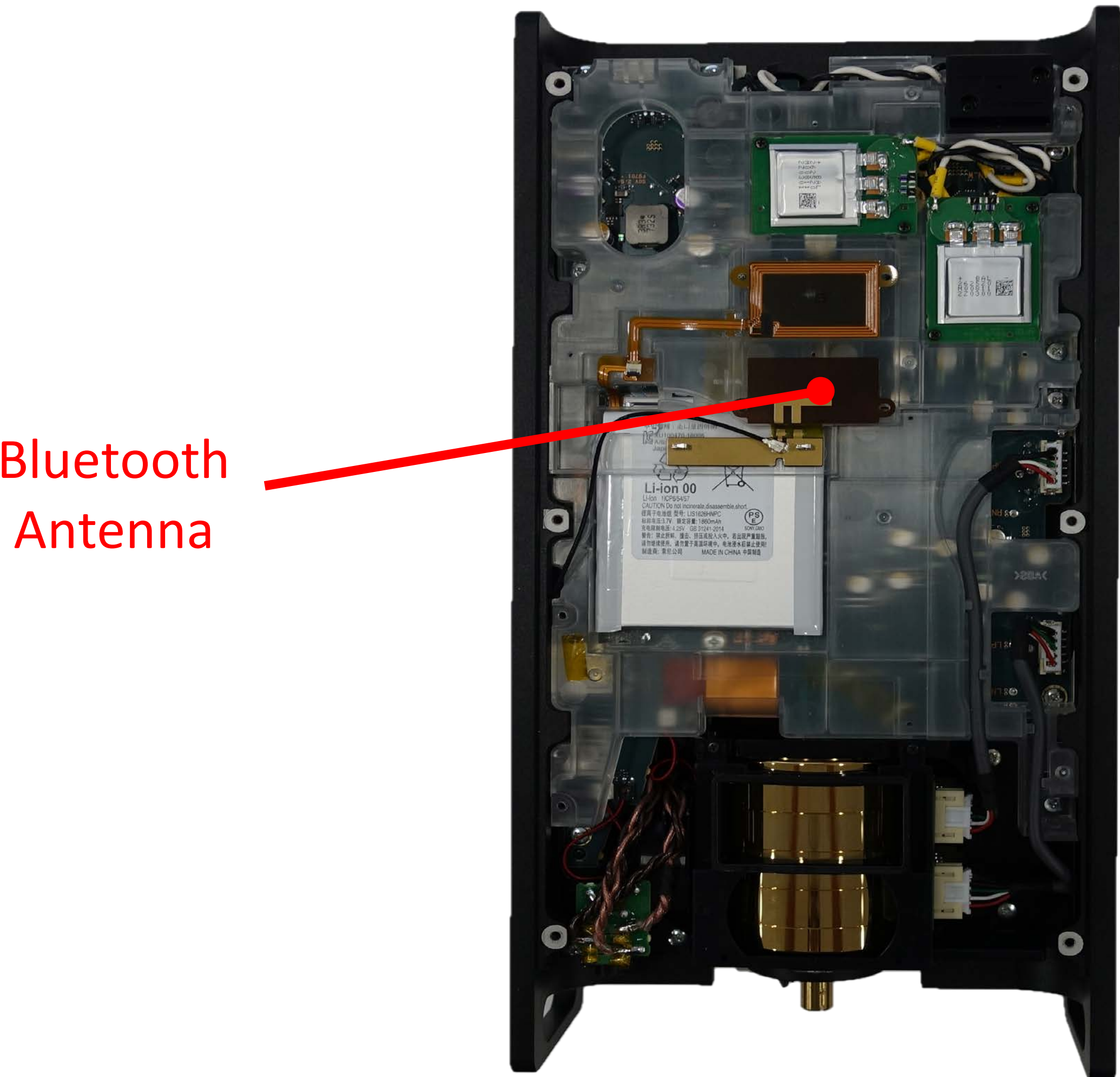
Top side of the product
