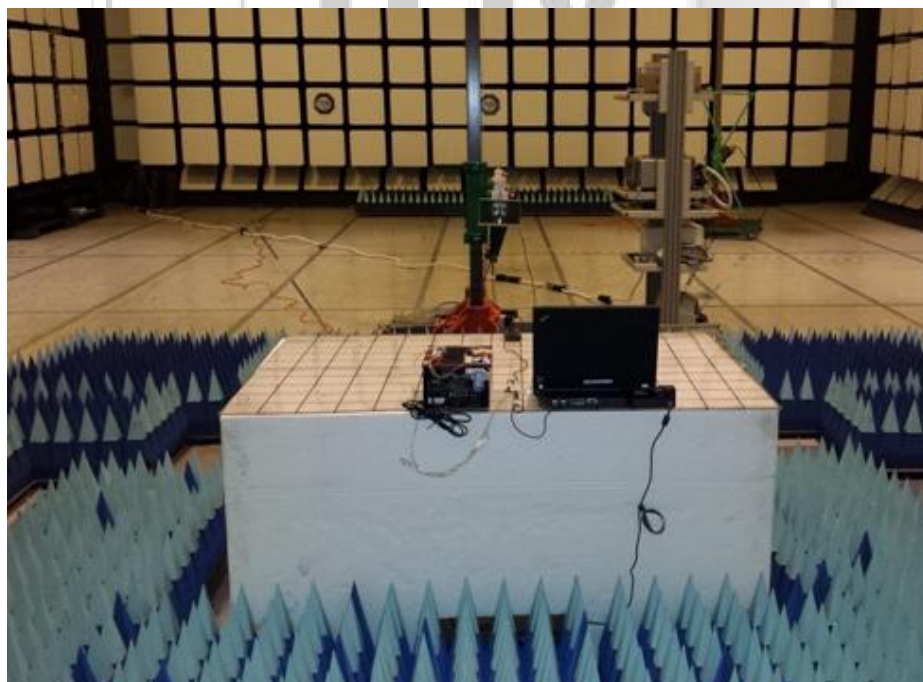
Radiated Emissions Test Setup (Rear View)
