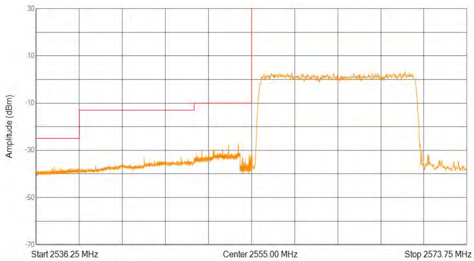
Band41(2555-2655) QAM16 BW=15MHz Channel=40315 RB Size=75 Position=#0
