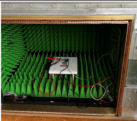
Photograph for Unwanted Emission into non-restricted frequency bands at the band edge
