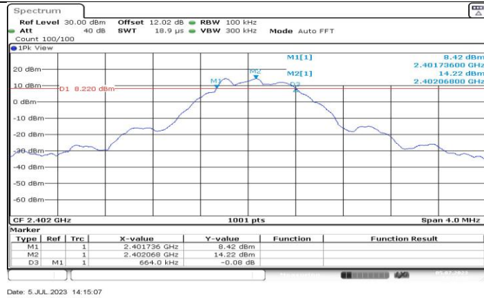
BLE_500K_Ant3_2402
