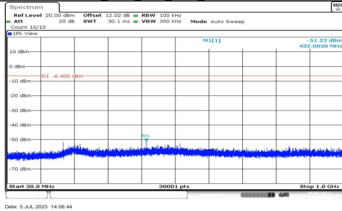
BLE_125K_Ant3_2402_30-1000
