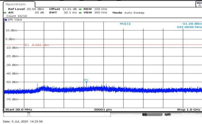
BLE_500K_Ant3_2480_30-1000
