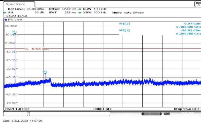
BLE_125K_Ant3_2402_1000-26500
