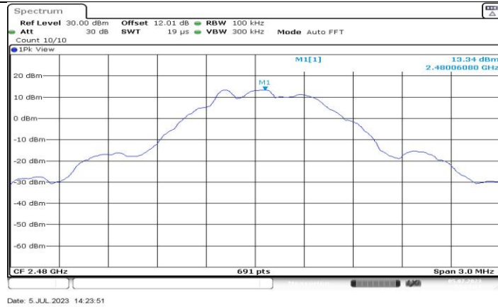
BLE_500K_Ant3_2480_0-Reference
