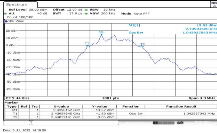
BLE_500K_Ant3_2440
