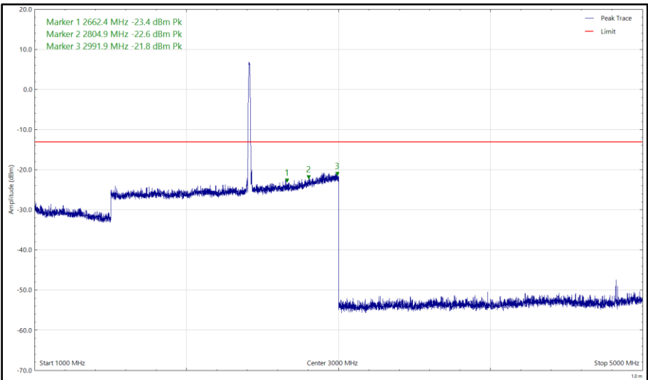
Figure 13 - LTE Cat NB B13_WIFI, 783_2412, 1 GHz to 5 GHz, Vertical (Peak)
