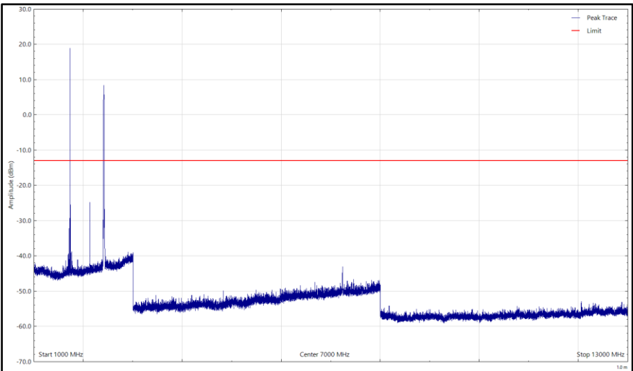
Figure 9 - LTE Cat M1 B4_WIFI, 1732.5_2412, 1 GHz to 13 GHz, Vertical (Peak)
