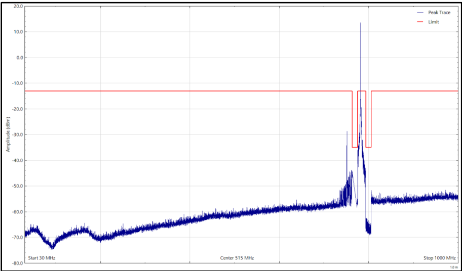
Figure 12 - LTE Cat NB B13_WIFI, 783_2412, 30 MHz to 1 GHz, Vertical (Peak)
