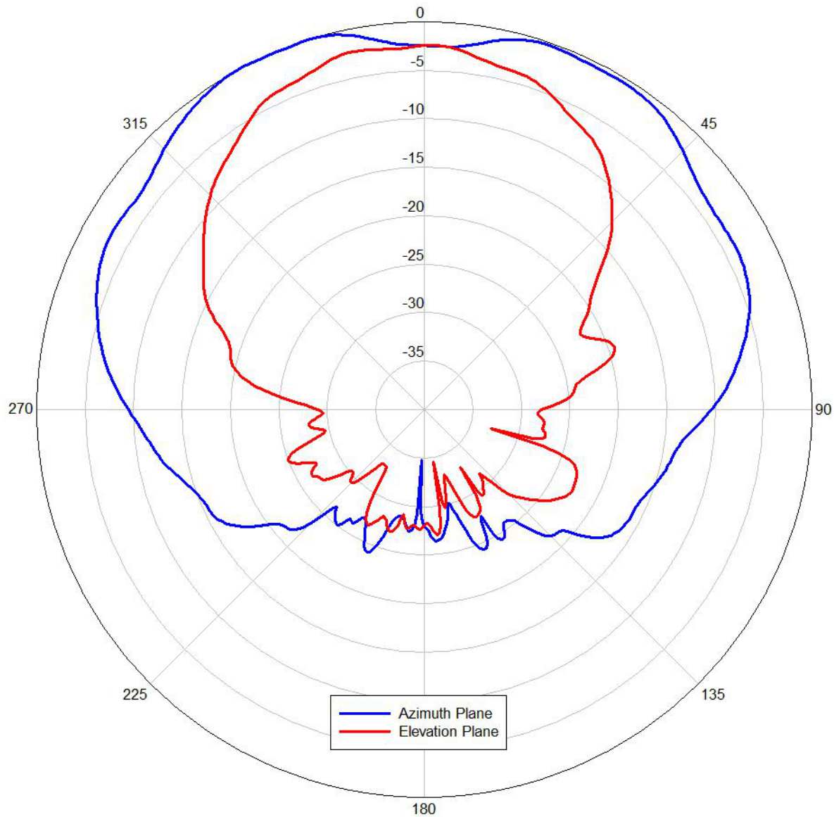
Figure 2 Azimuth and Elevation Radiation Patterns - 5 GHz Band
