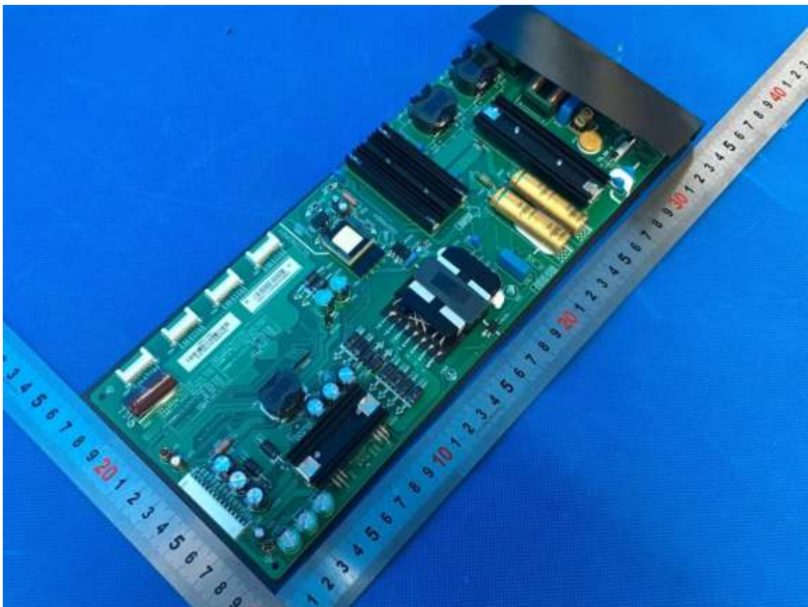
Picture 13 – Power board with mylar sheet view (Model FSP194-2FS01)
