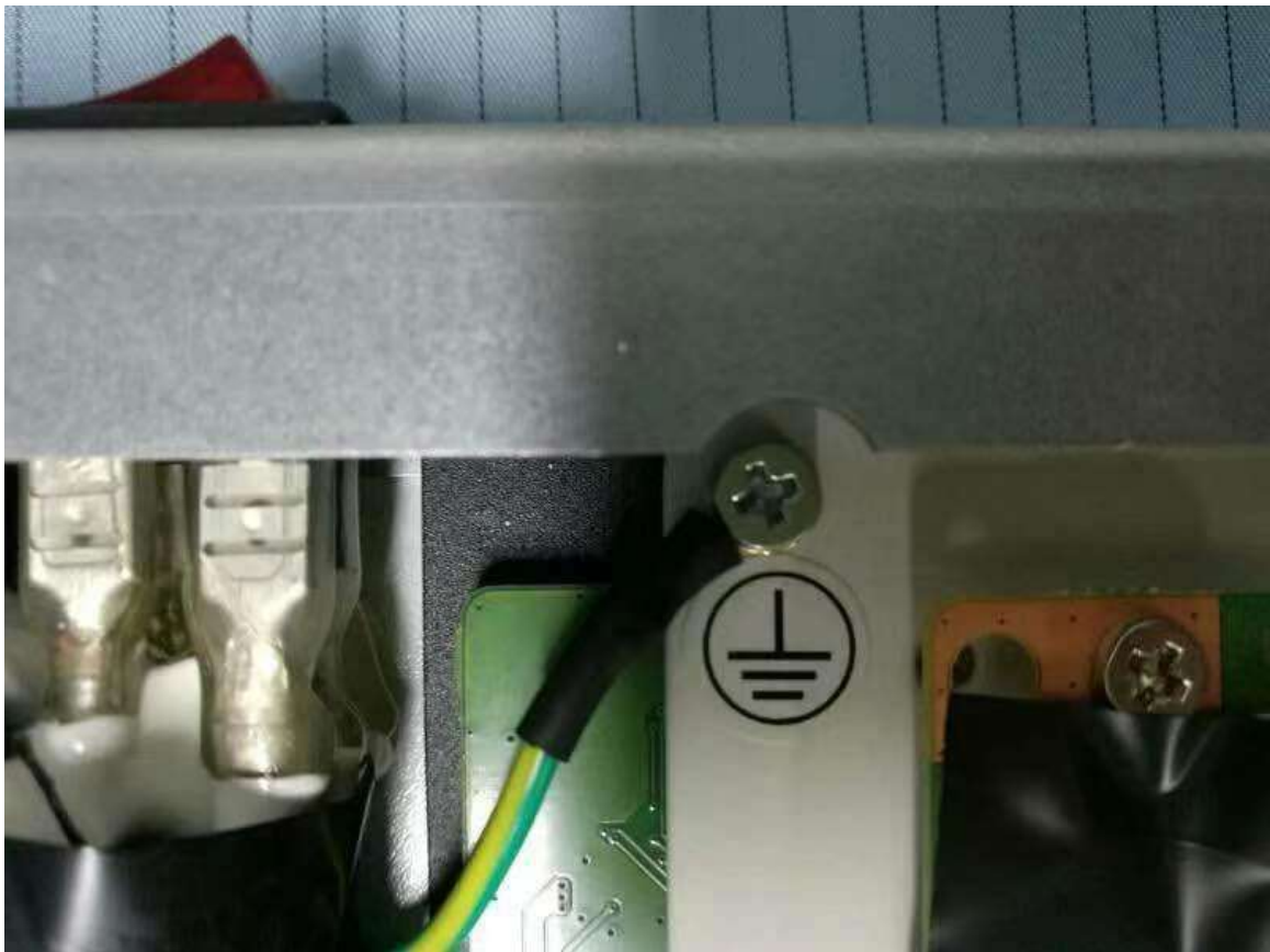
Picture 11 – Protective earth terminal
