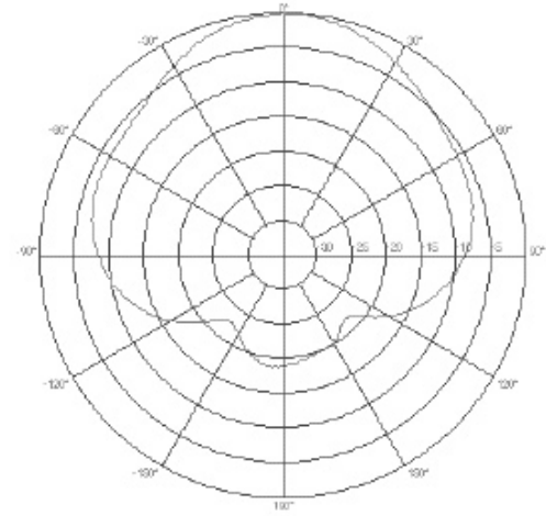
R380.900.909, 4.9 GHz, H-PLANE
