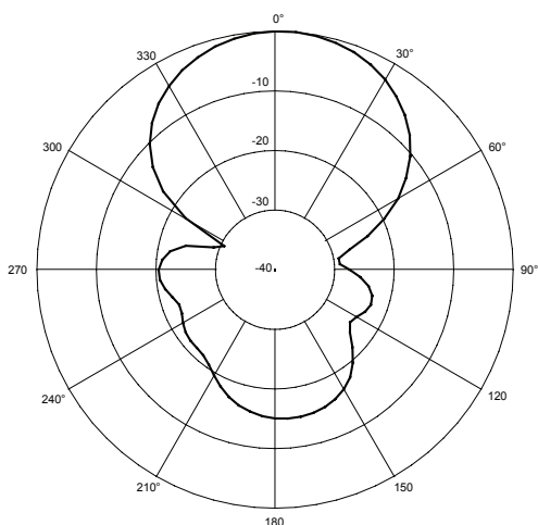
YA6 SERIES (740-960 MHz) E-PLANE
