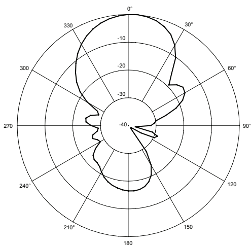
YA5 SERIES (740-960 MHz) E-PLANE
