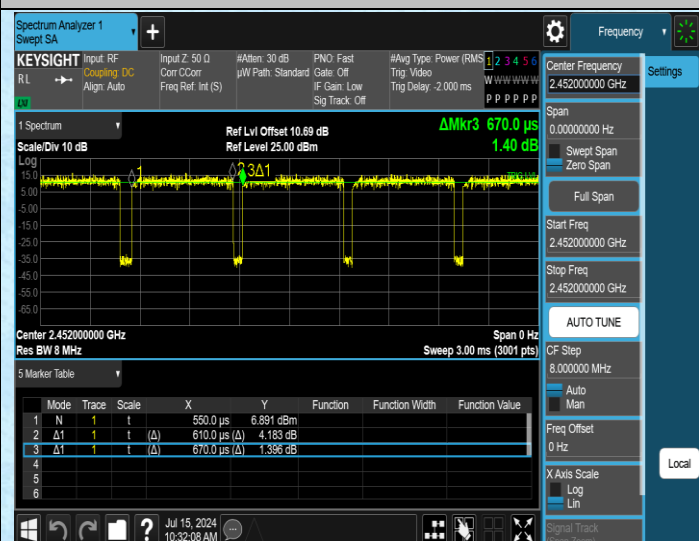
NTNV-11N40SISO-Ant1-2452
