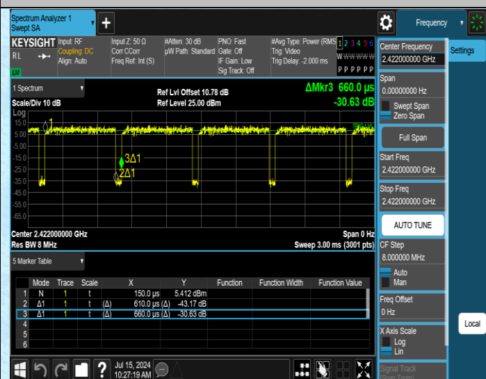
NTNV-11N40SISO-Ant1-2422
