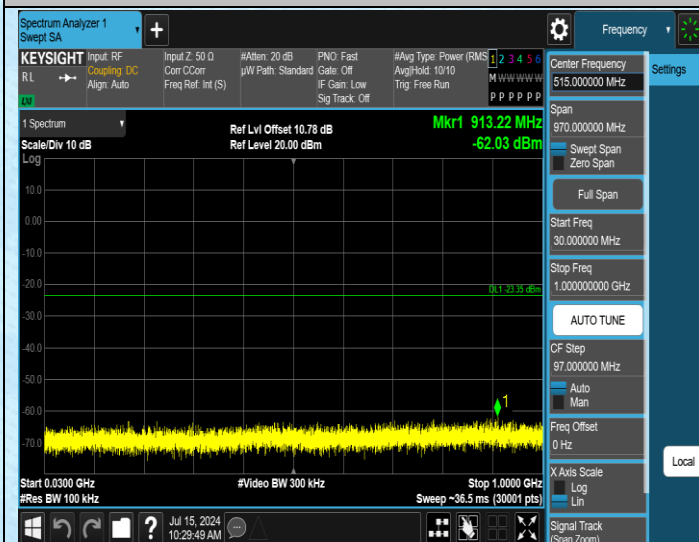
11N40SISO-Ant1-2422-30~1000-PASS
