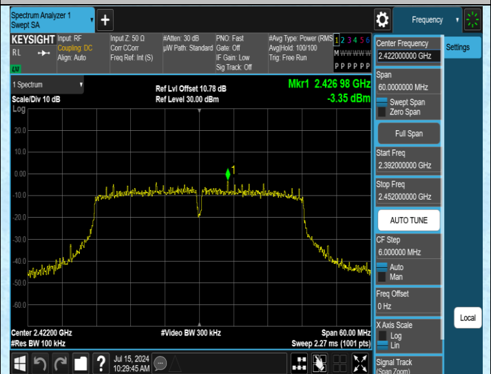
11N40SISO-Ant1-2422-0~Reference-PASS
