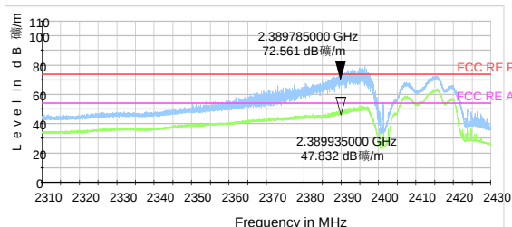
802.11g -Channel 1 Peak+ Average
