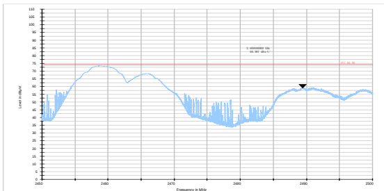
802.11b-Channel 11 Peak
