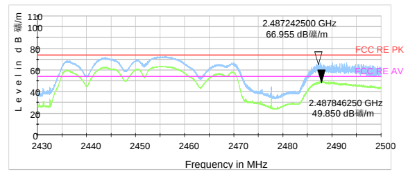
802.11n HT40 -Channel 9 Peak+ Average
