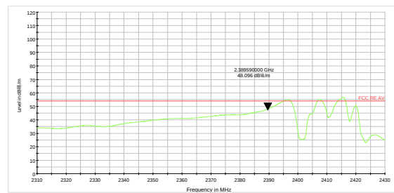
802.11g-Channel 1 Average
