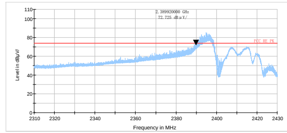
802.11g-Channel 1 Peak
