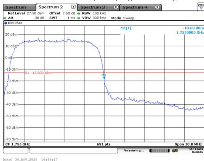
WCDMA Band IV,HSDPA,Right Band Edge
