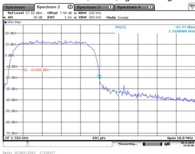
WCDMA Band IV, HSUPA, Right Band Edge
