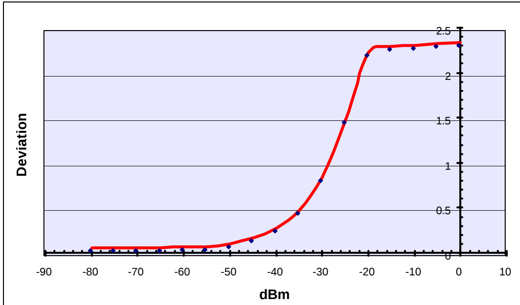
Modulation Limiting for 300Hz with 2.5kHz Dev.
