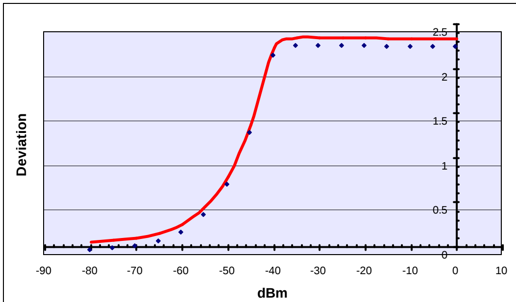
Modulation Limiting for 1000Hz with 2.5kHz Dev.
