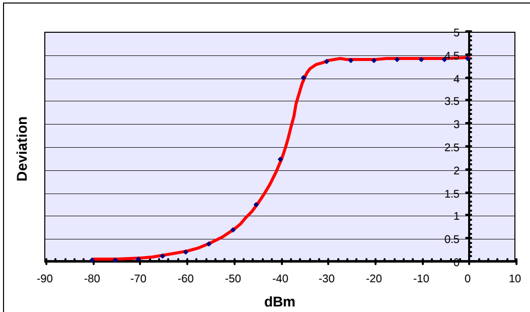
Modulation Limiting for 1000Hz with 5.0 kHz Dev.
