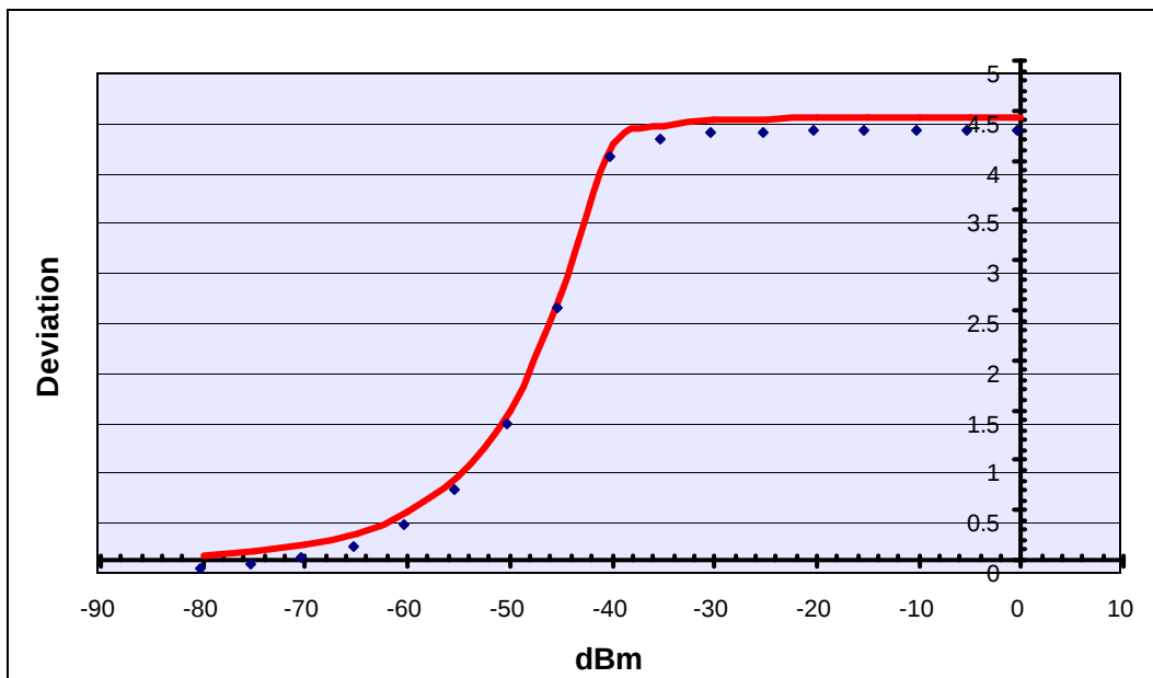
Modulation Limiting for 2500Hz with 5.0 kHz Dev.
