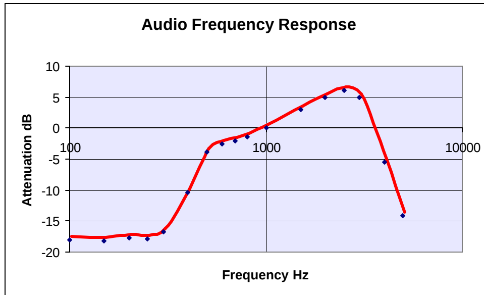
Audio Frequency Response with Narrow Band (2.5kHz)
