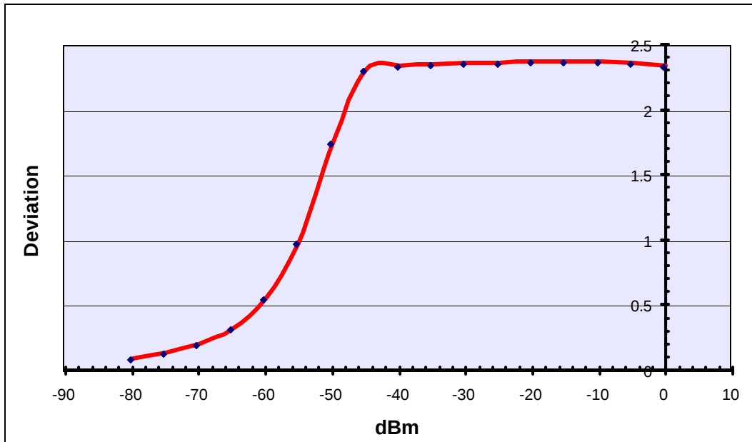
Modulation Limiting for 2500Hz with 2.5kHz Dev.
