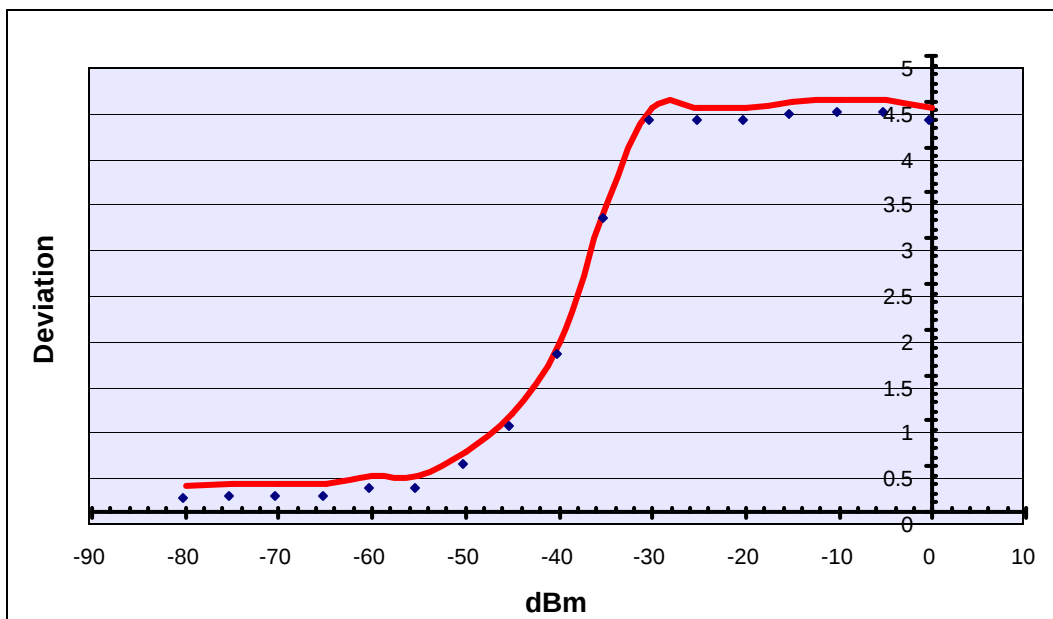
Modulation Limiting for 300Hz with 5.0kHz Dev.
