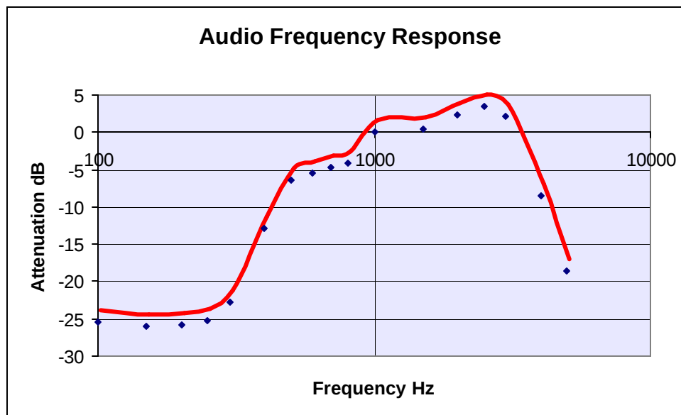
Audio Frequency Response with Wide Band (5.0kHz)
