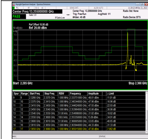
Band40_5MHz_64QAM_39225_1RB#0
