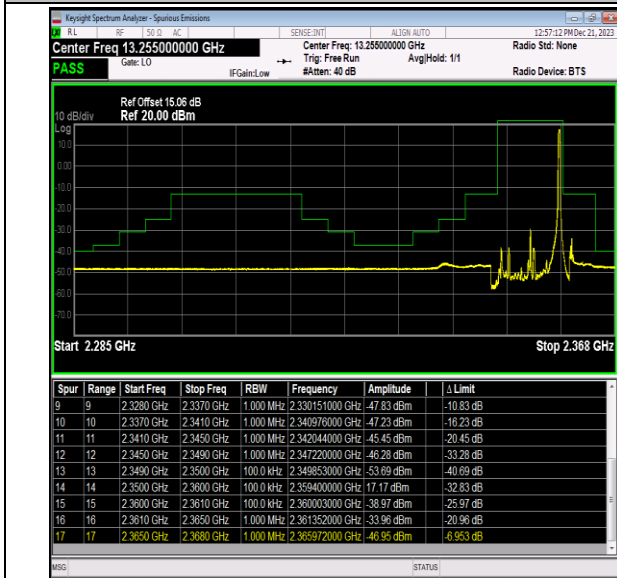
Band40_10MHz_QPSK_39200_1RB#49
