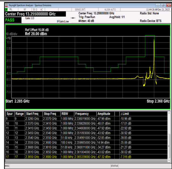
Band40_5MHz_64QAM_39225_1RB#24
