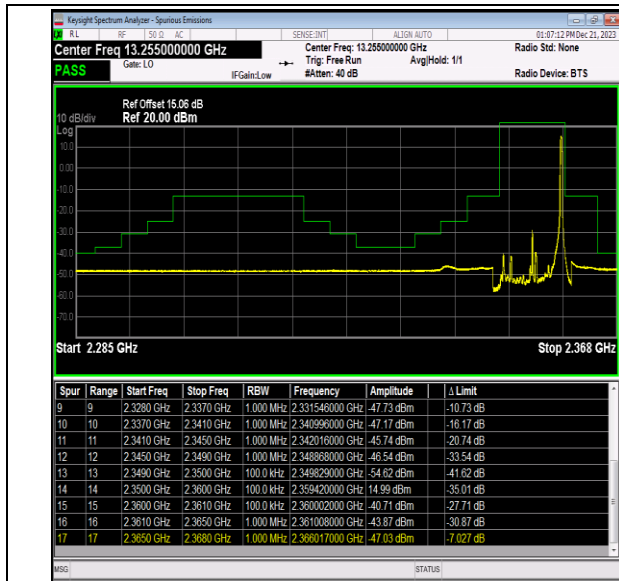
Band40_10MHz_64QAM_39200_1RB#49
