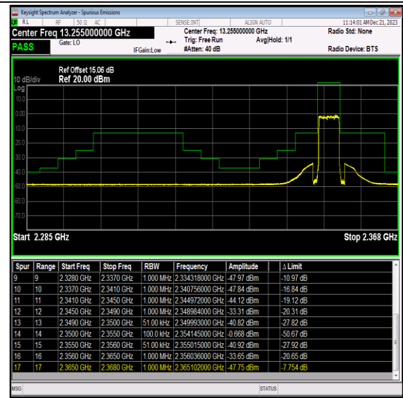
Band40_5MHz_64QAM_39175_25RB#0
