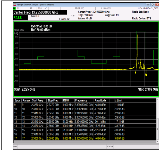
Band40_5MHz_16QAM_39225_1RB#0
