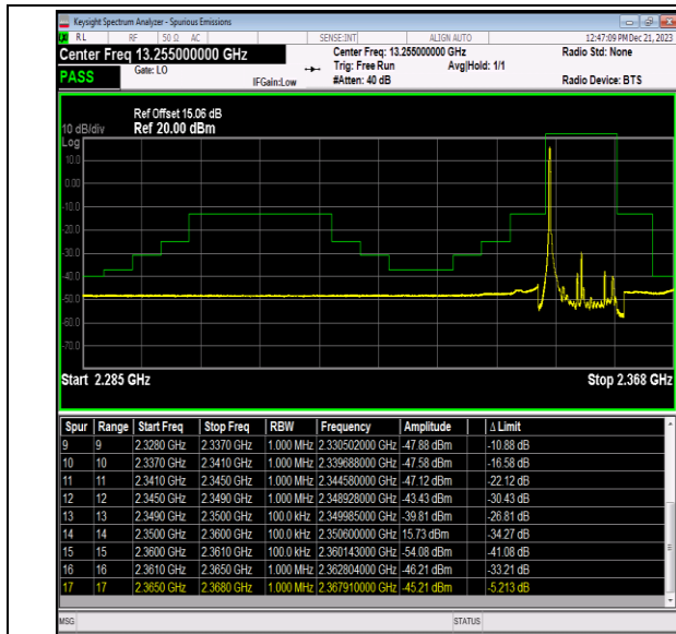
Band40_10MHz_16QAM_39200_1RB#0
