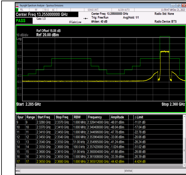
Band40_5MHz_64QAM_39225_25RB#0
