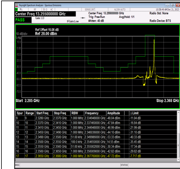
Band40_5MHz_64QAM_39175_1RB#24
