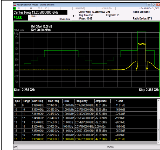
Band40_5MHz_16QAM_39225_25RB#0
