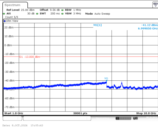
Band26-5MHz-QPSK-26740-1-0-Low-1000-10000--41.12-PASS
