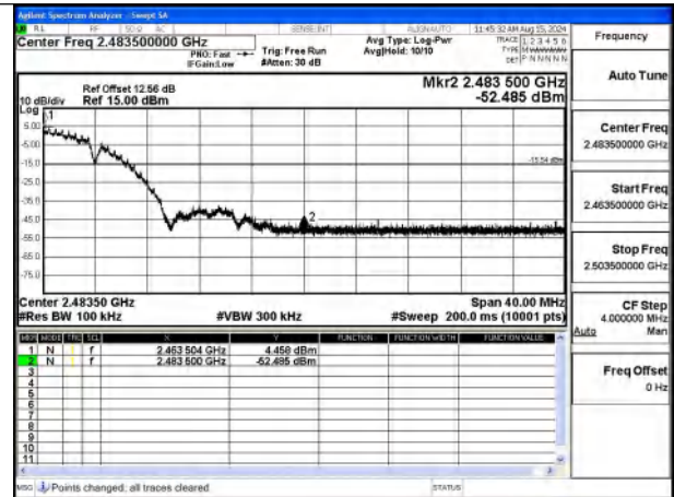
Mode:802.11b Frequency:2462MHz Ant:Chain0
