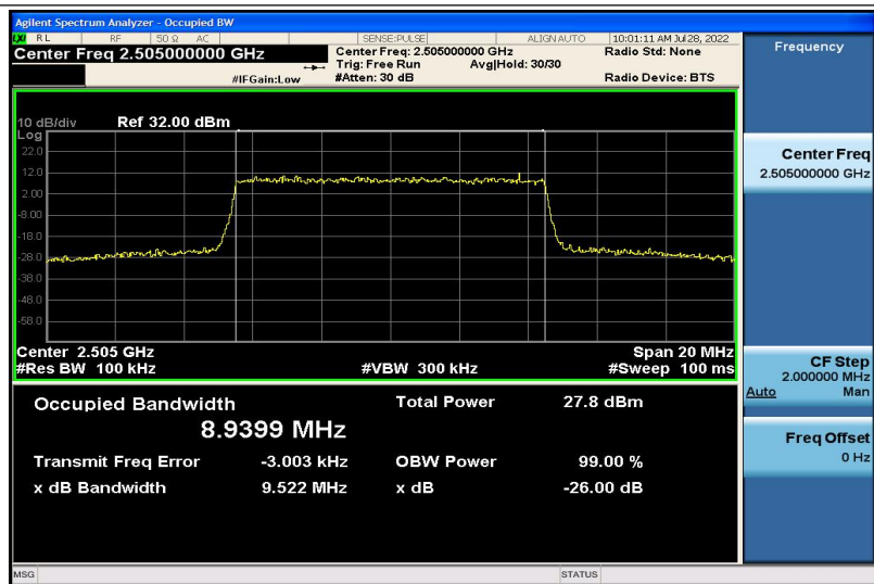
Band7-10MHz-16QAM-20800-50RB#0-8.9399
