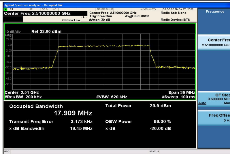
Band7-20MHz-16QAM-20850-100RB#0-17.909
