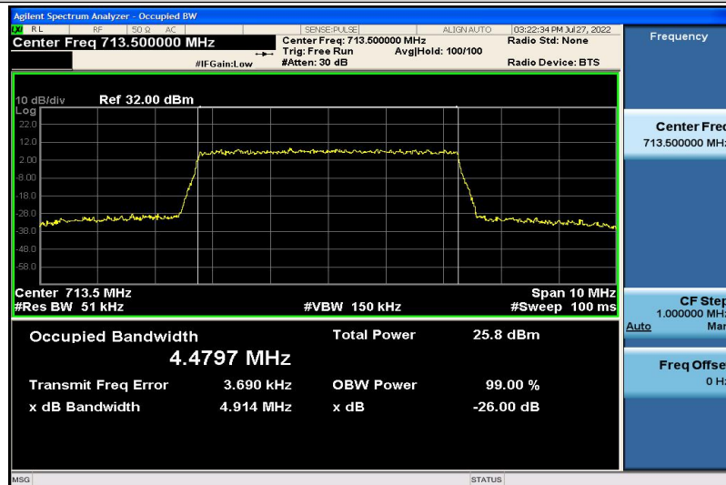
Band17-5MHz-16QAM-23825-25RB#0-4.4797
