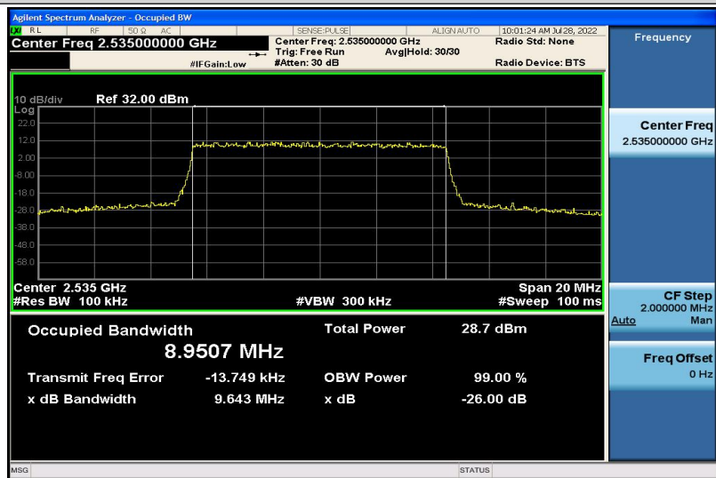
Band7-10MHz-QPSK-21100-50RB#0-8.9507
