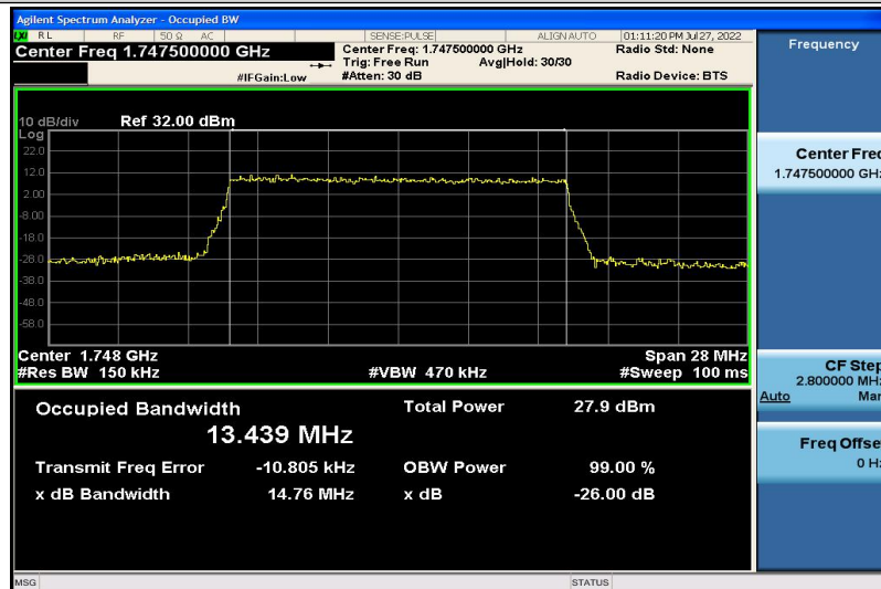
Band4-15MHz-16QAM-20325-75RB#0-13.439
