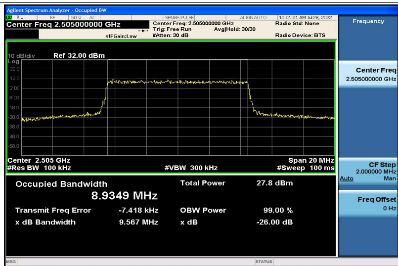
Band7-10MHz-QPSK-20800-50RB#0-8.9349
