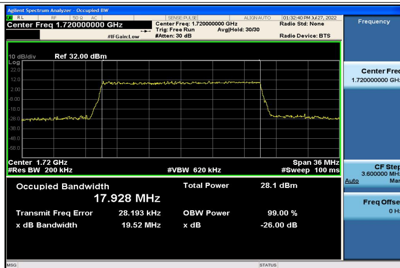
Band4-20MHz-16QAM-20050-100RB#0-17.928
