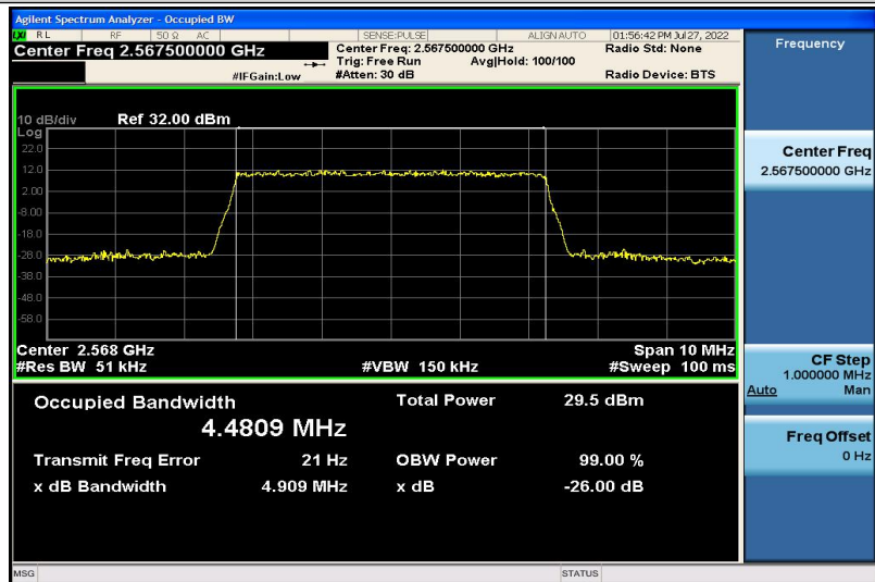
Band7-5MHz-QPSK-21425-25RB#0-4.4809
