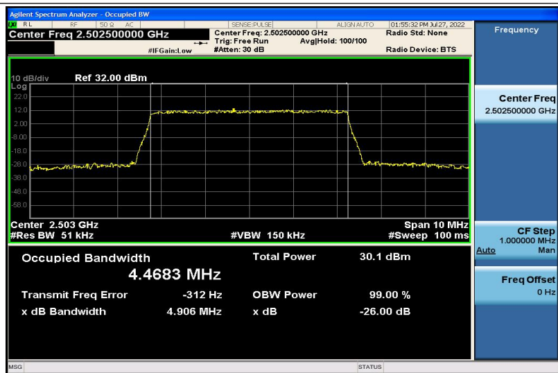
Band7-5MHz-QPSK-20775-25RB#0-4.4683
