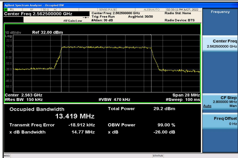
Band7-15MHz-16QAM-21375-75RB#0-13.419
