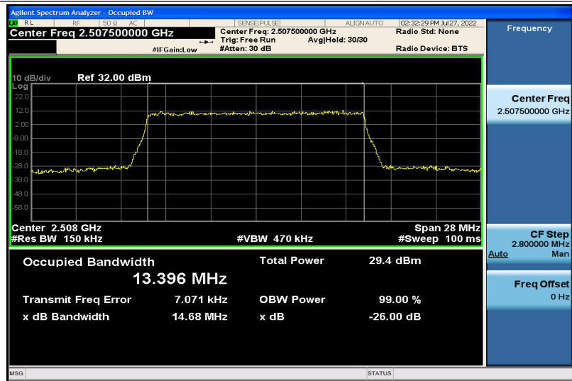
Band7-15MHz-16QAM-20825-75RB#0-13.396
