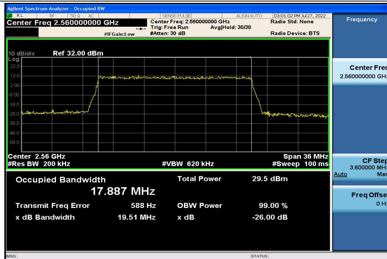
Band7-20MHz-16QAM-21350-100RB#0-17.887
