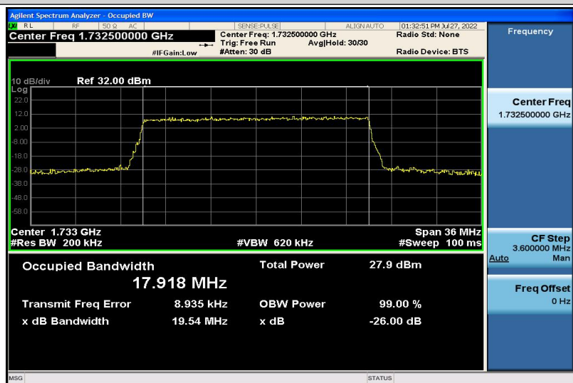
Band4-20MHz-QPSK-20175-100RB#0-17.918
