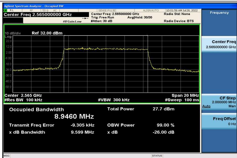
Band7-10MHz-16QAM-21400-50RB#0-8.9460
