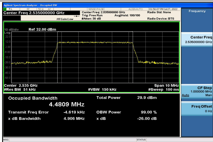
Band7-5MHz-QPSK-21100-25RB#0-4.4809
