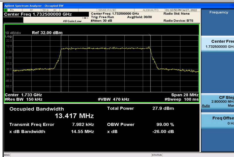
Band4-15MHz-QPSK-20175-75RB#0-13.417
