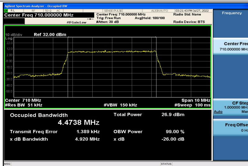
Band17-5MHz-QPSK-23790-25RB#0-4.4738
