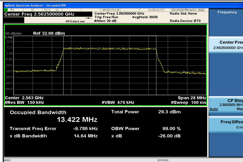
Band7-15MHz-QPSK-21375-75RB#0-13.422
