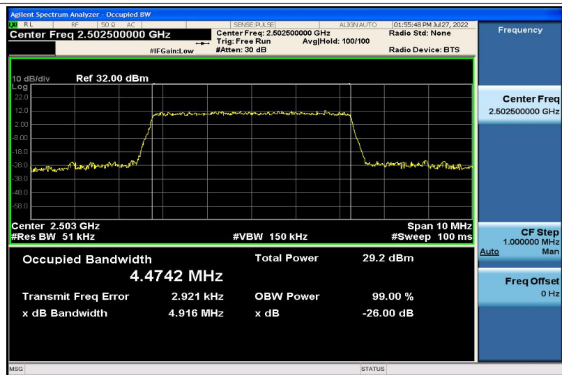
Band7-5MHz-16QAM-20775-25RB#0-4.4742
