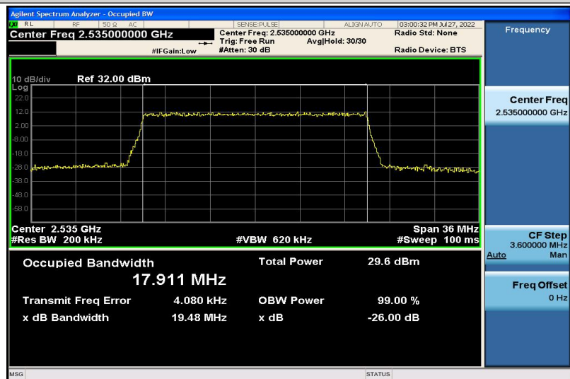
Band7-20MHz-QPSK-21100-100RB#0-17.911
