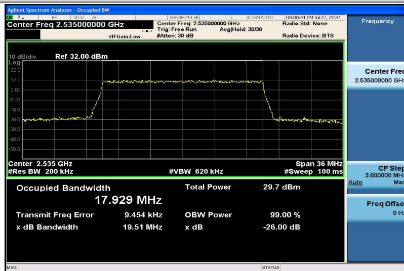
Band7-20MHz-16QAM-21100-100RB#0-17.929
