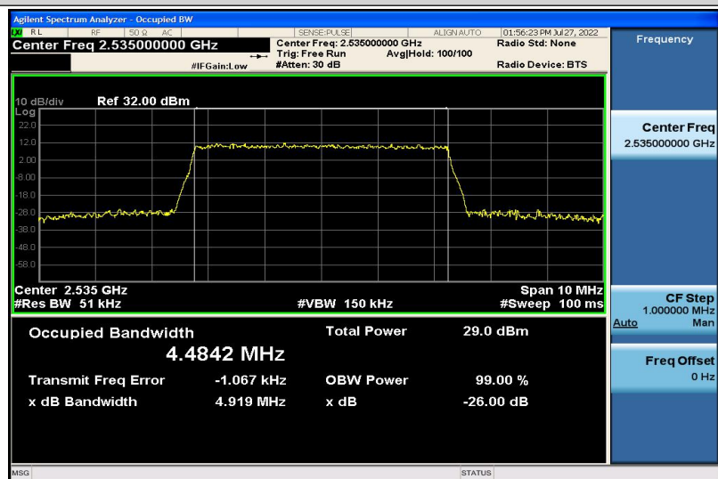
Band7-5MHz-16QAM-21100-25RB#0-4.4842
