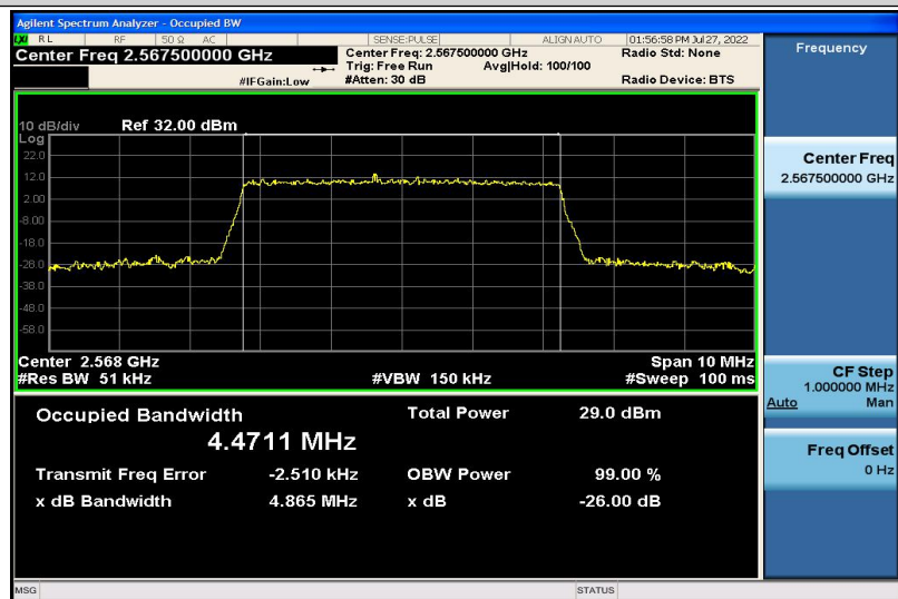
Band7-5MHz-16QAM-21425-25RB#0-4.4711
