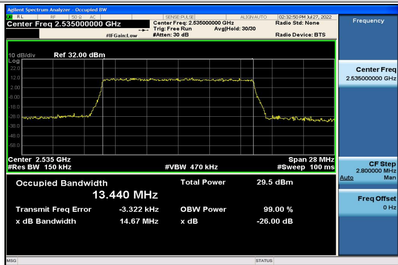
Band7-15MHz-16QAM-21100-75RB#0-13.440
