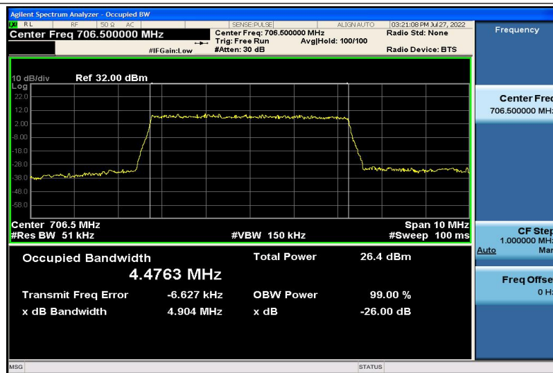
Band17-5MHz-QPSK-23755-25RB#0-4.4763
