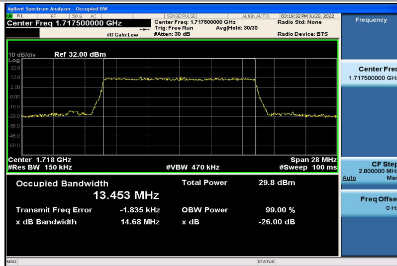
Band4-15MHz-QPSK-20025-75RB#0-13.453
