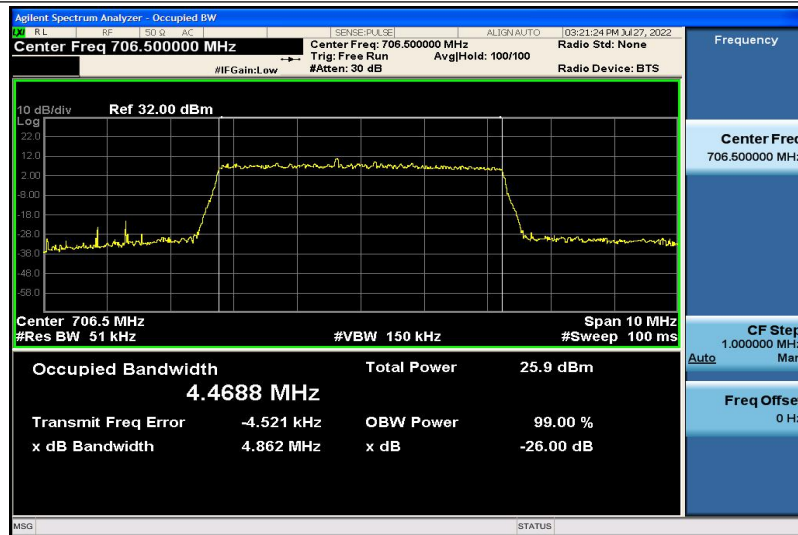
Band17-5MHz-16QAM-23755-25RB#0-4.4688
