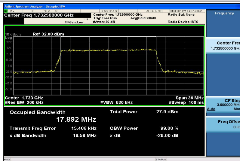
Band4-20MHz-16QAM-20175-100RB#0-17.892
