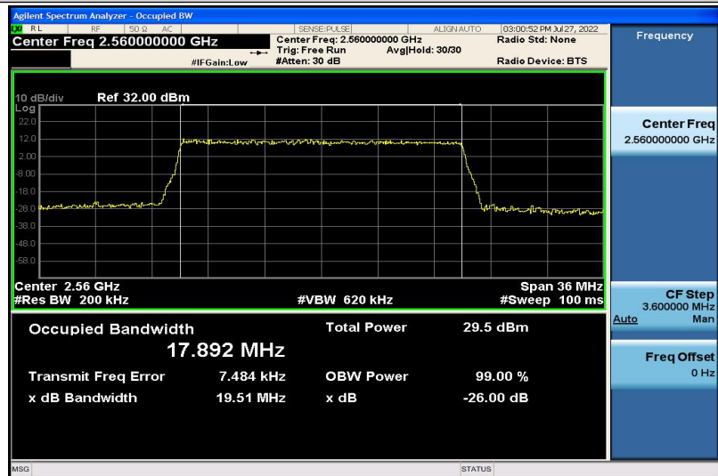
Band7-20MHz-QPSK-21350-100RB#0-17.892
