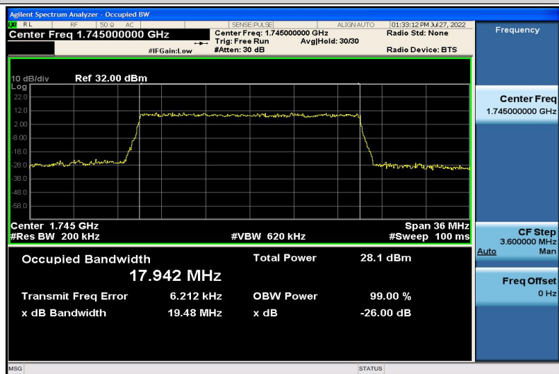
Band4-20MHz-QPSK-20300-100RB#0-17.942
