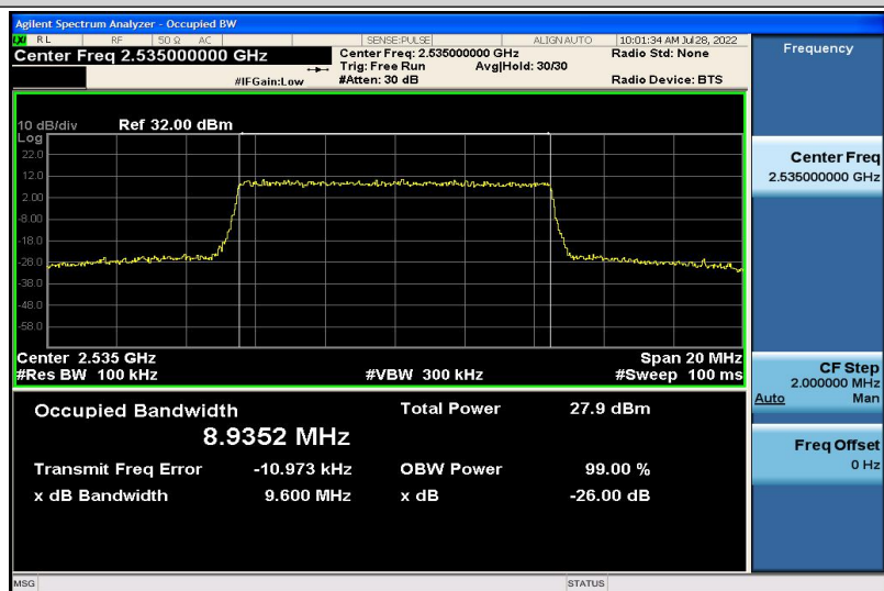
Band7-10MHz-16QAM-21100-50RB#0-8.9352
