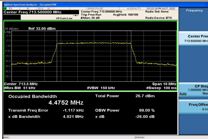
Band17-5MHz-QPSK-23825-25RB#0-4.4752
