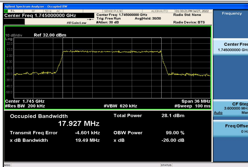
Band4-20MHz-16QAM-20300-100RB#0-17.927
