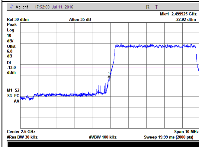
LTE Band 7 - Low Channel 16QAM-5
