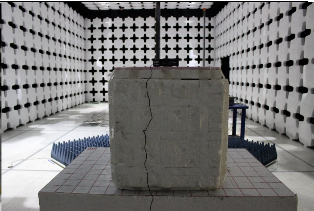
Spurious Emission Above 1GHz-Rear View
