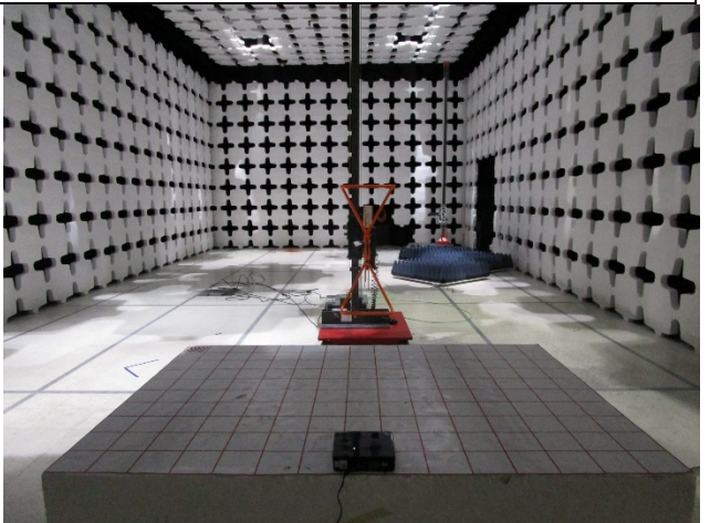
Spurious Emission Below 1GHz-Rear View
