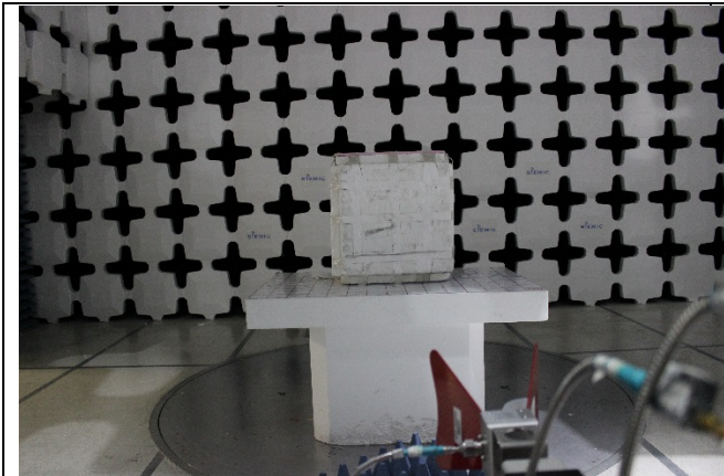
Spurious Emission Above 1GHz-Front View
