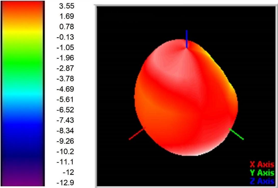
3D Radiation Patterns @2460MHz (Unit:dBi)
