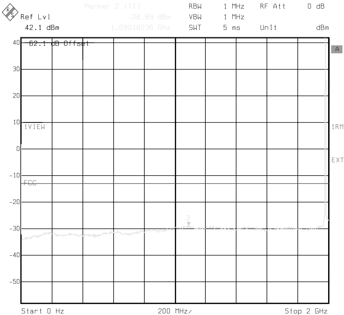
Figure 19 : Conducted Spurious Emissions - 3 Carrier, Channels 925, 950, 975 (10 kHz - 2 GHz)
