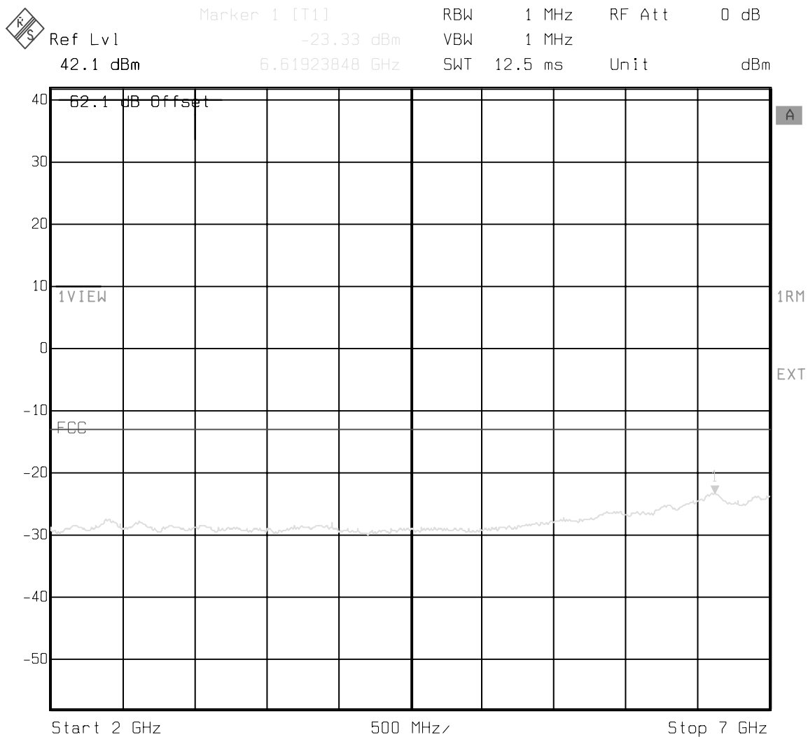
Figure 20 : Conducted Spurious Emissions - 3 Carrier, Channels 925, 950, 975 (2 GHz - 7 GHz)
