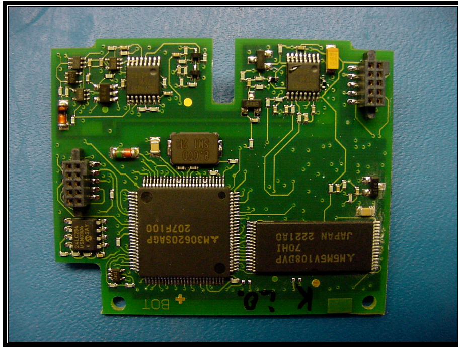
Photograph 55: Module Parts PCB2 Top View
