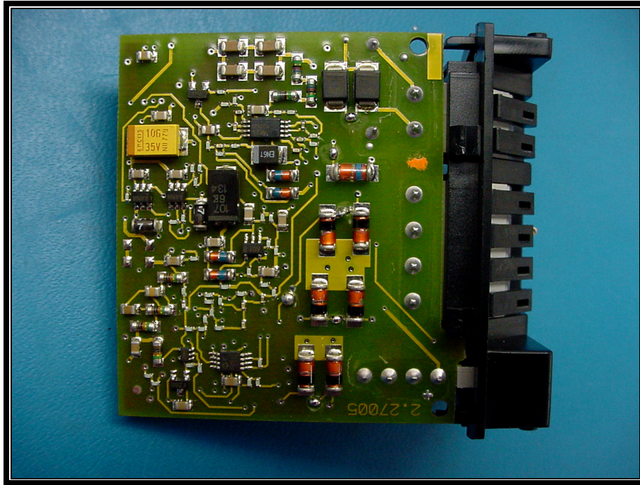
Photograph 54: Module Parts PCB1 Bottom View
