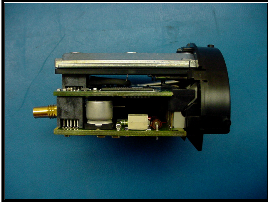
Photograph 52: EUT Module Parts Side View
