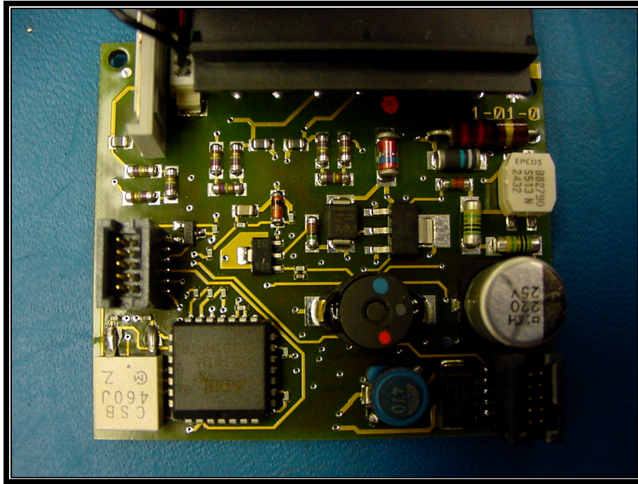
Photograph 53: Module Parts PCB1 Top View
