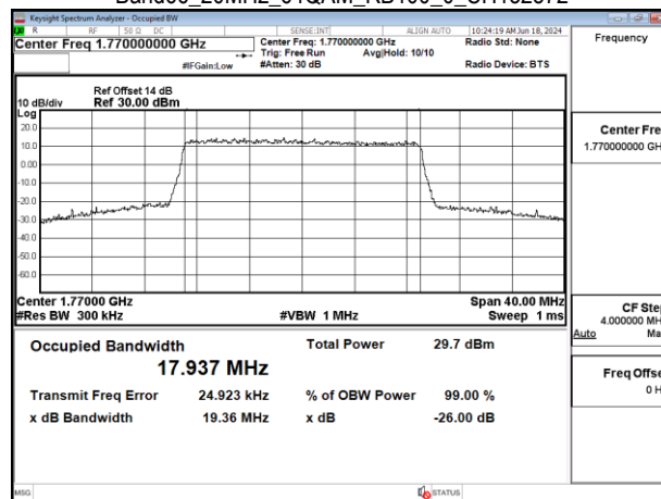
Band66 20MHz_64QAM_RB100_0_CH132572
