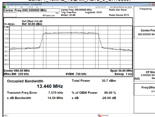
Band71_15MHz_16QAM_RB75_0_CH133397
