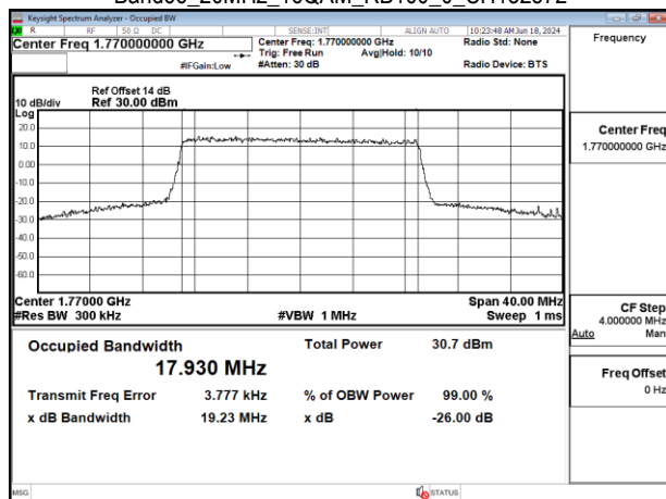
Band66 20MHz_16QAM_RB100_0_CH132572
