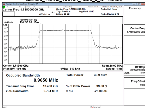
Band66_10MHz_16QAM_RB50_0_CH132322
