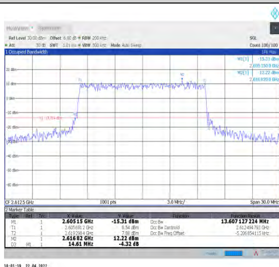
1-N38--30-15-H-6-CP-QPSK-Outer_Full-38@0-Ant1- 13.607-14.610-≤15-PASS
