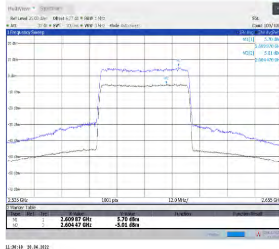
1-N38--30-40-M-2-CP-256QAM-Outer_Full-106@0-A Ant1-10.71-19.4%-7.12-3.59-PASS-≤13
