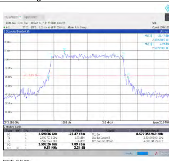
1-N38--30-10-M-9-CP-256QAM-Outer_Full-24@0-A nt1-8.577-9.540-≤10-PASS
