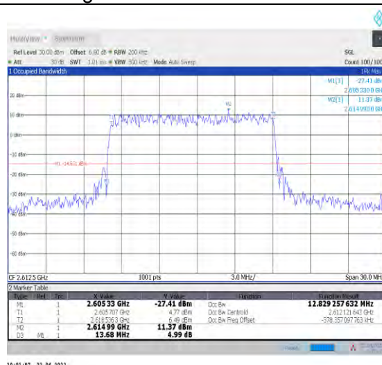
1-N38--30-15-H-5-DFT-256QAM-Outer_Full-36@0-A nt1-12.829-13.680-≤15-PASS
