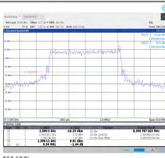
1-N38--30-10-M-7-CP-16QAM-Outer_Full-24@0-Ant 1-8.6-9.540-≤10-PASS
