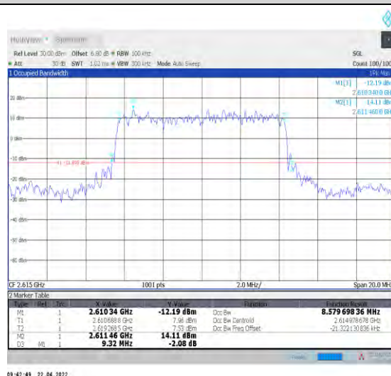
1-N38--30-10-H-2-DFT-PI2BPSK-Outer_Full-24@0-A Ant1-8.58-9.320-≤10-PASS
