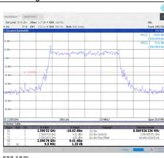
1-N38--30-10-M-5-DFT-256QAM-Outer_Full-24@0- Ant1-8.57-9.500-≤10-PASS
