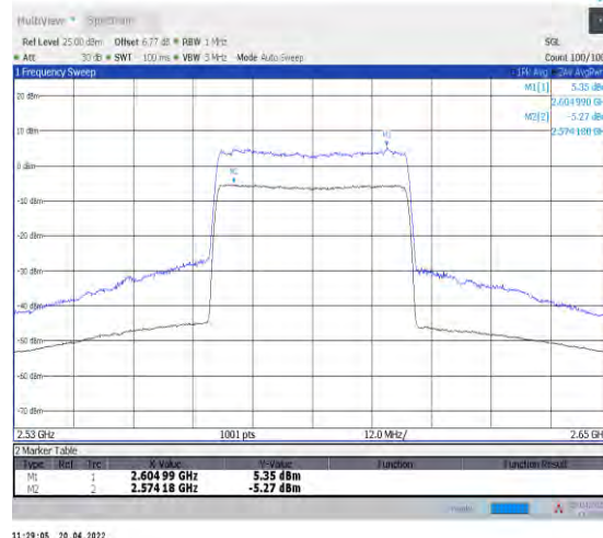
1-N38--30-40-L-2-CP-256QAM-Outer_Full-106@0-A Ant1-10.62-19.4%-7.12-3.50-PASS-≤13
