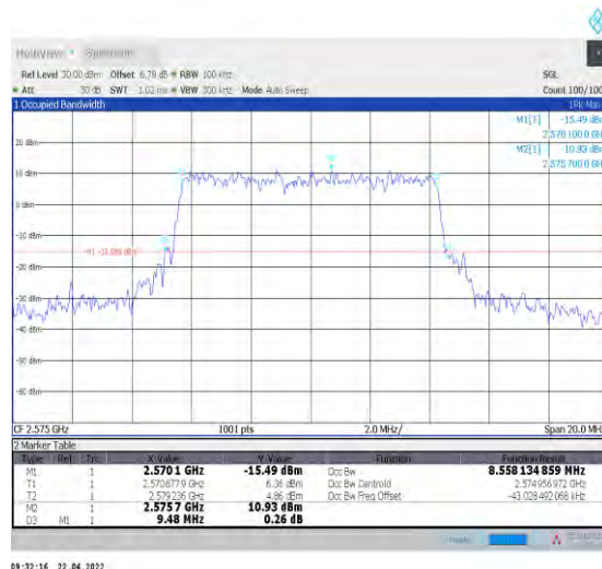
1-N38--30-10-L-4-DFT-64QAM-Outet_Full-24@0-Ant1 t1-8.558-9.480-≤10-PASS
