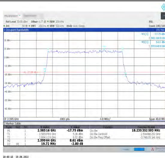
1-N38--30-20-M-9-CP-256QAM-Outer_Full-51@0-A nt1-18.235-19.720-≤20-PASS
