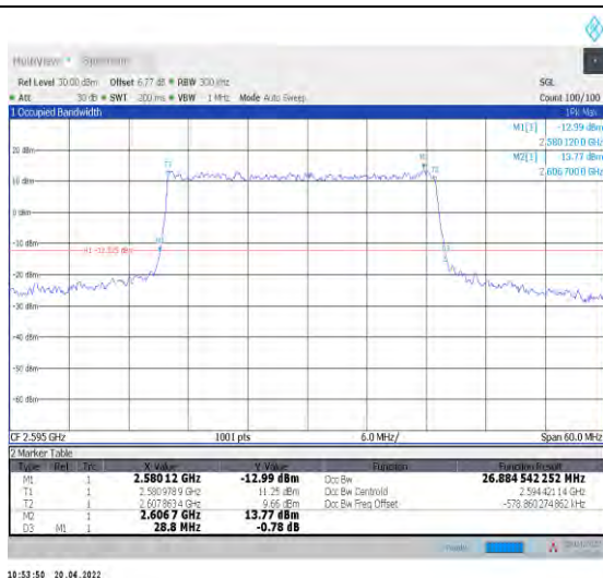
1-N38--30-30-M-3-DFT-16QAM-Outer_Full-75@0-An t1-26.885-28.800-≤30-PASS
