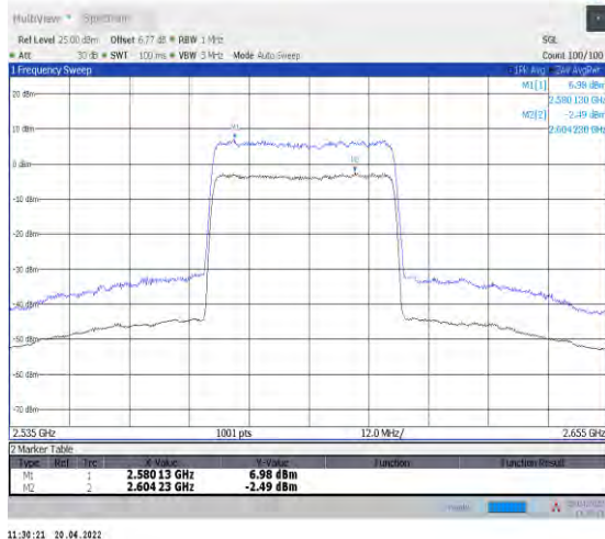
1-N38--30-40-M-1-DFT-256QAM-Outer_Full-100@0-A Ant1-9.47-19.4%-7.12-2.35-PASS-≤13
