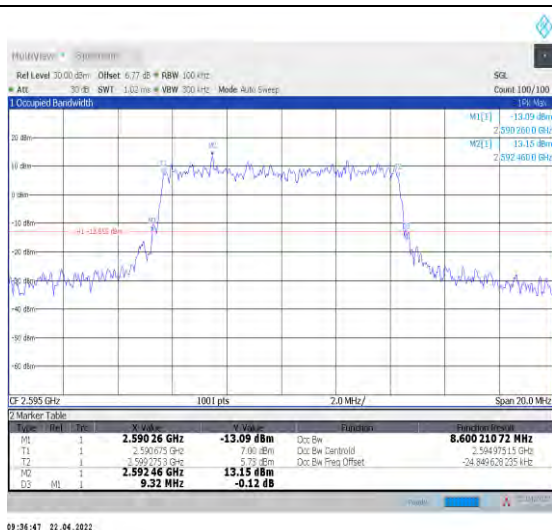
1-N38--30-10-M-4-DFT-64QAM-Outer_Full-24@0-An t1-8.6-9.320-≤10-PASS
