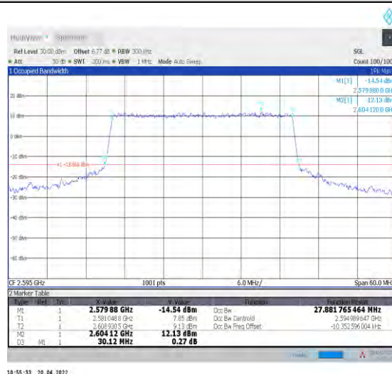
1-N38--30-30-M-6-CP-QPSK-Outer_Full-78@0-Ant1 -27.882-30.120-≤30-PASS
