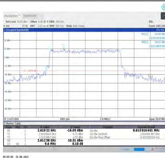
1-N38--30-10-H-6-CP-QPSK-Outer_Full-24@0-Ant1- 8.615-9.600-≤10-PASS
