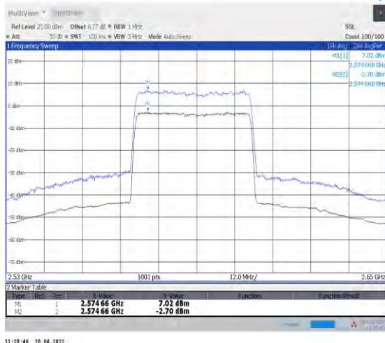
1-N38--30-40-L-1-DFT-256QAM-Outer_Full-100@0-A Ant1-9.72-19.4%-7.12-2.60-PASS-≤13
