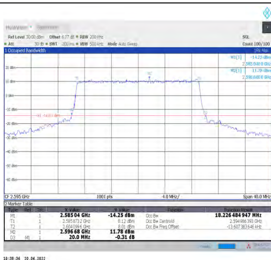
1-N38--30-20-M-6-CP-QPSK-Outer_Full-51@0-Ant1- 18.226-20.000-≤20-PASS
