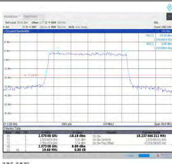
1-N38--30-20-L-9-CP-256QAM-Outer_Full-51@0-Ant 1-18.237-19.680-≤20-PASS
