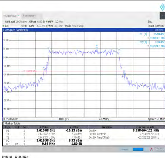
1-N38--30-10-H-5-DFT-256QAM-Outer_Full-24@0-A nt1-8.559-9.860-≤10-PASS
