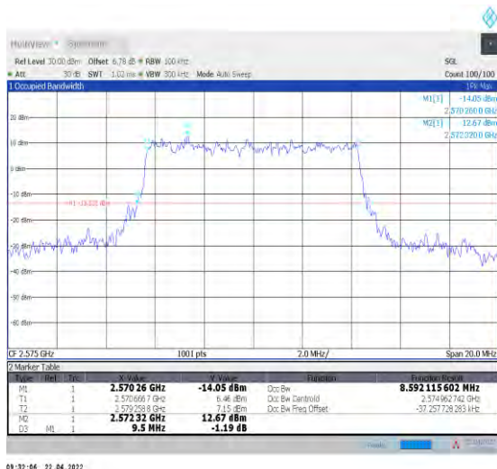
1-N38--30-10-L-3-DFT-16QAM-Outet_Full-24@0-Ant1 1-8.592-9.500-≤10-PASS
