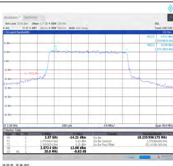
1-N38--30-20-L-7-CP-16QAM-Outer_Full-51@0-Ant1 -18.236-20.000-≤20-PASS
