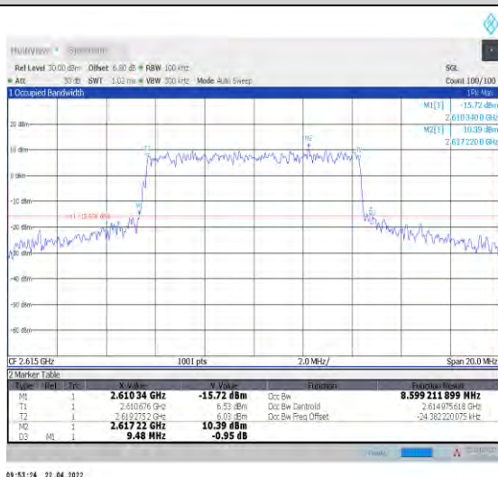
1-N38--30-10-H-1-DFT-QPSK-Outer_Full-24@0-Ant 1-8.599-9.480-≤10-PASS
