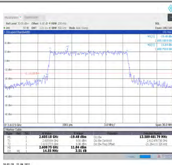
1-N38--30-15-H-7-CP-16QAM-Outer_Full-38@0-Ant 1-13.589-14.550-≤15-PASS
