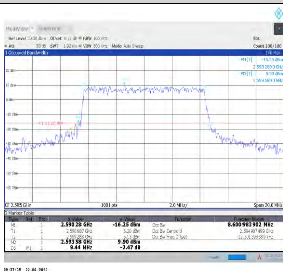
1-N38--30-10-M-6-CP-QPSK-Outer_Full-24@0-Ant1- 8.601-9.440-≤10-PASS
