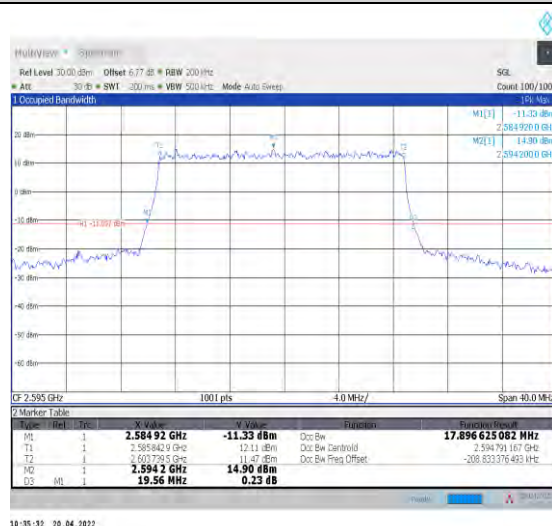
1-N38--30-20-M-1-DFT-QPSK-Outer_Full-50@0-Ant 1-17.897-19.560-≤20-PASS
