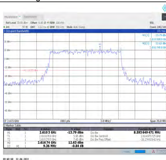
1-N38--30-10-H-4-DFT-64QAM-Outer_Full-24@0-An t1-8.594-9.360-≤10-PASS
