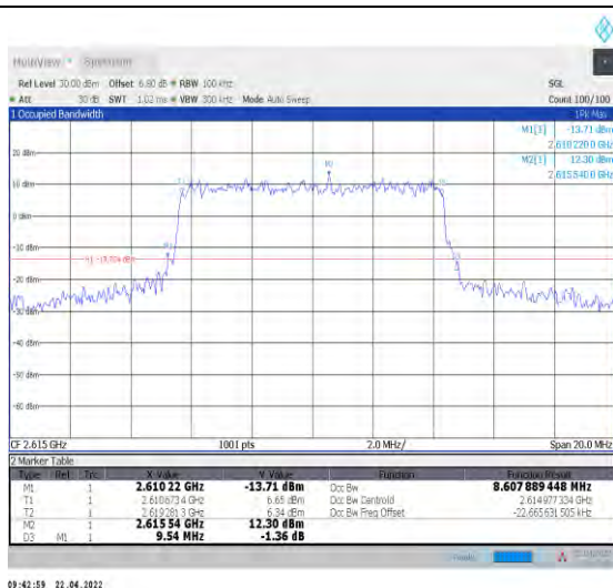
1-N38--30-10-H-3-DFT-16QAM-Outer_Full-24@0-An t1-8.608-9.540-≤10-PASS
