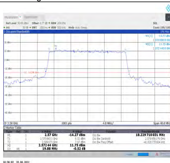
1-N38--30-20-L-8-CP-64QAM-Outer_Full-51@0-Ant 1-18.23-19.880-≤20-PASS
