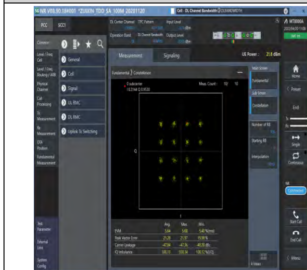
1-N38--30-40-M-7-CP-16QAM-Outer_Full-106@0-Ant1-see graph-PASS
