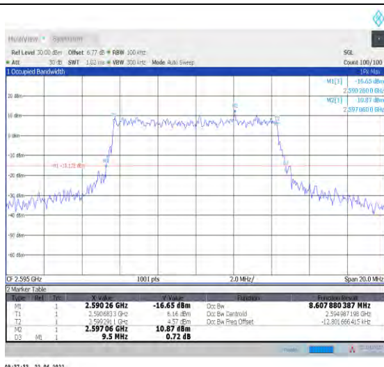
1-N38--30-10-M-8-CP-64QAM-Outer_Full-24@0-Ant 1-8.608-9.500-≤10-PASS
