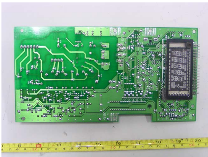
Internal photo-PCB View (2)
