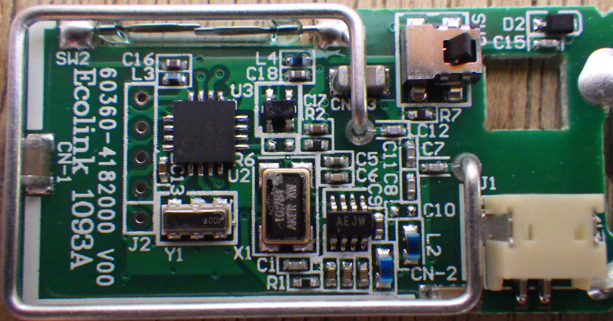
Top View of the PCB - NO Sticker - View #3
