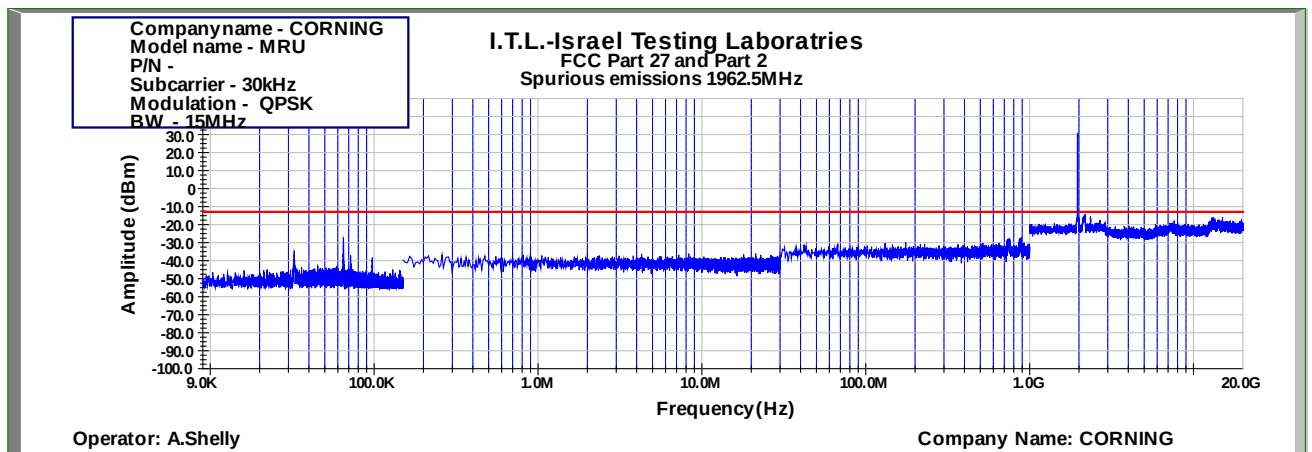
Figure 1018: Spurious Emissions at Antenna Terminal QPSK 15MHz B.W.; 1962.5MHz, 30kHz
