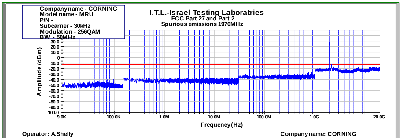
Figure 991: Spurious Emissions at Antenna Terminal 256QAM 50MHz B.W.; 1970.0MHz, 30kHz
