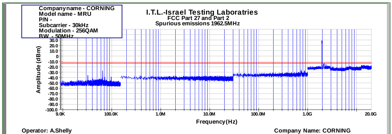
Figure 988: Spurious Emissions at Antenna Terminal 256QAM 50MHz B.W.; 1962.5MHz, 30kHz
