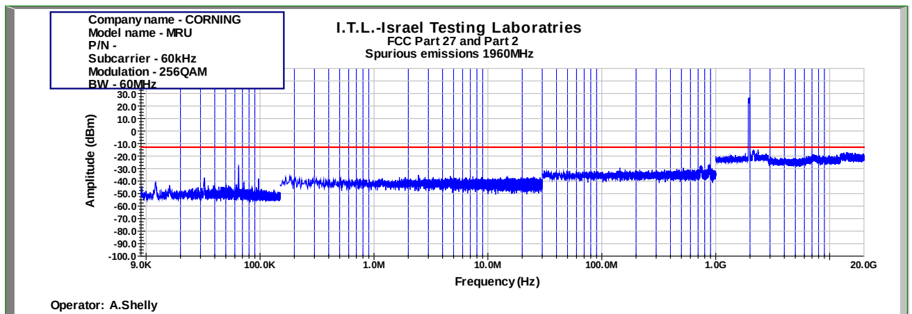
Figure 994: Spurious Emissions at Antenna Terminal 256QAM 60MHz B.W.; 1960.0MHz, 60kHz
