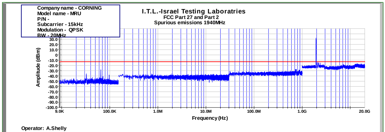
Figure 1023: Spurious Emissions at Antenna Terminal QPSK 20MHz B.W.; 1940.0MHz, 15kHz
