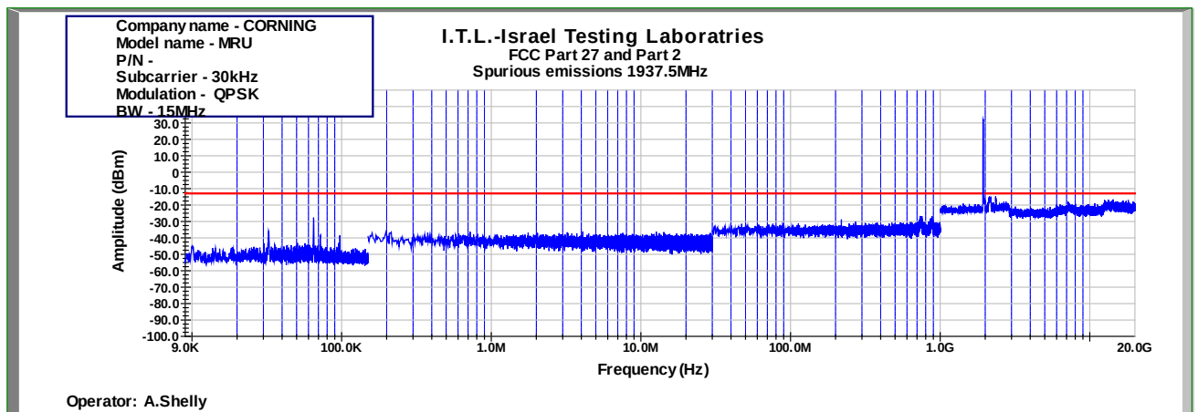
Figure 1015: Spurious Emissions at Antenna Terminal QPSK 15MHz B.W.; 1937.5MHz, 30kHz
