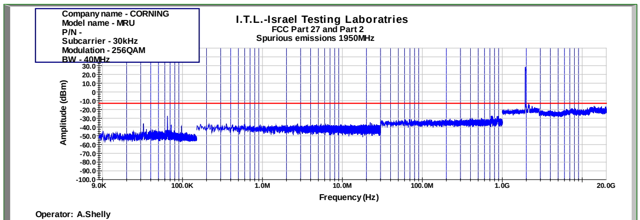
Figure 976: Spurious Emissions at Antenna Terminal 256QAM 40MHz B.W.; 1950.0MHz, 30kHz
