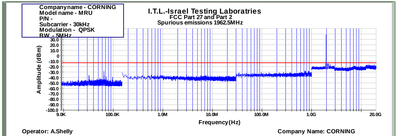
Figure 1002: Spurious Emissions at Antenna Terminal QPSK 5MHz B.W.; 1962.5MHz, 30kHz
