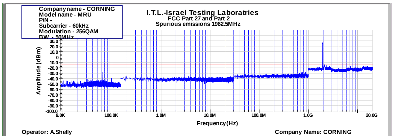
Figure 989: Spurious Emissions at Antenna Terminal 256QAM 50MHz B.W.; 1962.5MHz, 60kHz
