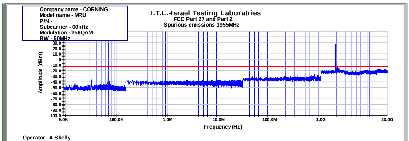
Figure 986: Spurious Emissions at Antenna Terminal 256QAM 50MHz B.W.; 1955.0MHz, 60kHz
