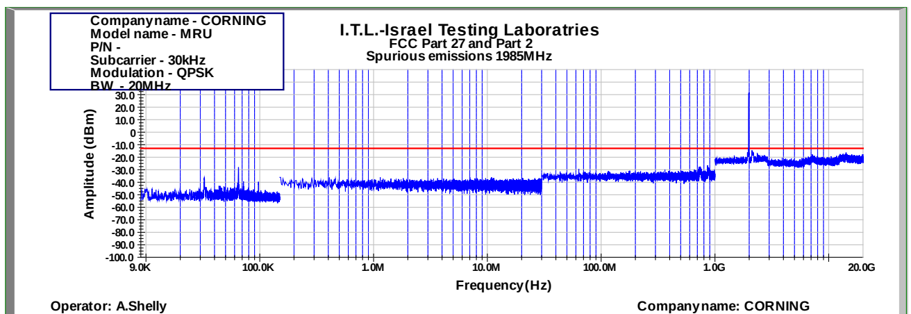
Figure 1030: Spurious Emissions at Antenna Terminal QPSK 20MHz B.W.; 1985.0MHz, 30kHz
