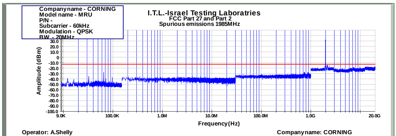
Figure 1031: Spurious Emissions at Antenna Terminal QPSK 20MHz B.W.; 1985.0MHz, 60kHz
