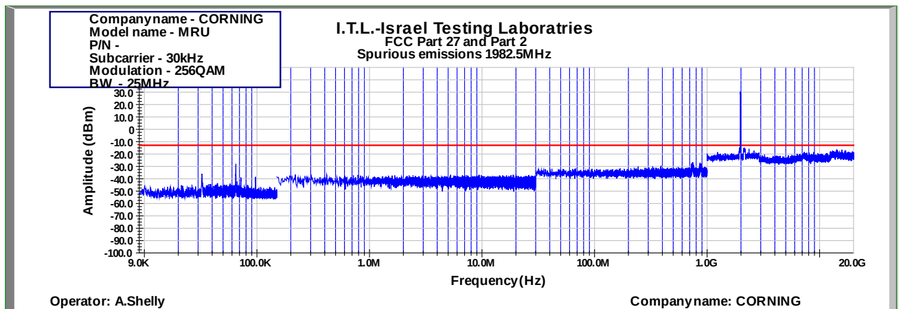
Figure 973: Spurious Emissions at Antenna Terminal 256QAM 25MHz B.W.; 1982.5MHz, 30kHz
