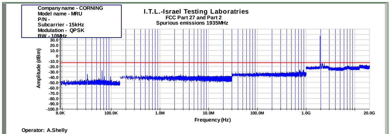
Figure 1005: Spurious Emissions at Antenna Terminal QPSK 10MHz B.W.; 1935.00MHz, 15kHz
