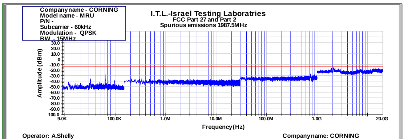
Figure 1022: Spurious Emissions at Antenna Terminal QPSK 15MHz B.W.; 1987.5MHz, 60kHz
