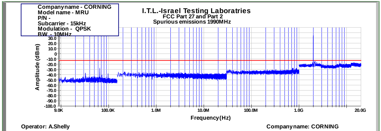
Figure 1011: Spurious Emissions at Antenna Terminal QPSK 10MHz B.W.; 1990.0MHz, 15kHz
