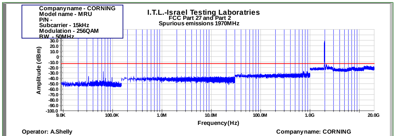
Figure 990: Spurious Emissions at Antenna Terminal 256QAM 50MHz B.W.; 1970.0MHz, 15kHz
