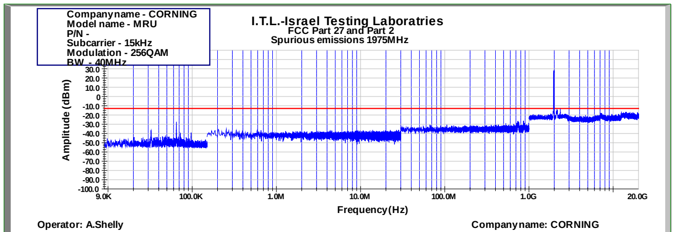
Figure 981: Spurious Emissions at Antenna Terminal 256QAM 40MHz B.W.; 1975.0MHz, 15kHz
