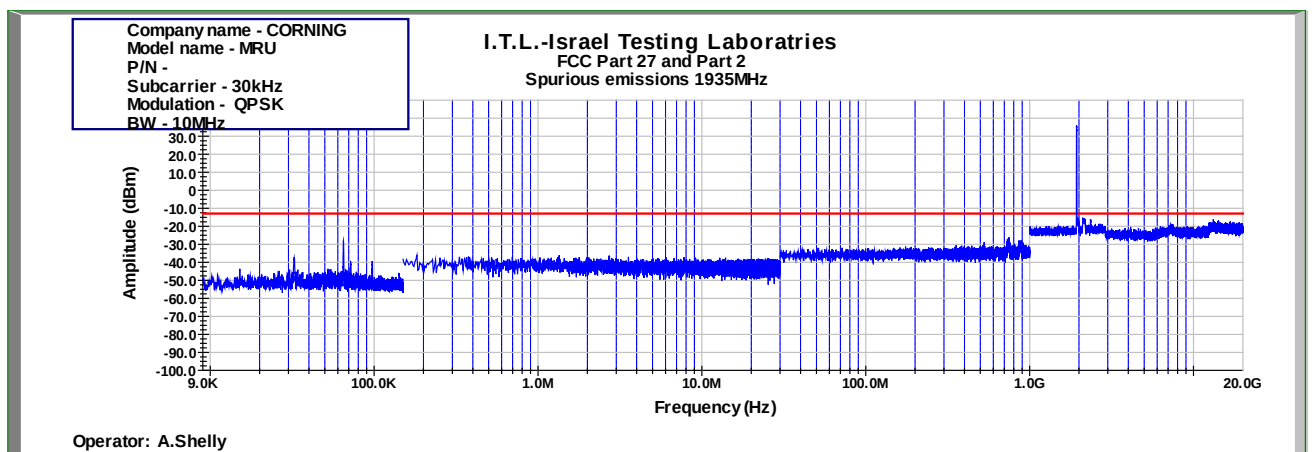
Figure 1006: Spurious Emissions at Antenna Terminal QPSK 10MHz B.W.; 1935.00MHz, 30kHz
