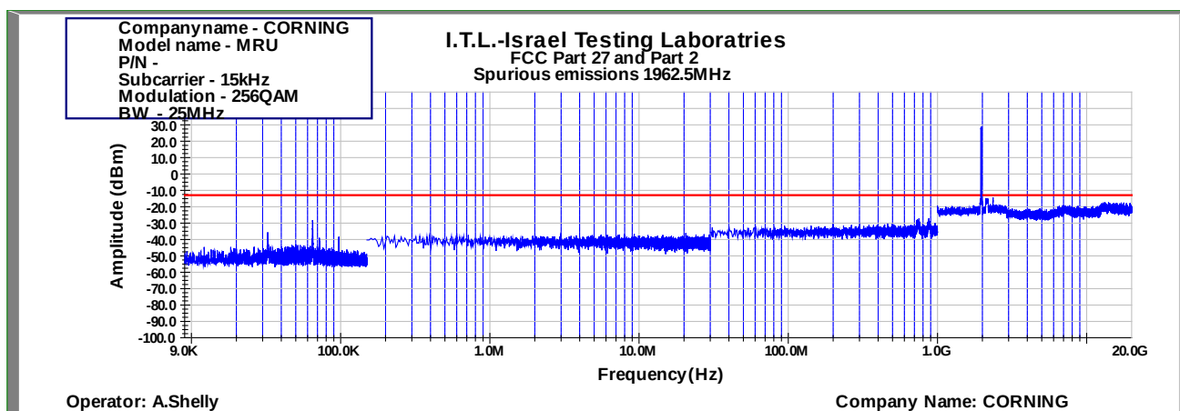
Figure 969: Spurious Emissions at Antenna Terminal 256QAM 25MHz B.W.; 1962.5MHz, 15kHz
