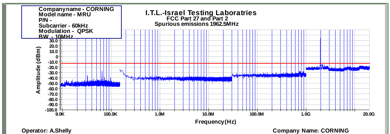
Figure 1010: Spurious Emissions at Antenna Terminal QPSK 10MHz B.W.; 1962.5MHz, 60kHz
