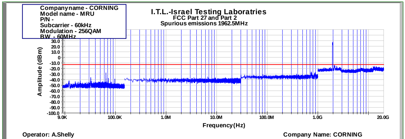
Figure 996: Spurious Emissions at Antenna Terminal 256QAM 60MHz B.W.; 1962.5MHz, 60kHz
