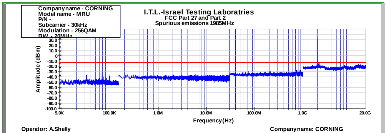
Figure 964: Spurious Emissions at Antenna Terminal 256QAM 20MHz B.W.; 1985.0MHz, 30kHz
