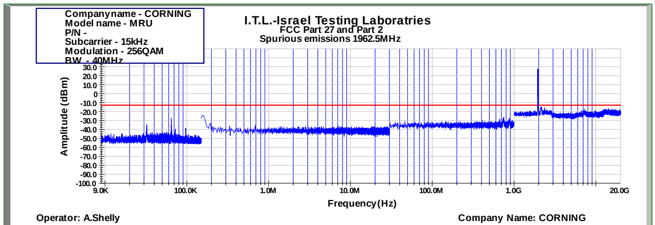
Figure 978: Spurious Emissions at Antenna Terminal 256QAM 40MHz B.W.; 1962.5MHz, 15kHz
