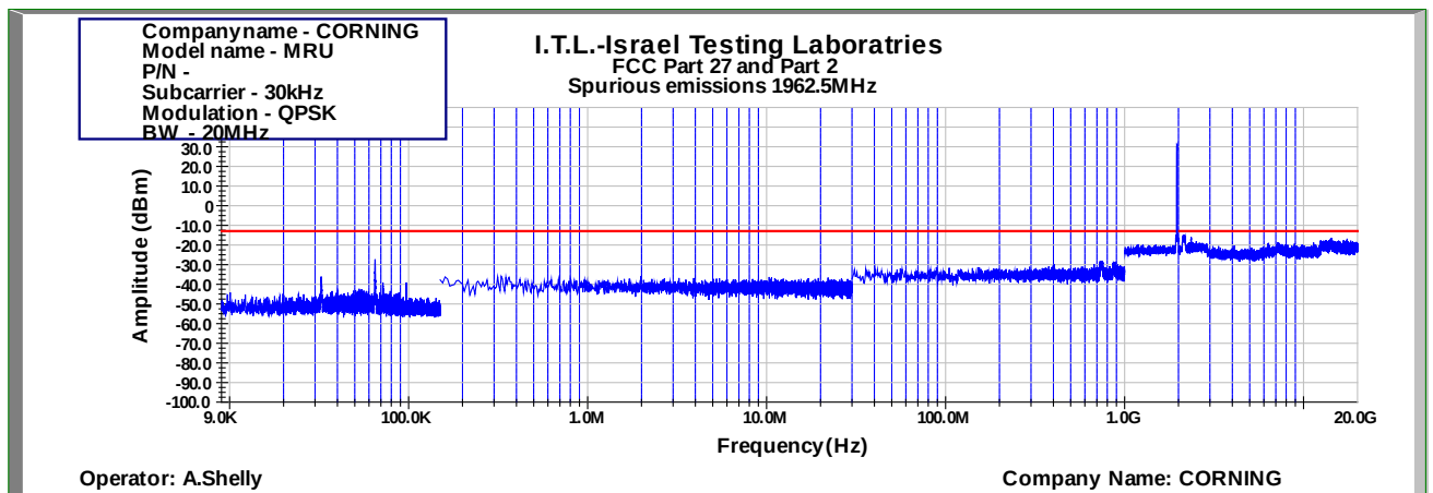
Figure 1027: Spurious Emissions at Antenna Terminal QPSK 20MHz B.W.; 1962.5MHz, 30kHz
