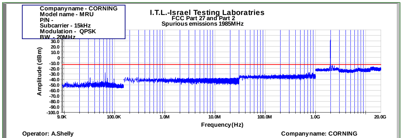
Figure 1029: Spurious Emissions at Antenna Terminal QPSK 20MHz B.W.; 1985.0MHz, 15kHz
