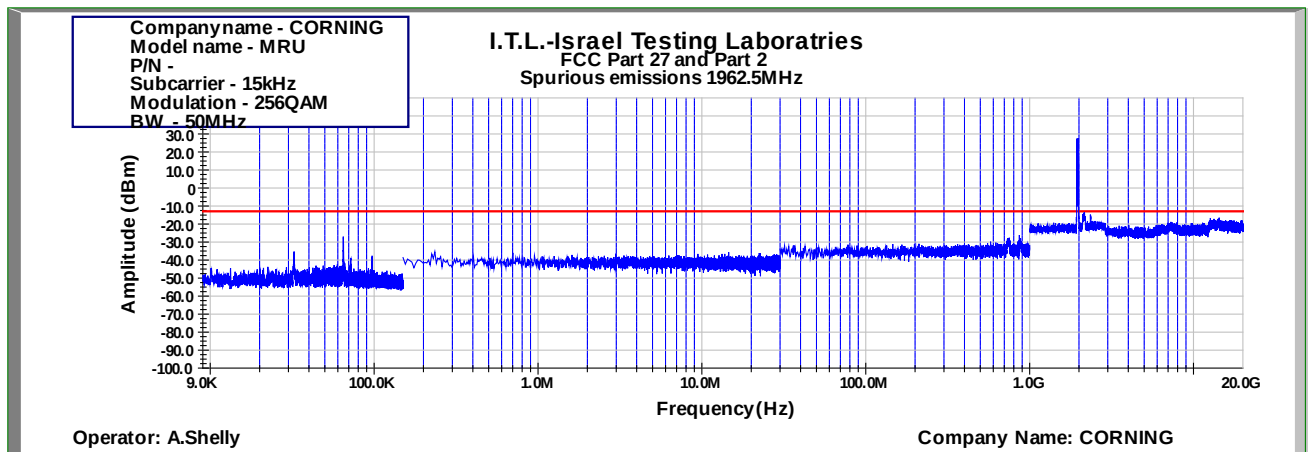
Figure 987: Spurious Emissions at Antenna Terminal 256QAM 50MHz B.W.; 1962.5MHz, 15kHz
