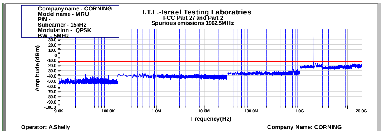
Figure 1001: Spurious Emissions at Antenna Terminal QPSK 5MHz B.W.; 1962.5MHz, 15kHz
