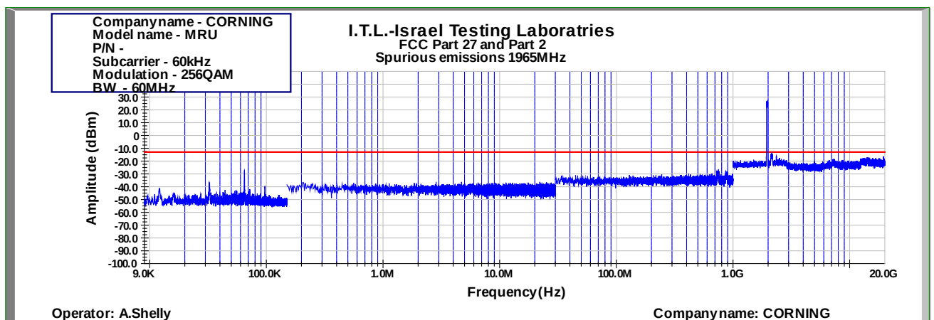
Figure 998: Spurious Emissions at Antenna Terminal 256QAM 60MHz B.W.; 1965.0MHz, 60kHz
