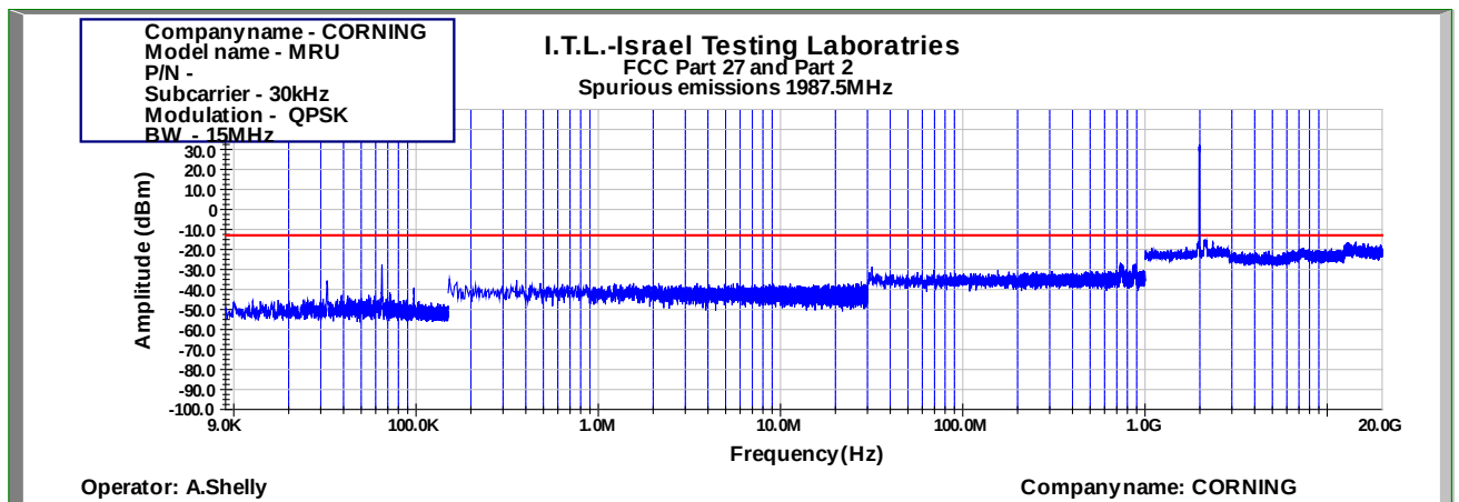
Figure 1021: Spurious Emissions at Antenna Terminal QPSK 15MHz B.W.; 1987.5MHz, 30kHz
