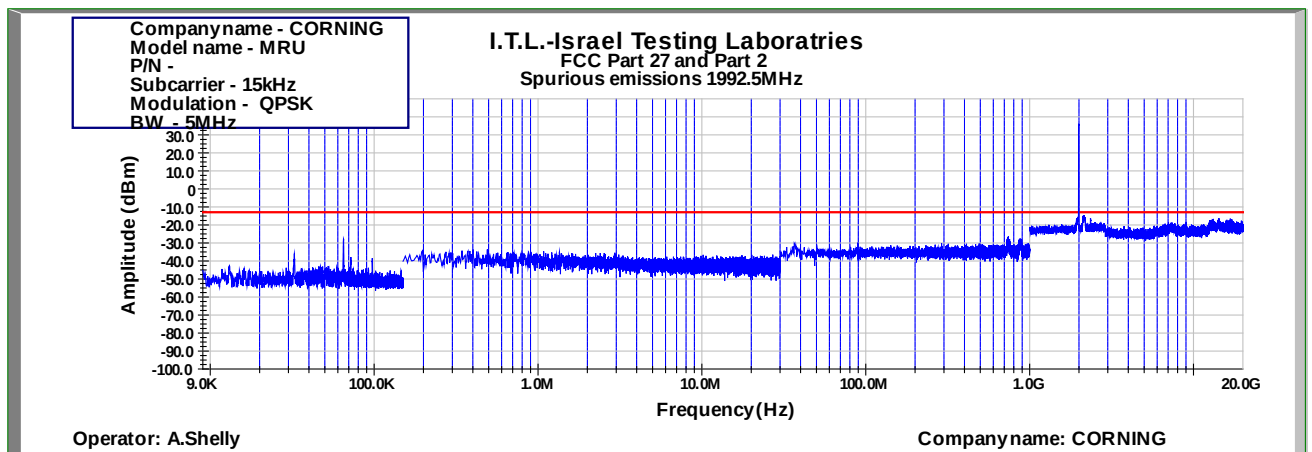
Figure 1003: Spurious Emissions at Antenna Terminal QPSK 5MHz B.W.; 1992.5MHz, 15kHz
