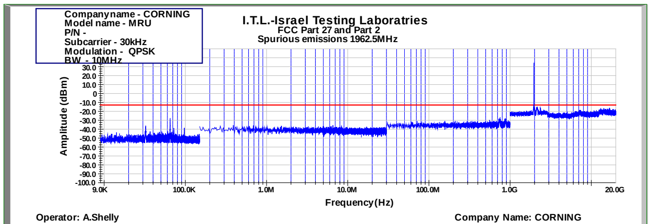
Figure 1009: Spurious Emissions at Antenna Terminal QPSK 10MHz B.W.; 1962.5MHz, 30kHz
