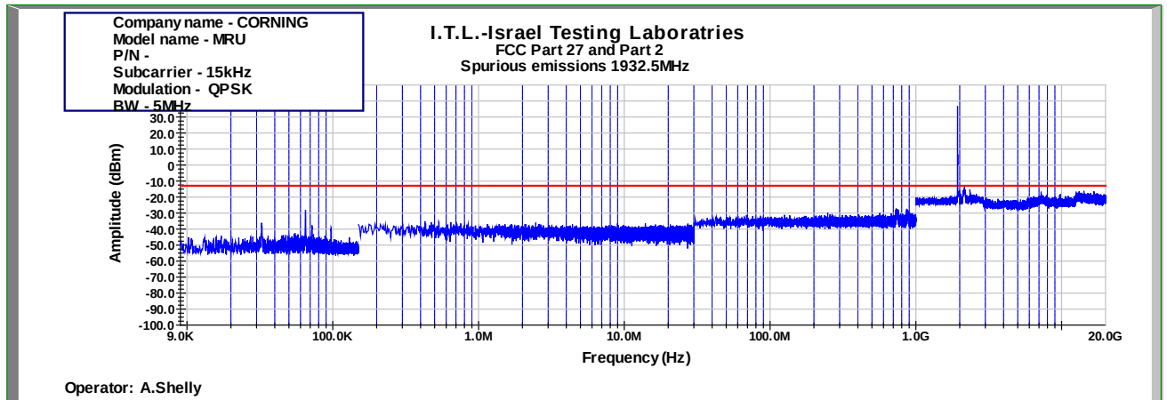
Figure 999: Spurious Emissions at Antenna Terminal QPSK 5MHz B.W.; 1932.5MHz, 15kHz
