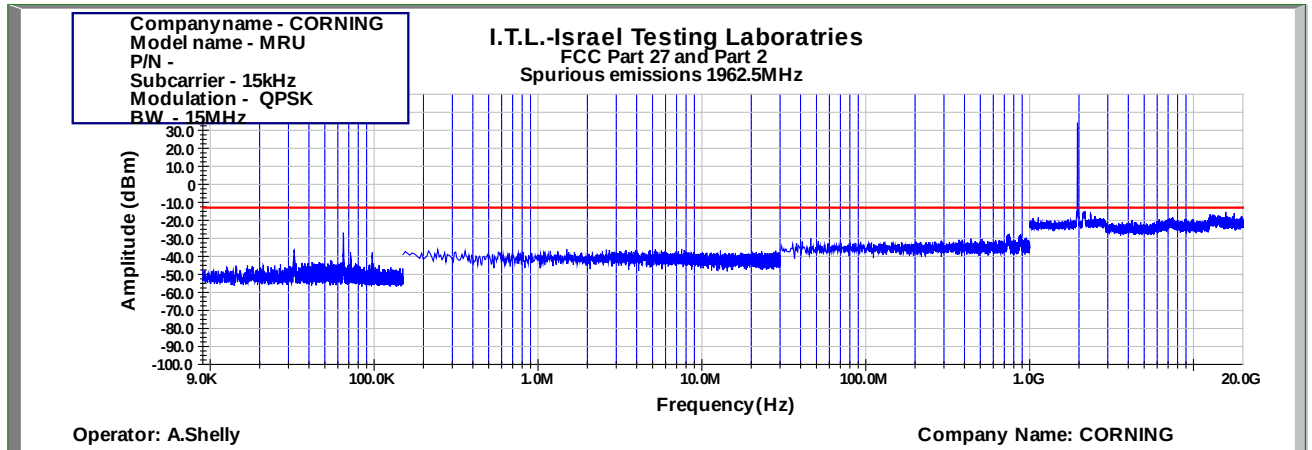
Figure 1017: Spurious Emissions at Antenna Terminal QPSK 15MHz B.W.; 1962.5MHz, 15kHz
