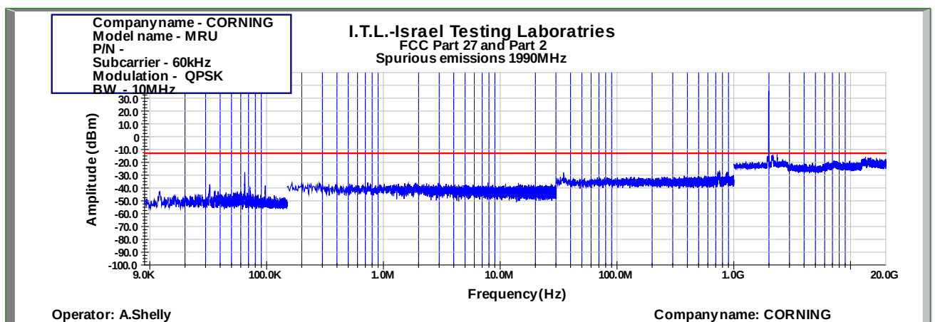
Figure 1013: Spurious Emissions at Antenna Terminal QPSK 10MHz B.W.; 1990.0MHz, 60kHz
