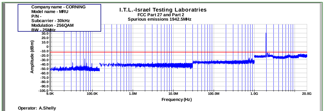
Figure 967: Spurious Emissions at Antenna Terminal 256QAM 25MHz B.W.; 1942.5MHz, 30kHz
