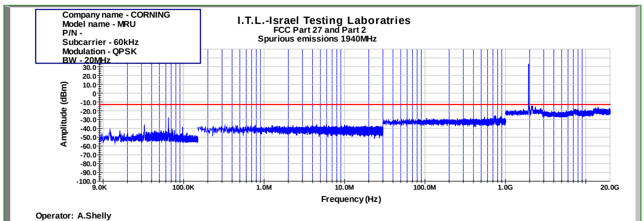
Figure 1025: Spurious Emissions at Antenna Terminal QPSK 20MHz B.W.; 1940.0MHz, 60kHz
