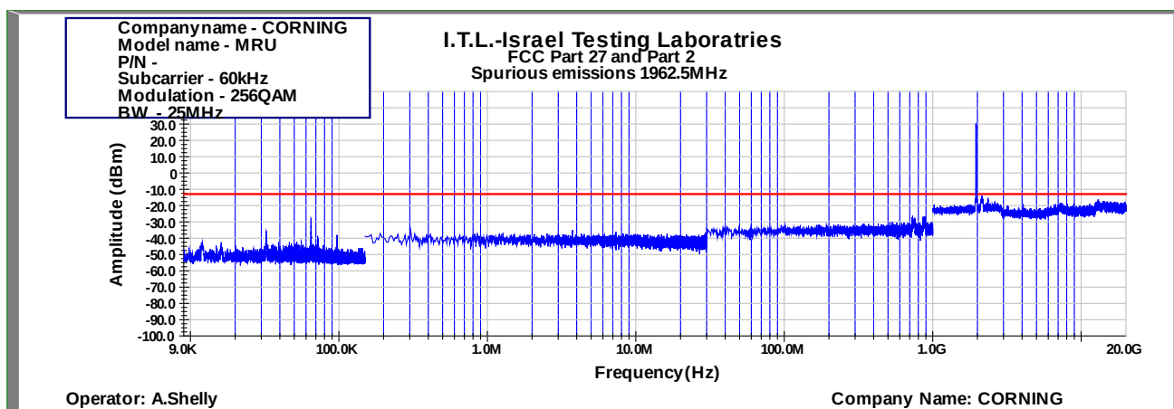
Figure 971: Spurious Emissions at Antenna Terminal 256QAM 25MHz B.W.; 1962.5MHz, 60kHz
