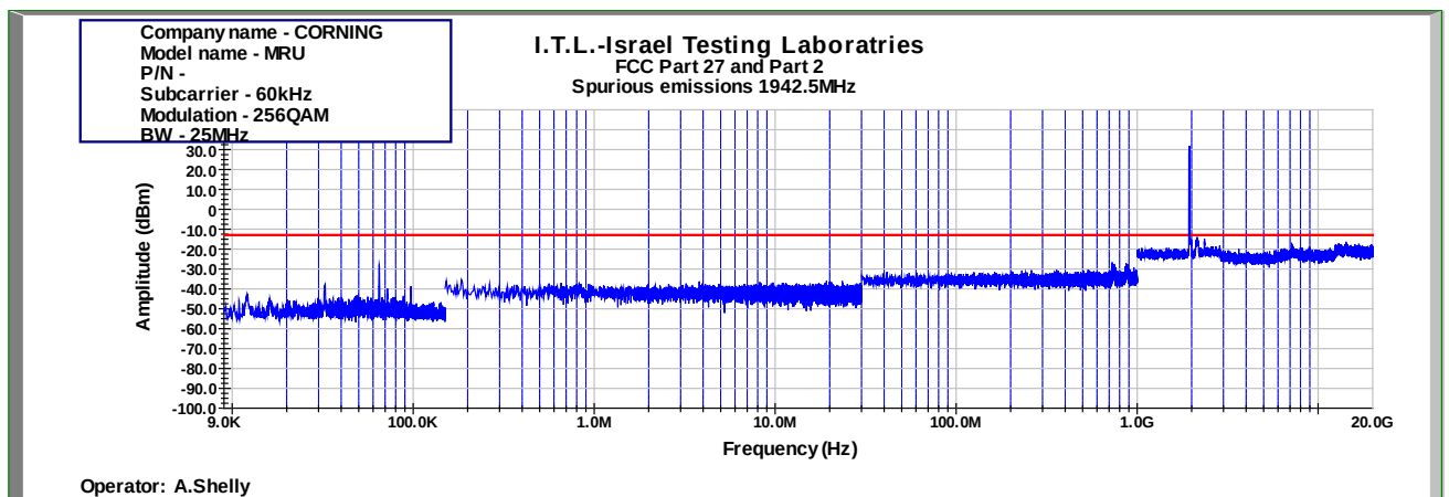
Figure 968: Spurious Emissions at Antenna Terminal 256QAM 25MHz B.W.; 1942.5MHz, 60kHz
