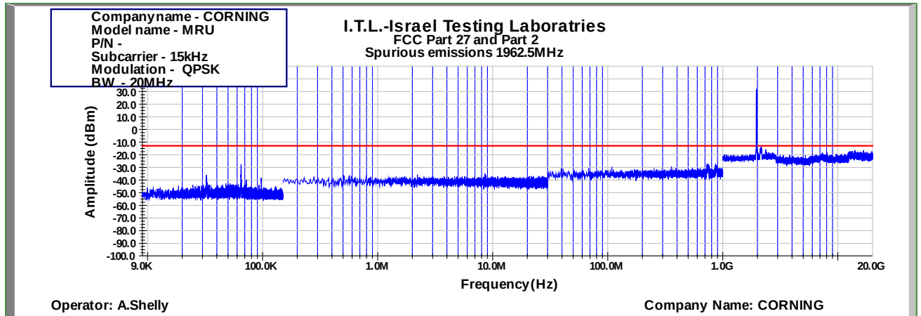
Figure 1026: Spurious Emissions at Antenna Terminal QPSK 20MHz B.W.; 1962.5MHz, 15kHz
