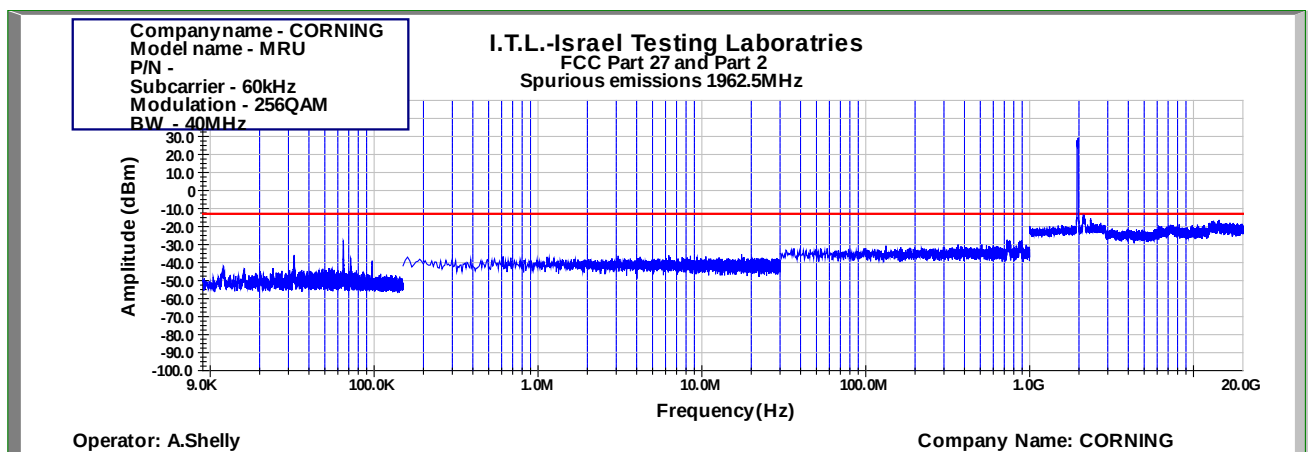
Figure 980: Spurious Emissions at Antenna Terminal 256QAM 40MHz B.W.; 1962.5MHz, 60kHz
