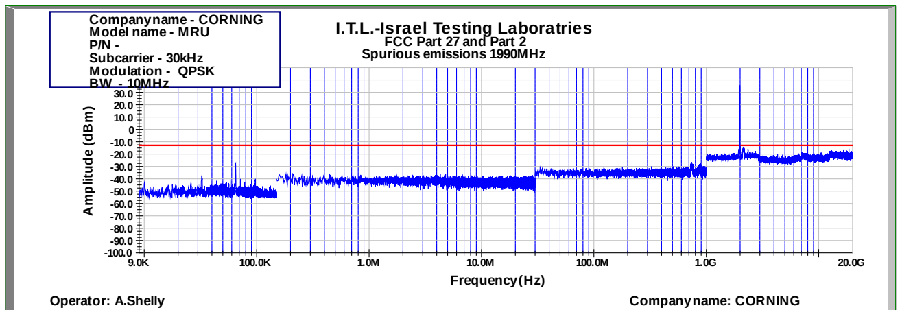
Figure 1012: Spurious Emissions at Antenna Terminal QPSK 10MHz B.W.; 1990.0MHz, 30kHz
