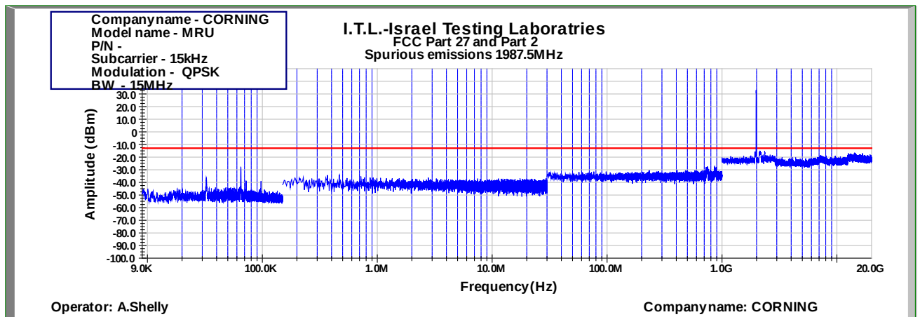
Figure 1020: Spurious Emissions at Antenna Terminal QPSK 15MHz B.W.; 1987.5MHz, 15kHz
