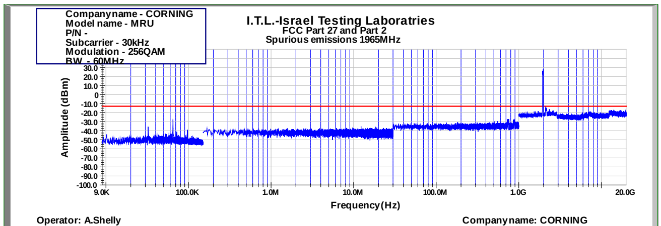
Figure 997: Spurious Emissions at Antenna Terminal 256QAM 60MHz B.W.; 1965.0MHz, 30kHz
