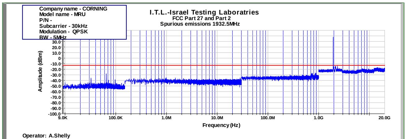
Figure 1000: Spurious Emissions at Antenna Terminal QPSK 5MHz B.W.; 1932.5MHz, 30kHz
