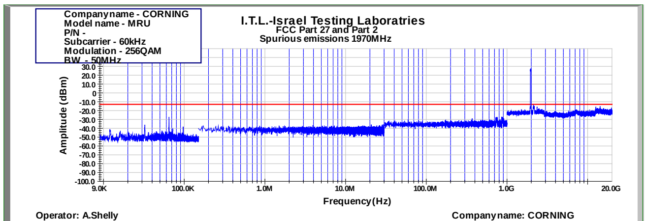
Figure 992: Spurious Emissions at Antenna Terminal 256QAM 50MHz B.W.; 1970.0MHz, 60kHz
