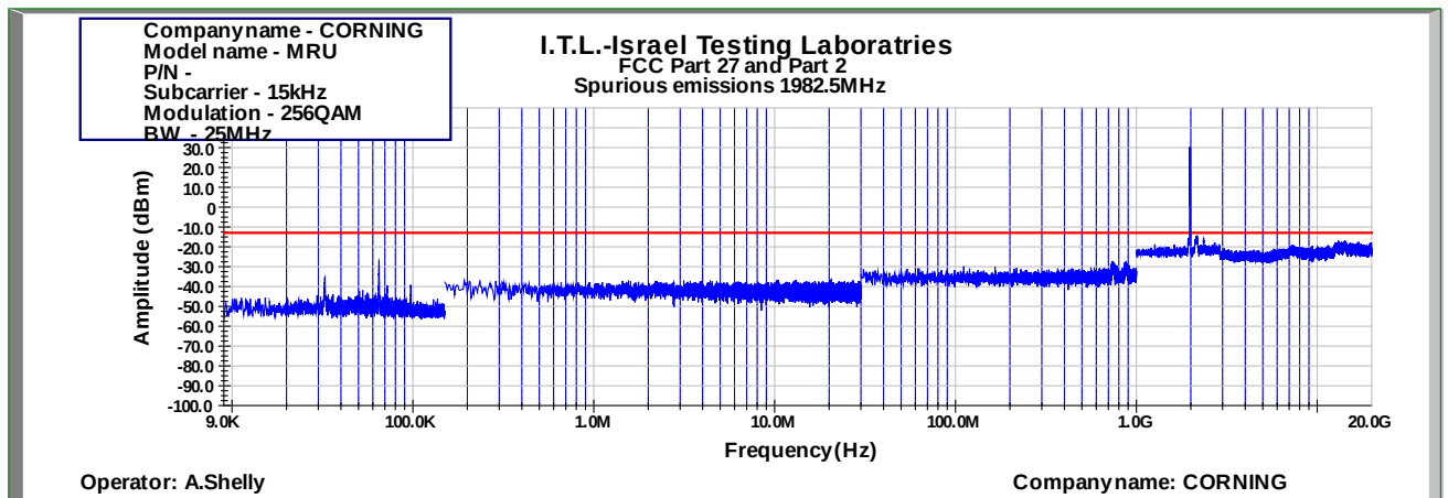
Figure 972: Spurious Emissions at Antenna Terminal 256QAM 25MHz B.W.; 1982.5MHz, 15kHz
