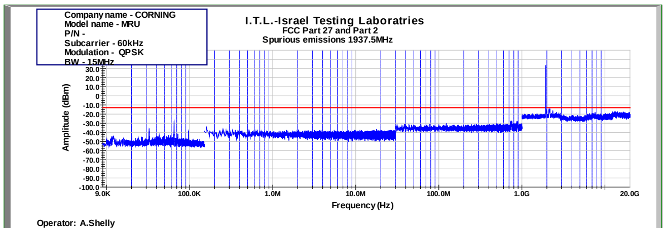
Figure 1016: Spurious Emissions at Antenna Terminal QPSK 15MHz B.W.; 1937.5MHz, 60kHz
