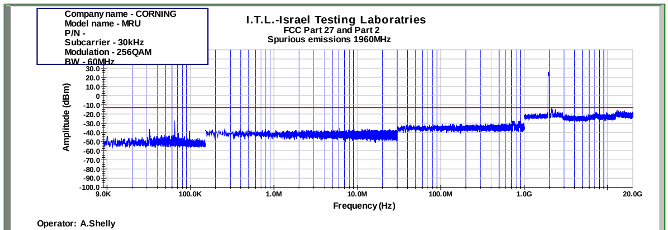
Figure 993: Spurious Emissions at Antenna Terminal 256QAM 60MHz B.W.; 1960.0MHz, 30kHz
