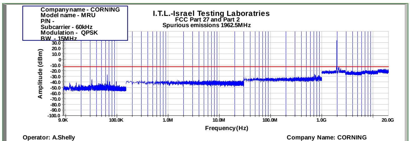
Figure 1019: Spurious Emissions at Antenna Terminal QPSK 15MHz B.W.; 1962.5MHz, 60kHz
