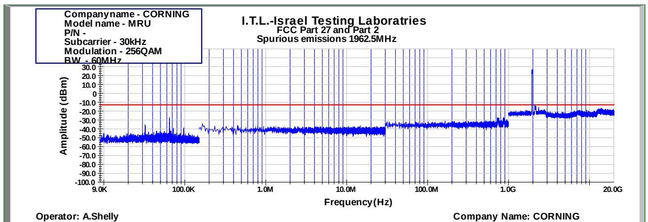
Figure 995: Spurious Emissions at Antenna Terminal 256QAM 60MHz B.W.; 1962.5MHz, 30kHz
