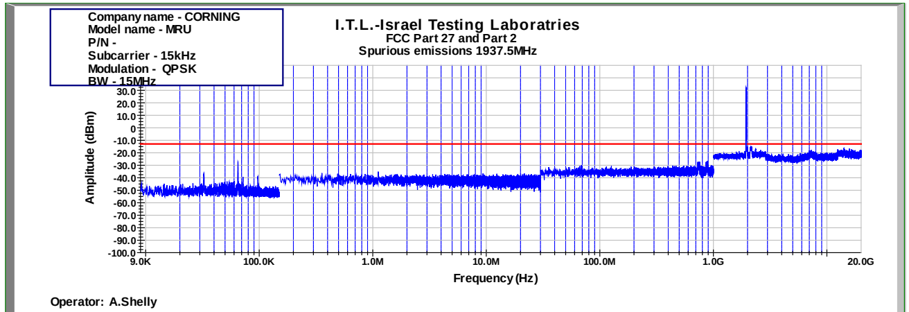
Figure 1014: Spurious Emissions at Antenna Terminal QPSK 15MHz B.W.; 1937.5MHz, 15kHz
