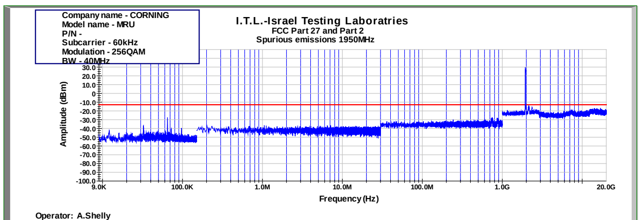
Figure 977: Spurious Emissions at Antenna Terminal 256QAM 40MHz B.W.; 1950.0MHz, 60kHz
