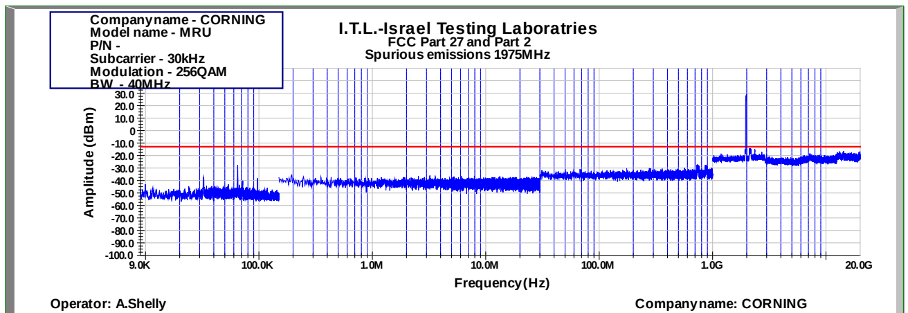
Figure 982: Spurious Emissions at Antenna Terminal 256QAM 40MHz B.W.; 1975.0MHz, 30kHz
