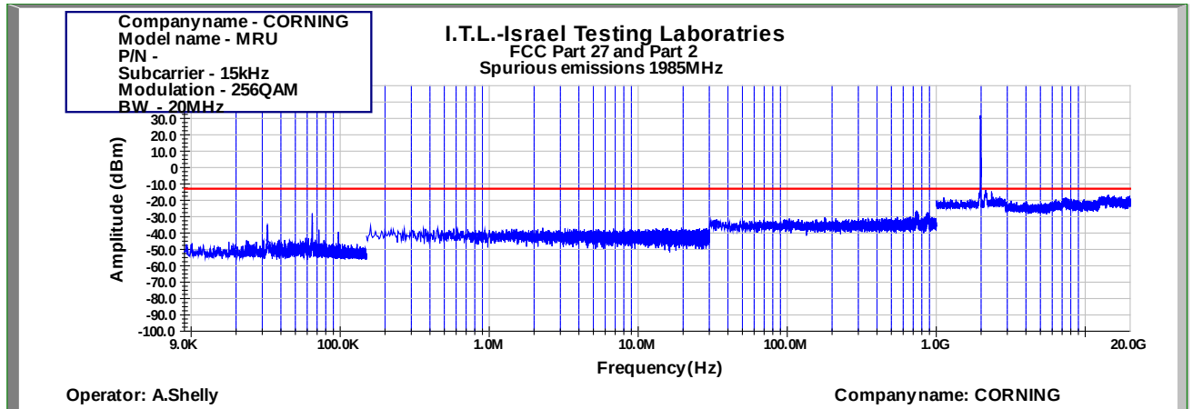
Figure 963: Spurious Emissions at Antenna Terminal 256QAM 20MHz B.W.; 1985.0MHz, 15kHz
