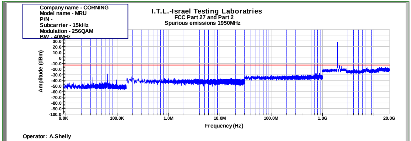
Figure 975: Spurious Emissions at Antenna Terminal 256QAM 40MHz B.W.; 1950.0MHz, 15kHz
