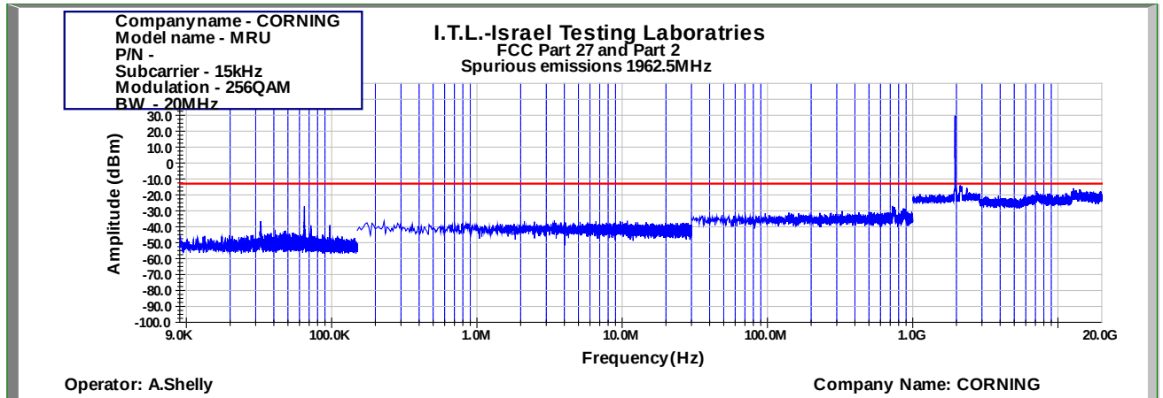
Figure 960: Spurious Emissions at Antenna Terminal 256QAM 20MHz B.W.; 1962.5MHz, 15kHz
