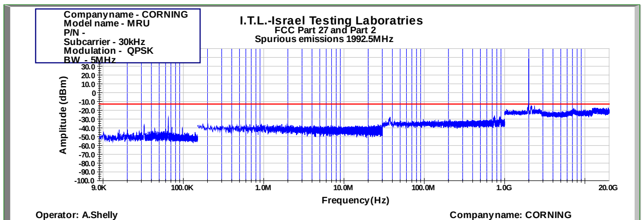
Figure 1004: Spurious Emissions at Antenna Terminal QPSK 5MHz B.W.; 1992.5MHz, 30kHz
