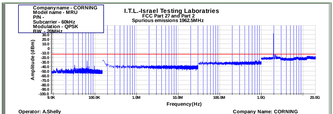
Figure 1028: Spurious Emissions at Antenna Terminal QPSK 20MHz B.W.; 1962.5MHz, 60kHz
