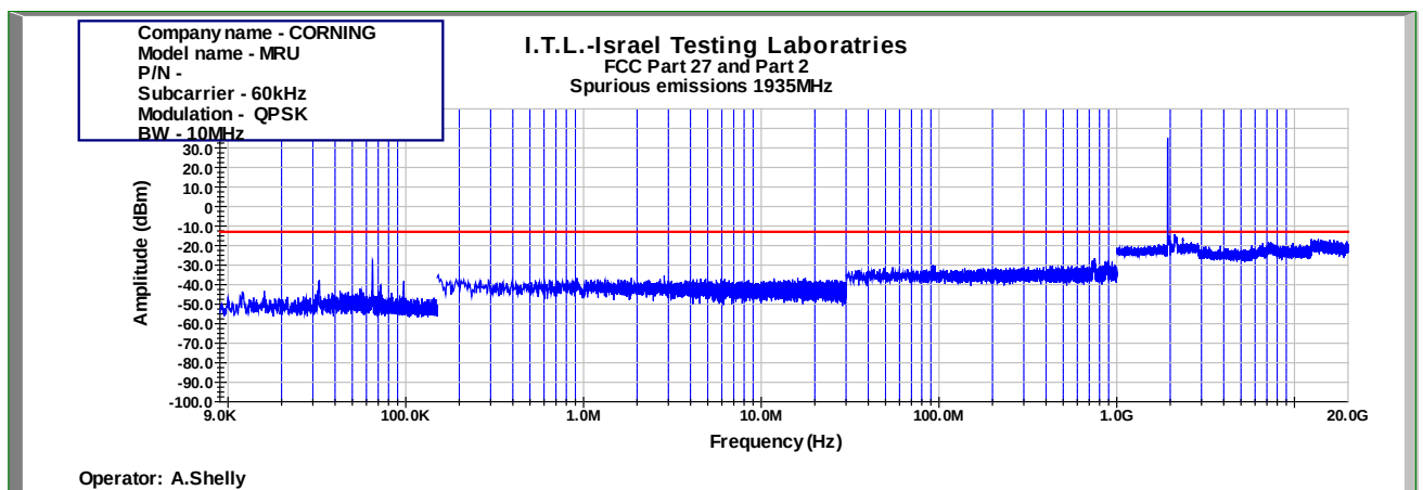
Figure 1007: Spurious Emissions at Antenna Terminal QPSK 10MHz B.W.; 1935.00MHz, 60kHz
