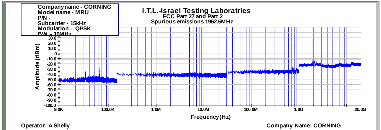
Figure 1008: Spurious Emissions at Antenna Terminal QPSK 10MHz B.W.; 1962.5MHz, 15kHz
