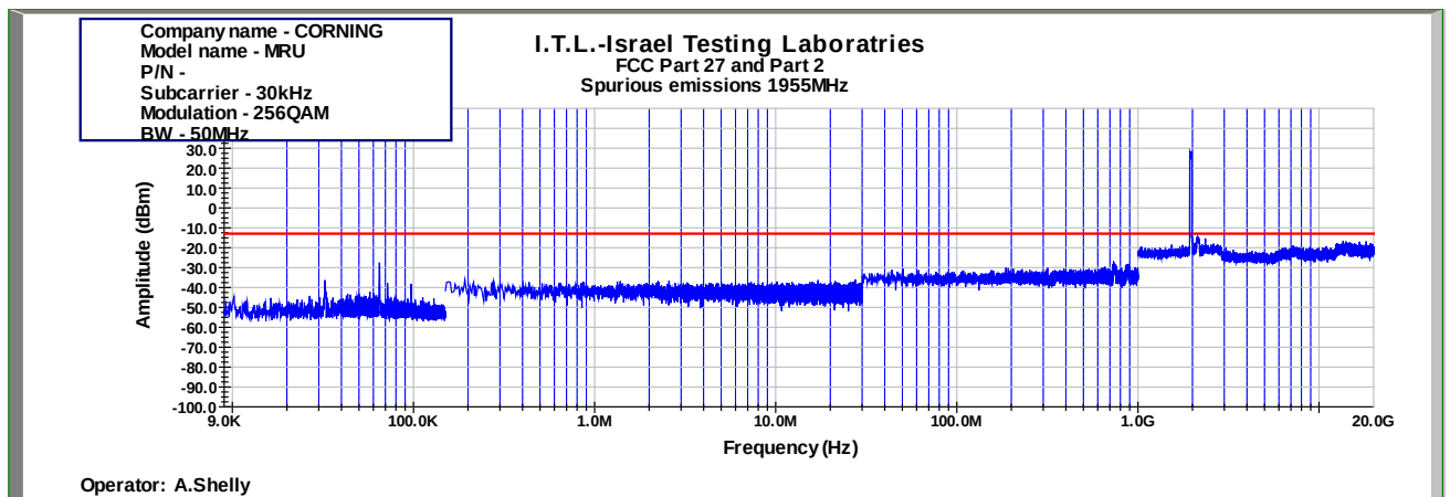
Figure 985: Spurious Emissions at Antenna Terminal 256QAM 50MHz B.W.; 1955.0MHz, 30kHz
