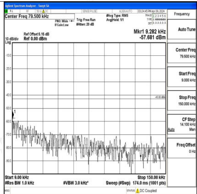
Band66_15MHz_16QAM_132047_1RB#0_0.009~0.15_0.00 9~0.15
