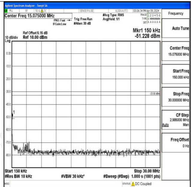
Band66_15MHz_QPSK_132597_1RB#0_0.15~30_0.15~30
