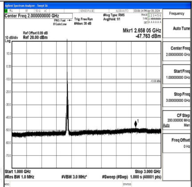
Band66_10MHz_QPSK_132322_1RB#0_1000~3000_1000 ~3000
