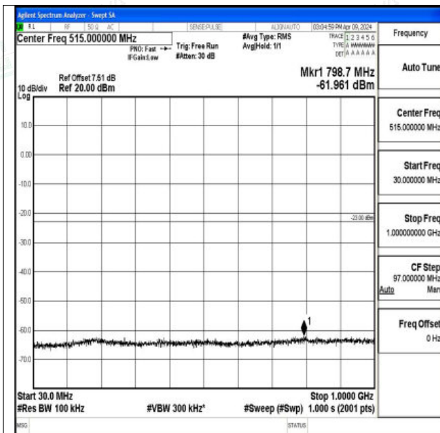
Band66_10MHz_QPSK_132022_1RB#0_30~1000_30~1000
