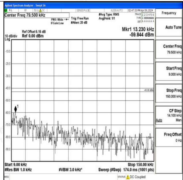
Band66_5MHz_16QAM_132647_1RB#0_0.009~0.15_0.009 ~0.15
