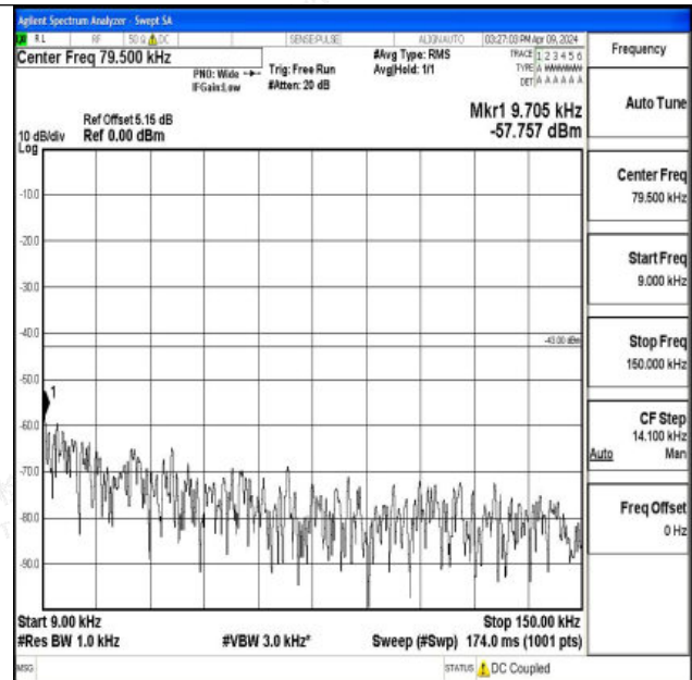
Band66_15MHz_16QAM_132597_1RB#0_0.009~0.15_0.00 9~0.15
