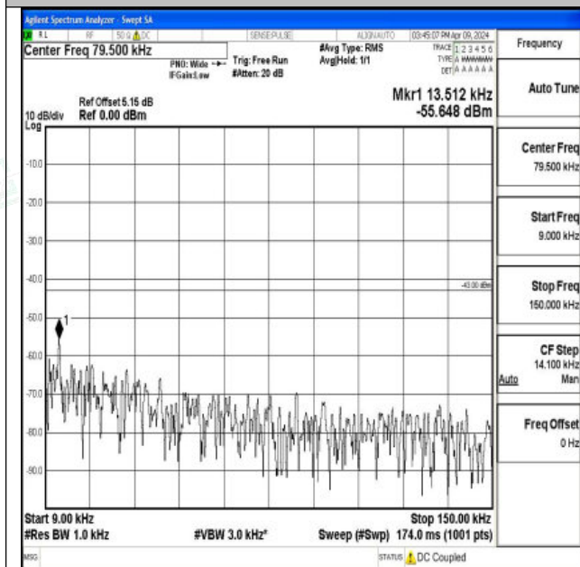
Band66_20MHz_QPSK_132572_1RB#0_0.009~0.15_0.00 9~0.15
