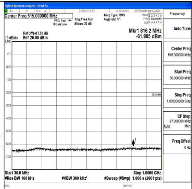
Band66_10MHz_16QAM_132022_1RB#0_30~1000_30~10
