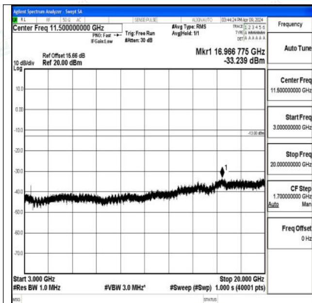
Band66_20MHz_QPSK_132322_1RB#0_3000~20000_30 00~20000
