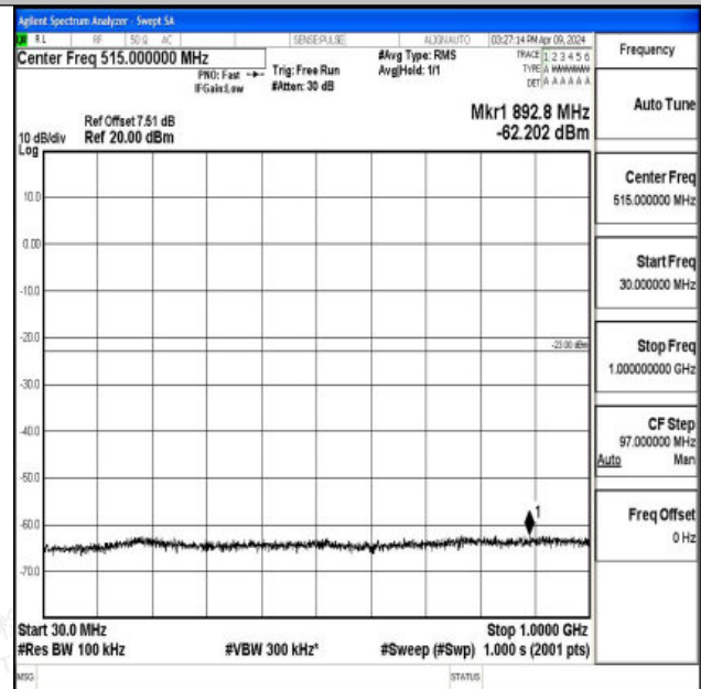
Band66_15MHz_16QAM_132597_1RB#0_30~1000_30~10 00
