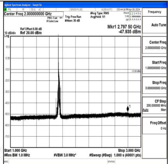
Band66_20MHz_QPSK_132322_1RB#0_1000~3000_1000 ~3000
