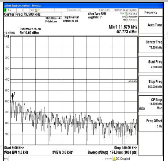
Band66_10MHz_16QAM_132022_1RB#0_0.009~0.15_0.009~0.15
