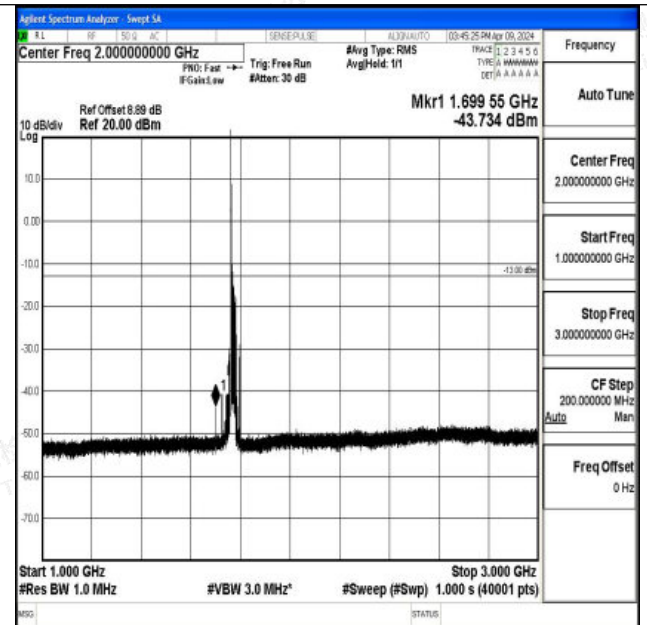
Band66_20MHz_QPSK_132572_1RB#0_1000~3000_1000~3000
