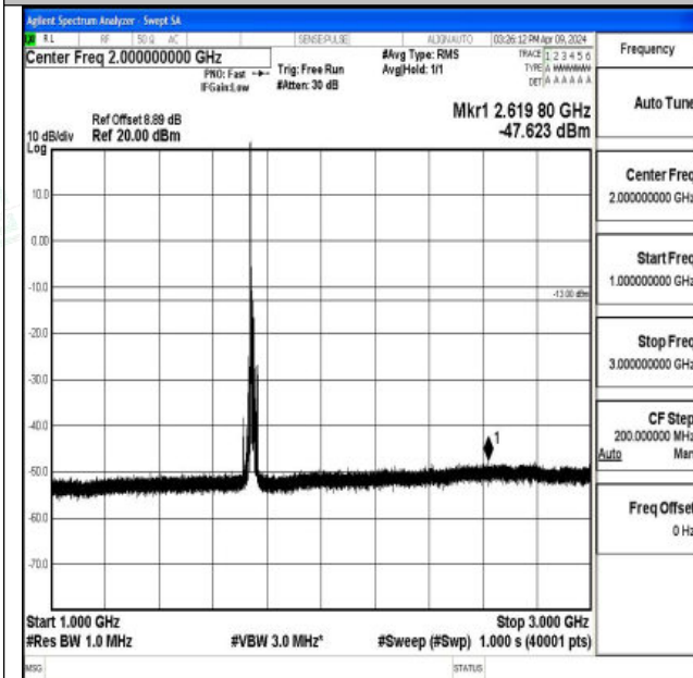
Band66_15MHz_16QAM_132322_1RB#0_1000~3000_10
