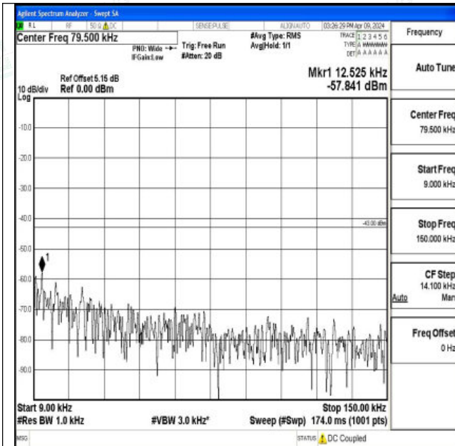
Band66_15MHz_QPSK_132597_1RB#0_0.009~0.15_0.00 9~0.15
