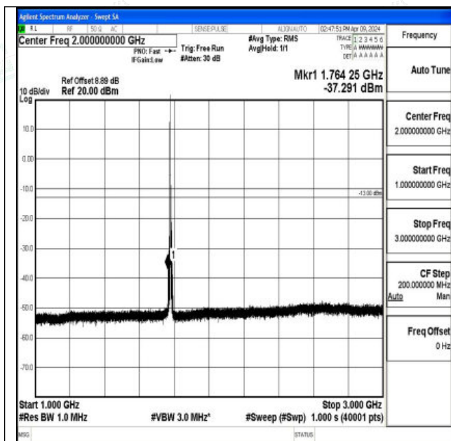
Band66_5MHz_16QAM_132647_1RB#0_1000~3000_100 0~3000
