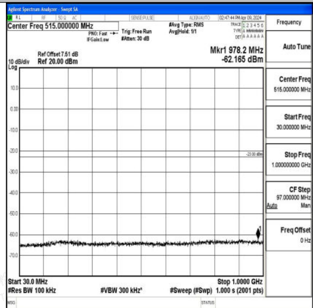
Band66_5MHz_16QAM_132647_1RB#0_30~1000_30~100 0
