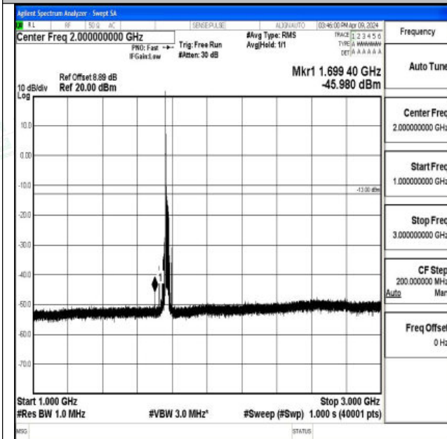
Band66_20MHz_16QAM_132572_1RB#0_1000~3000_10
