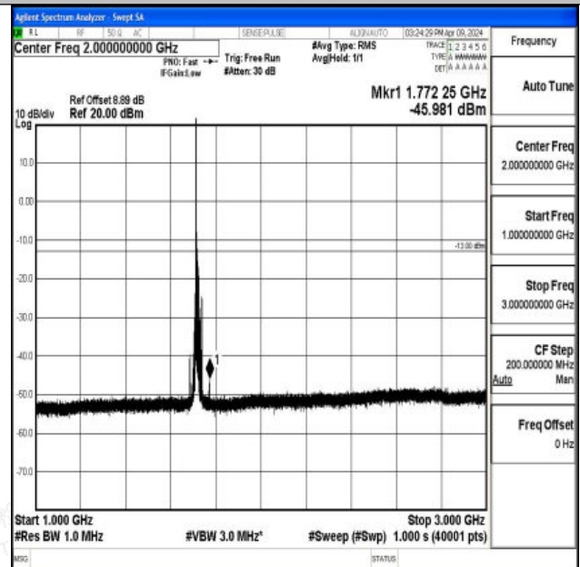
Band66_15MHz_QPSK_132047_1RB#0_1000~3000_1000 ~3000
