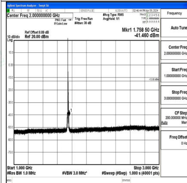
Band66_5MHz_16QAM_132322_1RB#0_1000~3000_1000~3000
