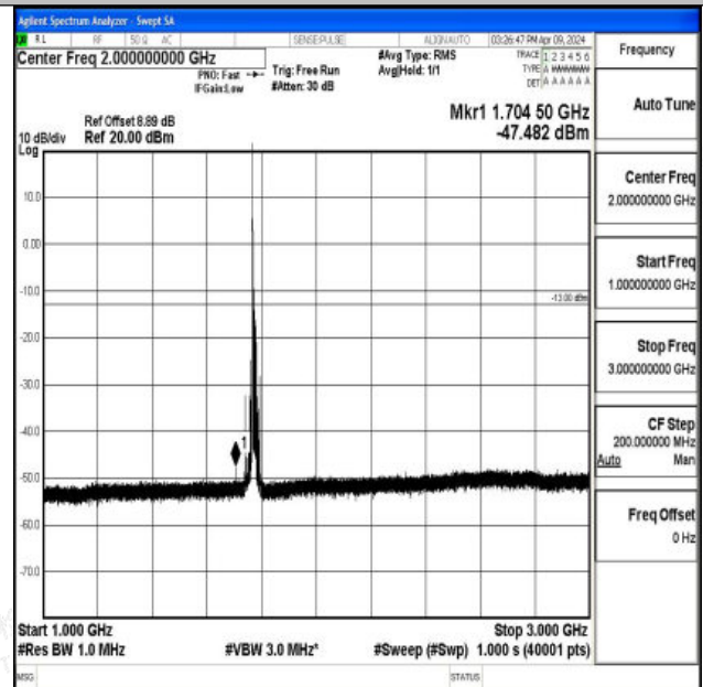
Band66_15MHz_QPSK_132597_1RB#0_1000~3000_1000 ~3000
