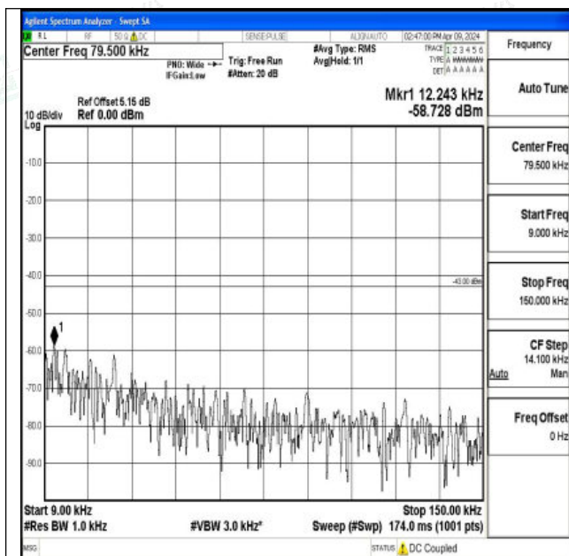
Band66_5MHz_QPSK_132647_1RB#0_0.009~0.15_0.009~0.15
