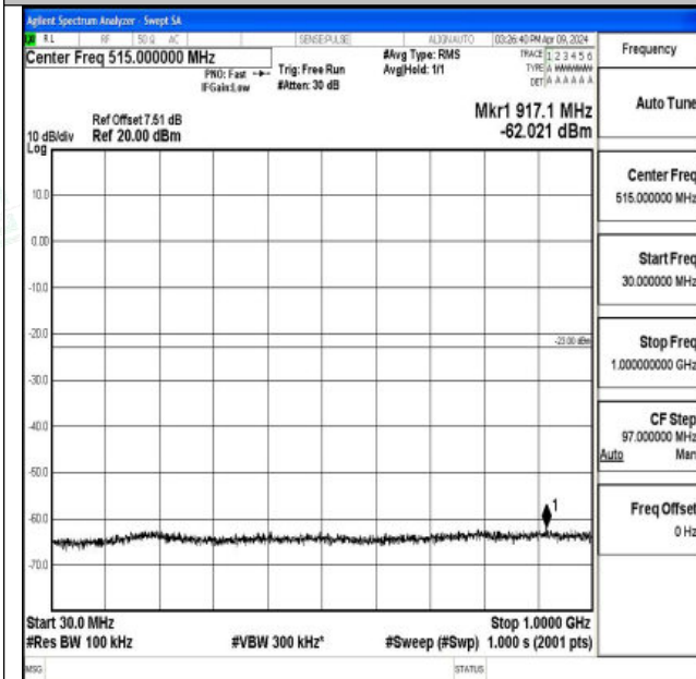
Band66_15MHz_QPSK_132597_1RB#0_30~1000_30~10 00
