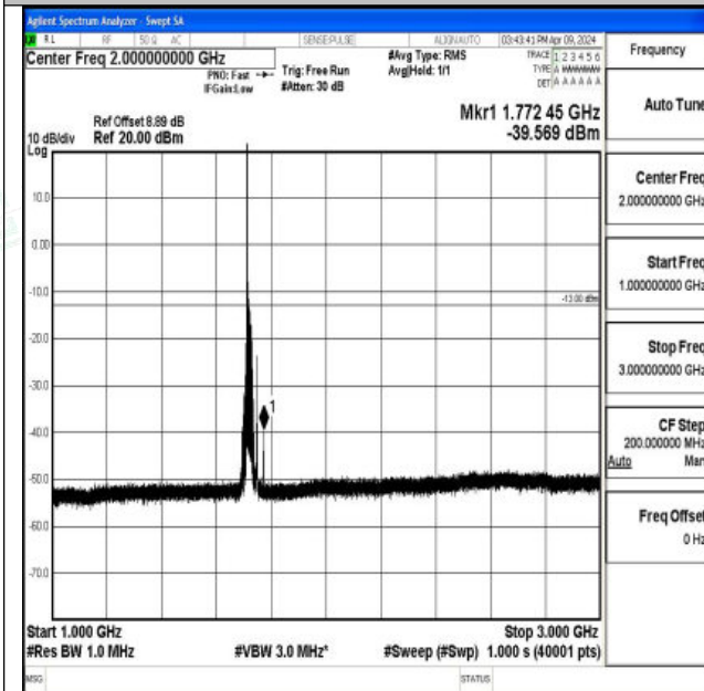
Band66_20MHz_16QAM_132072_1RB#0_1000~3000_10
