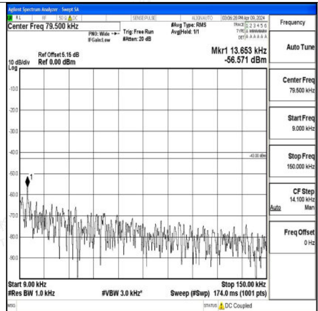
Band66_10MHz_16QAM_132322_1RB#0_0.009~0.15_0.00 9~0.15
