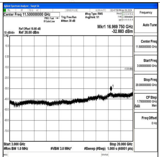
Band66_5MHz_16QAM_132647_1RB#0_3000~20000_300 0~20000
