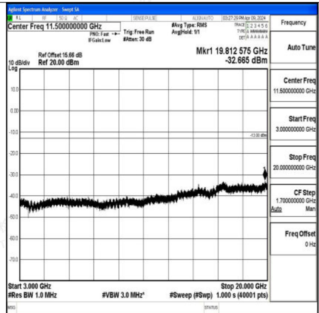
Band66_15MHz_16QAM_132597_1RB#0_3000~20000_30 00~20000
