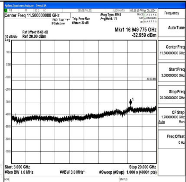
Band66_15MHz_16QAM_132322_1RB#0_3000~20000_30
