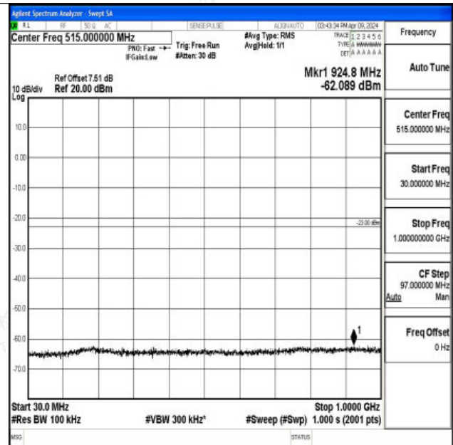
Band66_20MHz_16QAM_132072_1RB#0_30~1000_30~10
