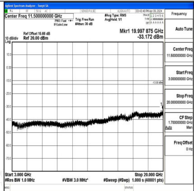
Band66_20MHz_16QAM_132072_1RB#0_3000~20000_30
