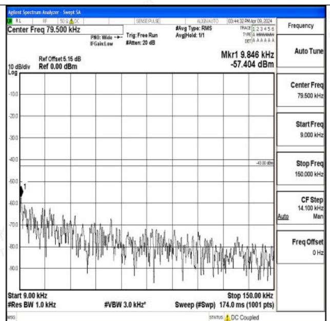
Band66_20MHz_16QAM_132322_1RB#0_0.009~0.15_0.00 9~0.15
