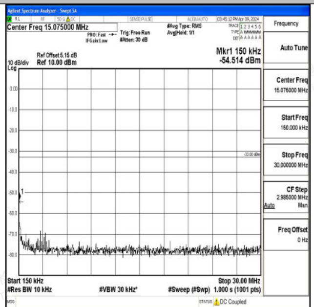
Band66_20MHz_QPSK_132572_1RB#0_0.15~30_0.15~30
