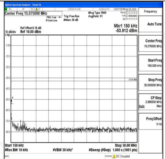
Band66_10MHz_QPSK_132622_1RB#0_0.15~30_0.15~30
