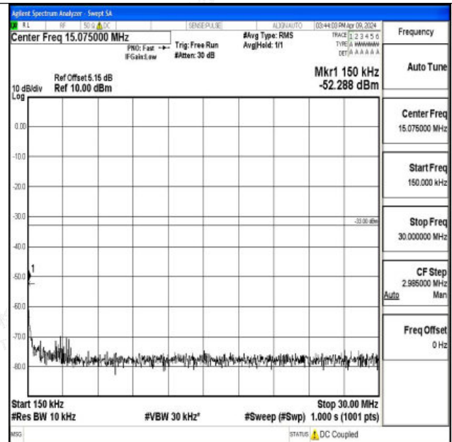
Band66_20MHz_QPSK_132322_1RB#0_0.15~30_0.15~30
