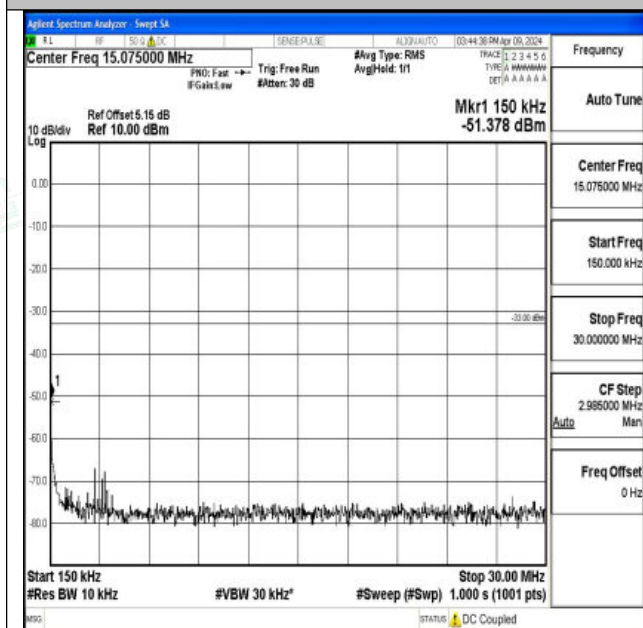
Band66_20MHz_16QAM_132322_1RB#0_0.15~30_0.15~ 30
