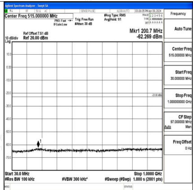
Band66_15MHz_16QAM_132322_1RB#0_30~1000_30~10
