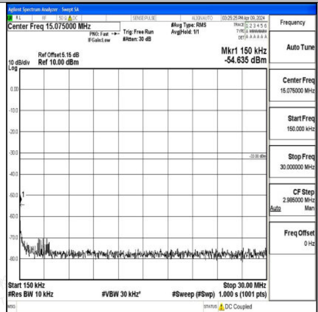
Band66_15MHz_QPSK_132322_1RB#0_0.15~30_0.15~30
