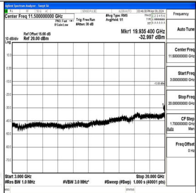
Band66_20MHz_16QAM_132572_1RB#0_3000~20000_30
