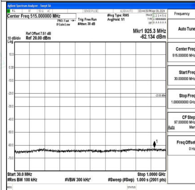
Band66_20MHz_QPSK_132322_1RB#0_30~1000_30~10 00
