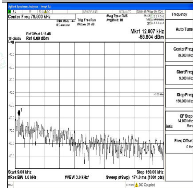
Band66_10MHz_QPSK_132022_1RB#0_0.009~0.15_0.00 9~0.15
