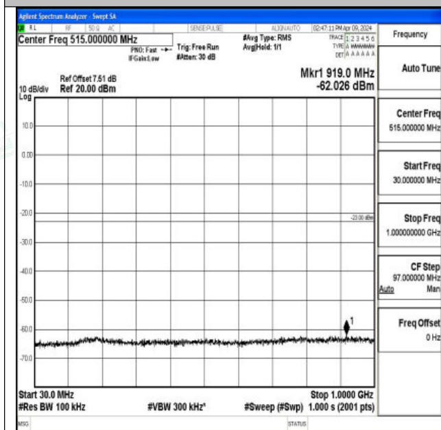
Band66_5MHz_QPSK_132647_1RB#0_30~1000_30~1000
