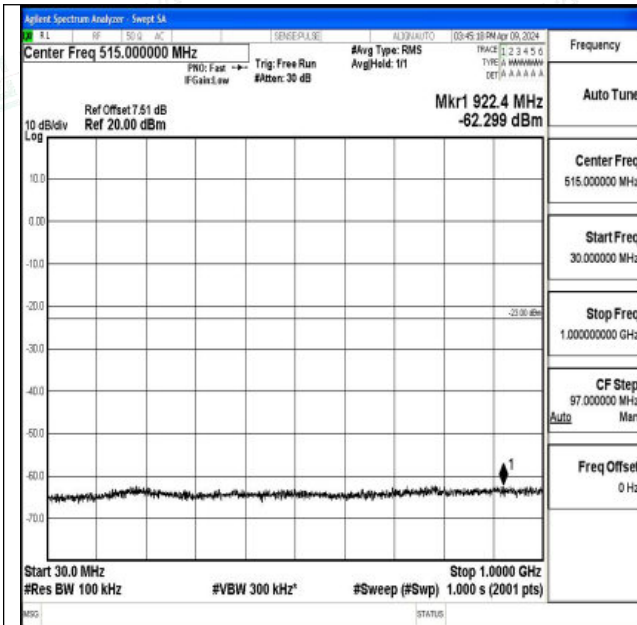
Band66_20MHz_QPSK_132572_1RB#0_30~1000_30~1000
