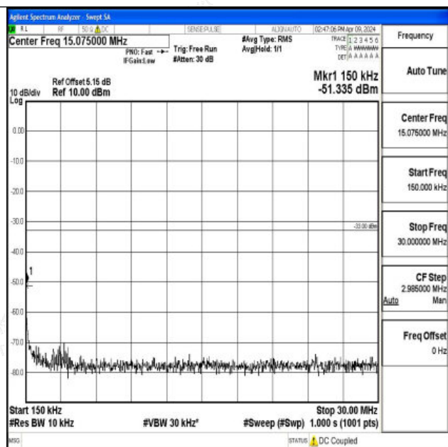
Band66_5MHz_QPSK_132647_1RB#0_0.15~30_0.15~30
