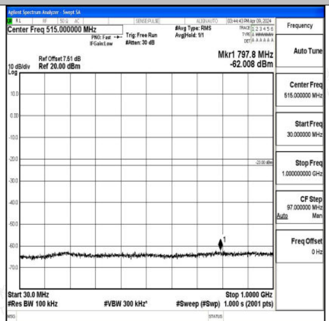
Band66_20MHz_16QAM_132322_1RB#0_30~1000_30~10 00
