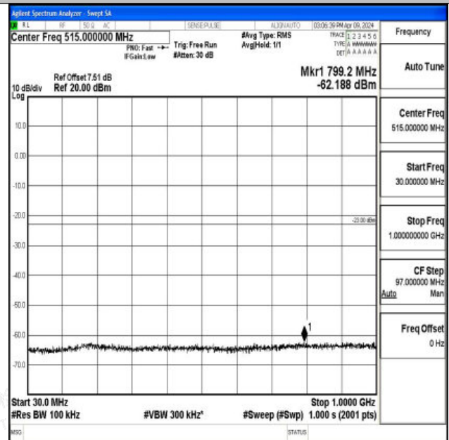
Band66_10MHz_16QAM_132322_1RB#0_30~1000_30~10 00
