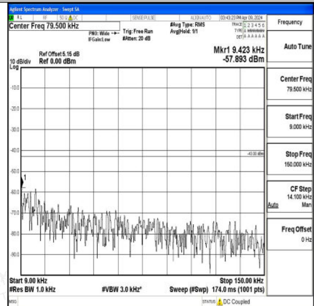
Band66_20MHz_16QAM_132072_1RB#0_0.009~0.15_0.009~0.15
