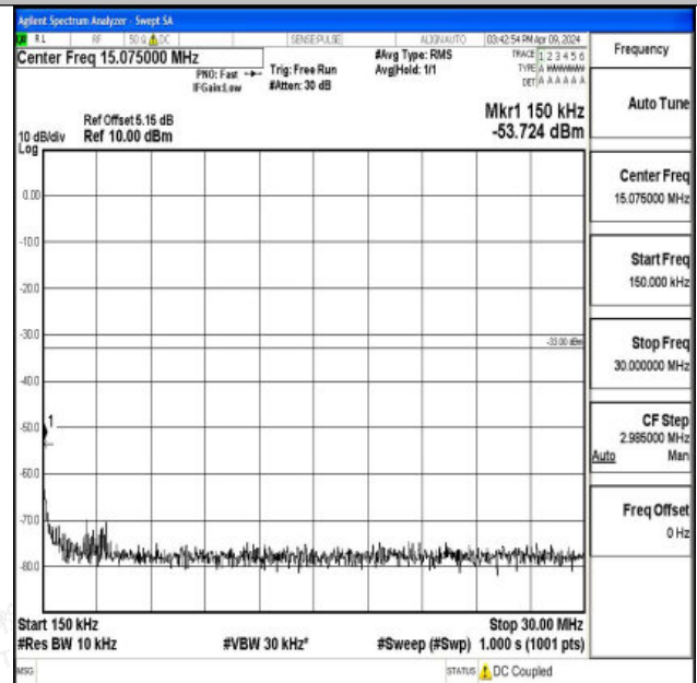
Band66_20MHz_QPSK_132072_1RB#0_0.15~30_0.15~30
