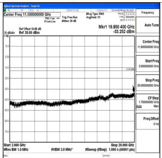
Band66_20MHz_16QAM_132322_1RB#0_3000~20000_30 00~20000
