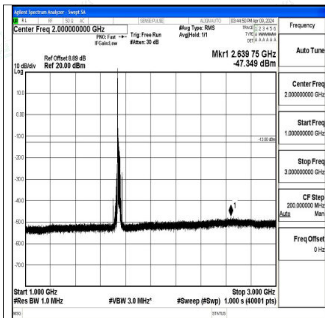
Band66_20MHz_16QAM_132322_1RB#0_1000~3000_10 00~3000
