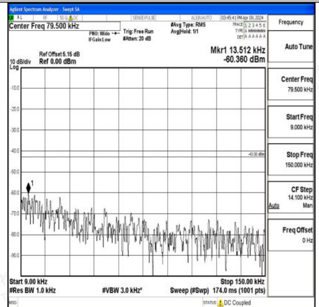
Band66_20MHz_16QAM_132572_1RB#0_0.009~0.15_0.009~0.15
