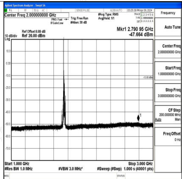
Band66_15MHz_QPSK_132322_1RB#0_1000~3000_1000 ~3000
