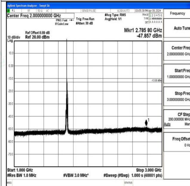
Band66_10MHz_16QAM_132022_1RB#0_1000~3000_10
