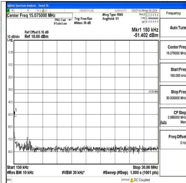
Band66_10MHz_16QAM_132622_1RB#0_0.15~30_0.15~30
