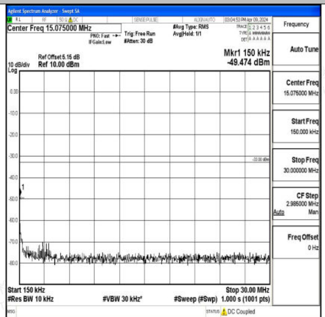
Band66_10MHz_QPSK_132022_1RB#0_0.15~30_0.15~30
