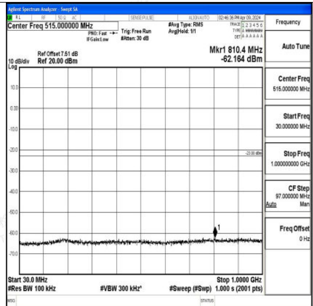
Band66_5MHz_16QAM_132322_1RB#0_30~1000_30~100
