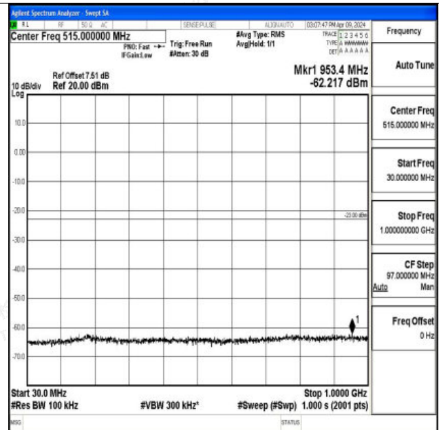
Band66_10MHz_16QAM_132622_1RB#0_30~1000_30~10
