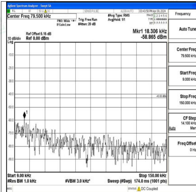
Band66_20MHz_QPSK_132322_1RB#0_0.009~0.15_0.00 9~0.15
