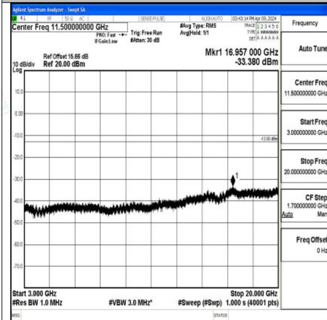
Band66_20MHz_QPSK_132072_1RB#0_3000~20000_3000~20000
