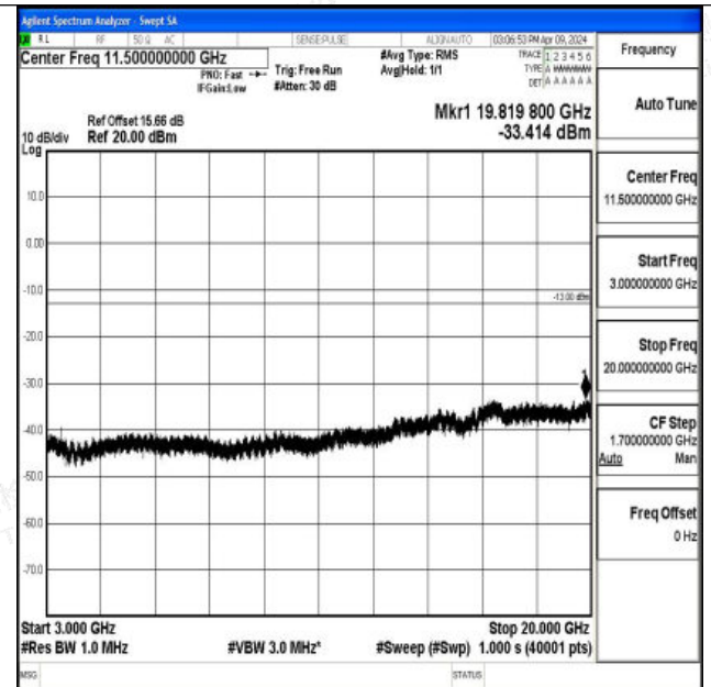
Band66_10MHz_16QAM_132322_1RB#0_3000~20000_30 00~20000
