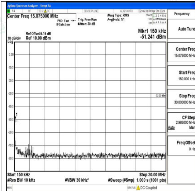
Band66_5MHz_16QAM_132322_1RB#0_0.15~30_0.15~3
