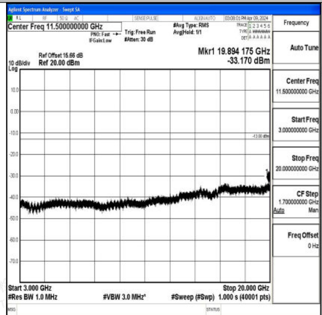
Band66_10MHz_16QAM_132622_1RB#0_3000~20000_30
