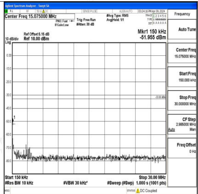
Band66_15MHz_QPSK_132047_1RB#0_0.15~30_0.15~30
