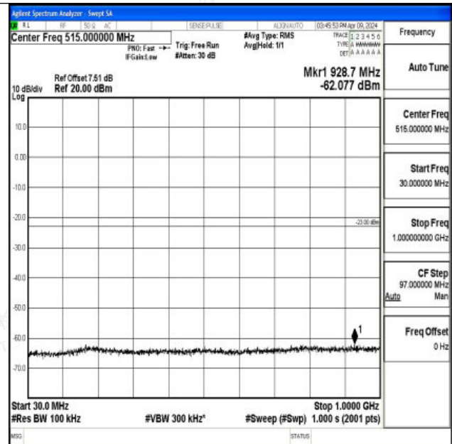
Band66_20MHz_16QAM_132572_1RB#0_30~1000_30~10
