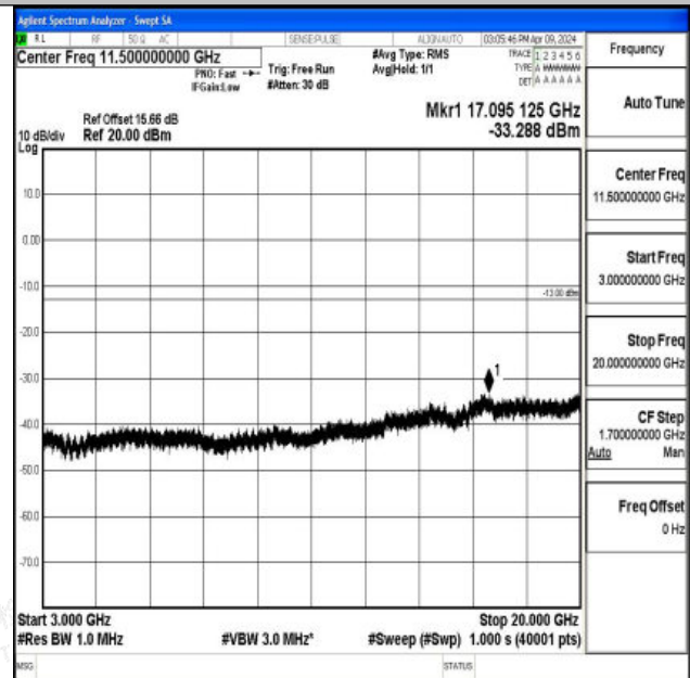
Band66_10MHz_16QAM_132022_1RB#0_3000~20000_30
