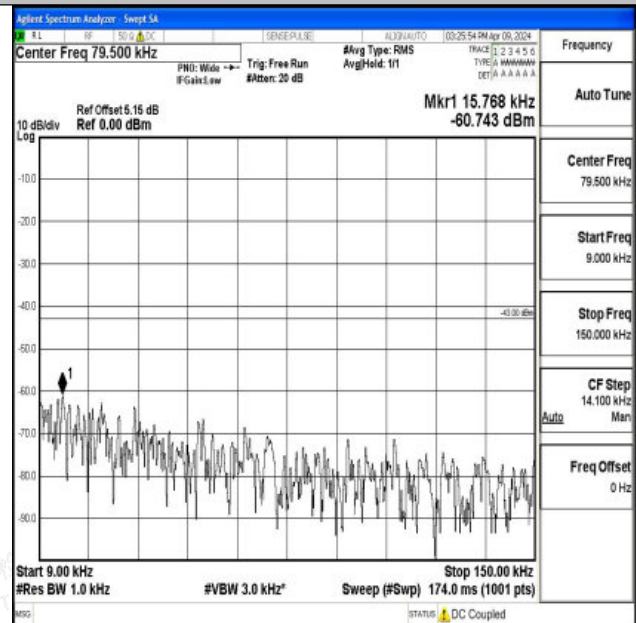
Band66_15MHz_16QAM_132322_1RB#0_0.009~0.15_0.00 9~0.15
