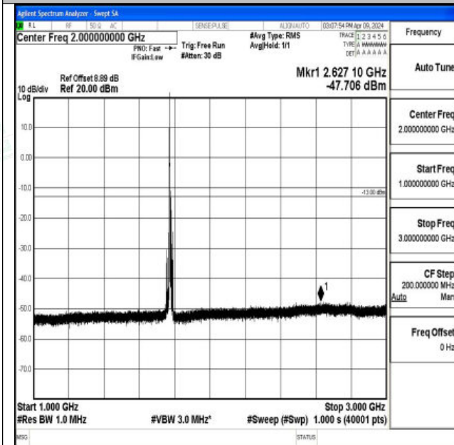
Band66_10MHz_16QAM_132622_1RB#0_1000~3000_10
