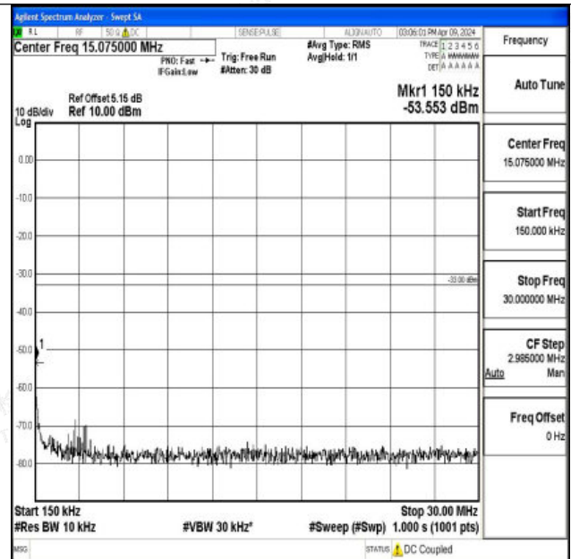
Band66_10MHz_QPSK_132322_1RB#0_0.15~30_0.15~30
