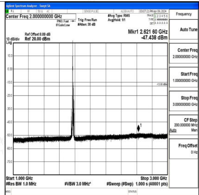
Band66_10MHz_QPSK_132622_1RB#0_1000~3000_1000~3000
