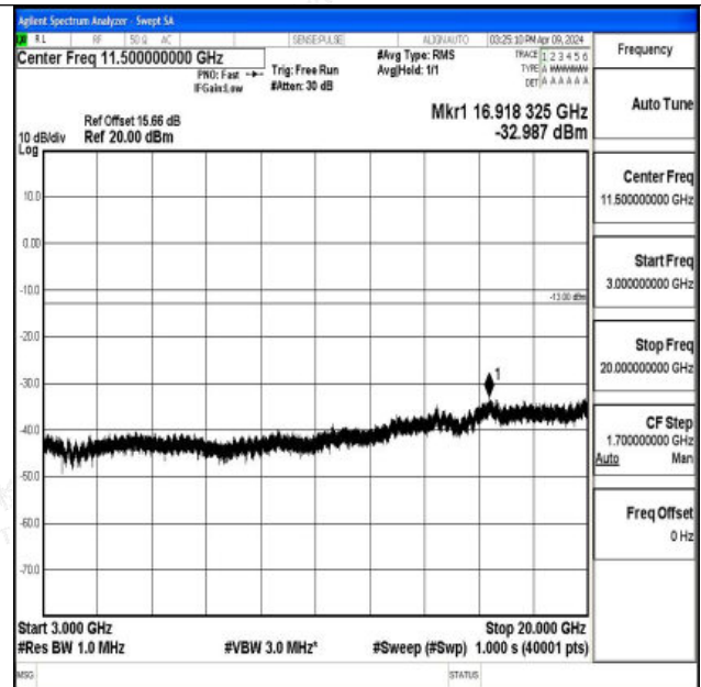
Band66_15MHz_16QAM_132047_1RB#0_3000~20000_30 00~20000
