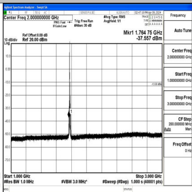
Band66_5MHz_QPSK_132647_1RB#0_1000~3000_1000~3000
