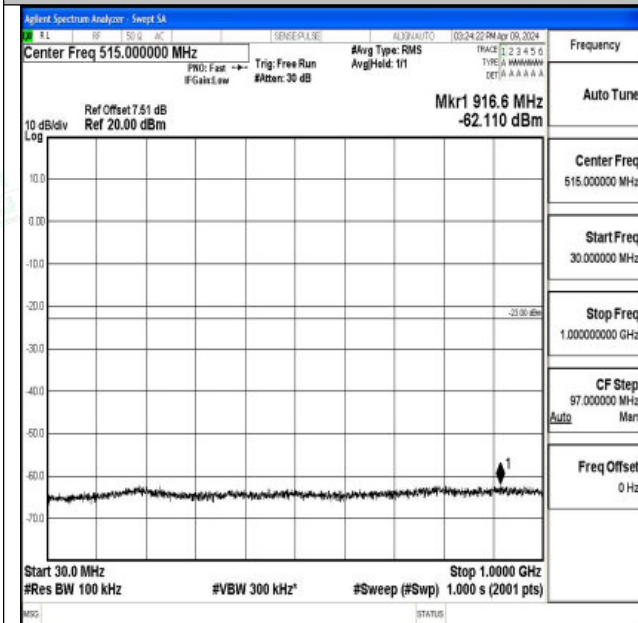
Band66_15MHz_QPSK_132047_1RB#0_30~1000_30~10 00
