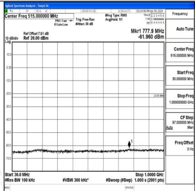
Band66_15MHz_16QAM_132047_1RB#0_30~1000_30~10 00
