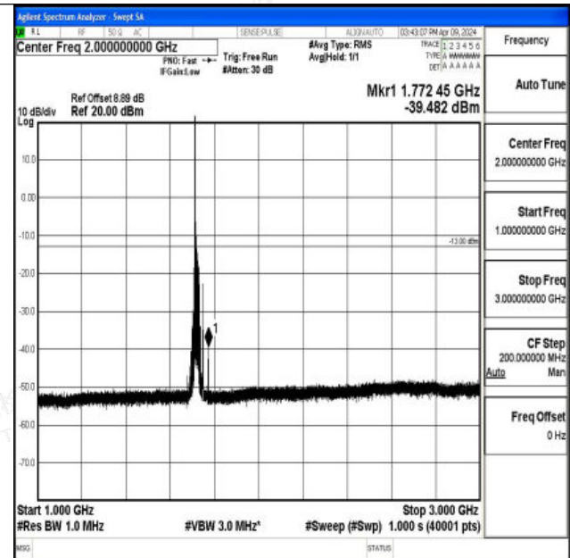
Band66_20MHz_QPSK_132072_1RB#0_1000~3000_1000~3000
