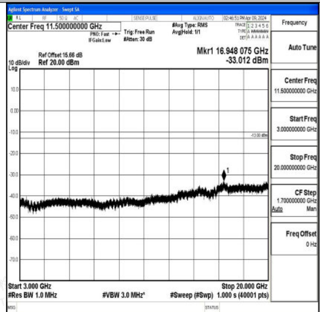
Band66_5MHz_16QAM_132322_1RB#0_3000~20000_3000~20000
