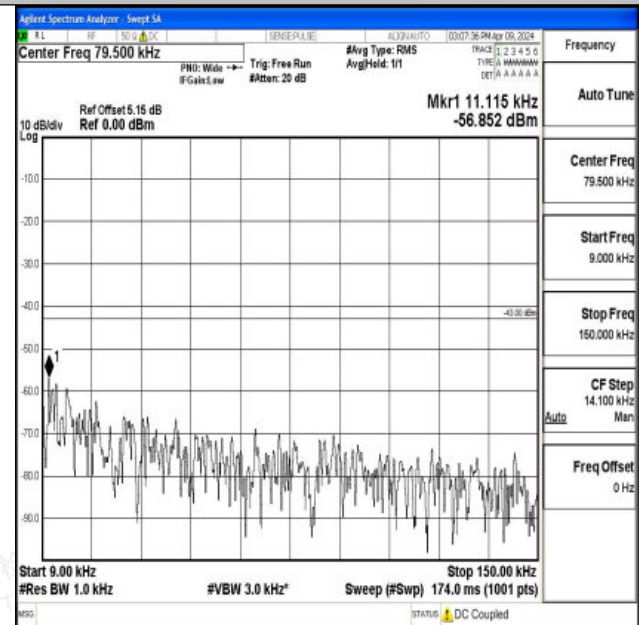
Band66_10MHz_16QAM_132622_1RB#0_0.009~0.15_0.009~0.15
