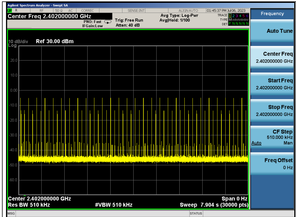
Test_Graph_EDR_HOP_ANT1_NA_3Mbps_2402_Number of Bursts
