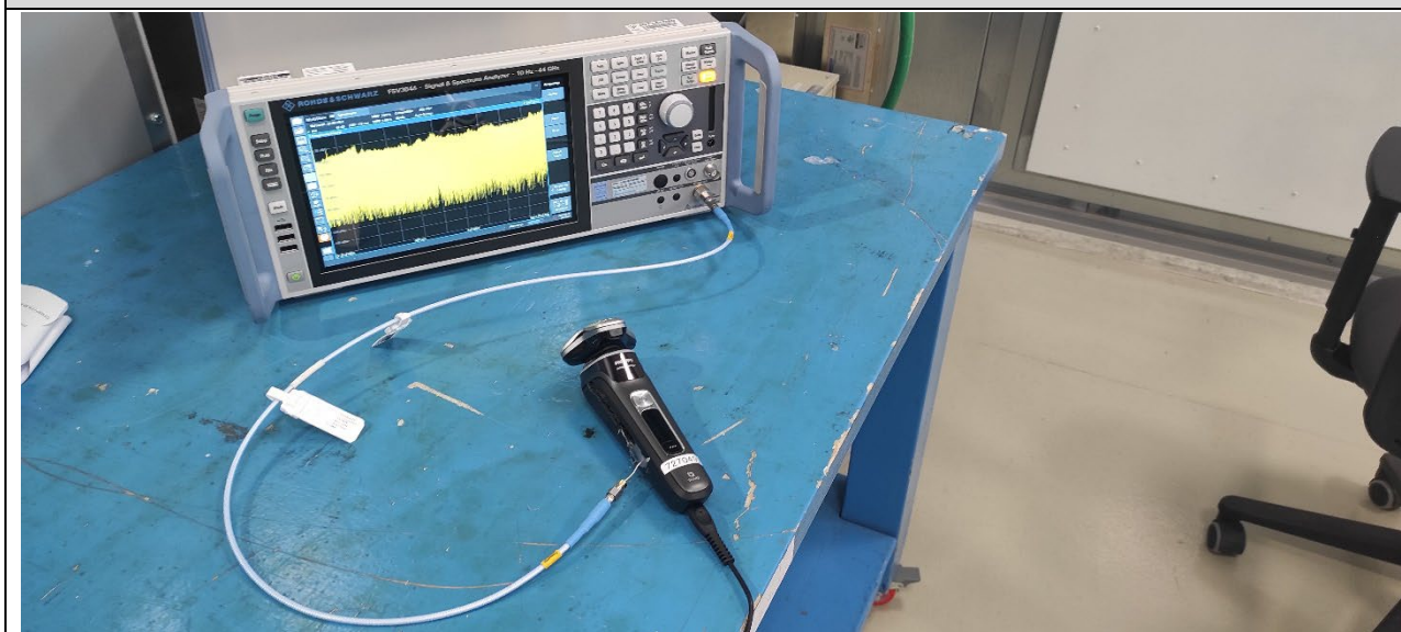
conducted emissions on RF antenna connector
