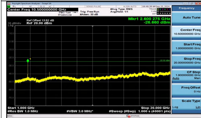
Band38_5MHz_16QAM_38225_1RB#24_1000~20000_1000~20000
