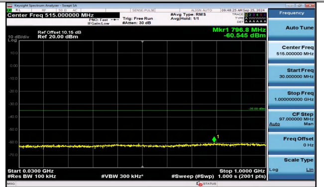
Band38_5MHz_16QAM_38225_1RB#24_30~1000_30~10
