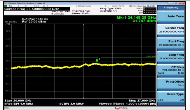
Band38_5MHz_16QAM_38225_1RB#24_20000~27000_20000~27000
