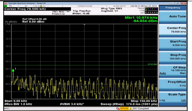
Band38_5MHz_16QAM_38225_1RB#24_0.009~0.15_0.009~0.15
