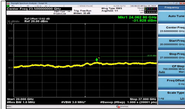
Band38_5MHz_QPSK_38225_1RB#24_20000~27000_20000~27000
