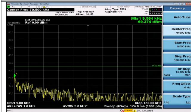
Band38_5MHz_QPSK_38225_25RB#0_0.009~0.15_0.009~0.15
