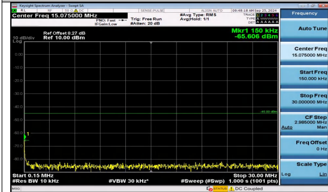
Band38_5MHz_16QAM_38225_1RB#24_0.15~30_0.15~30
